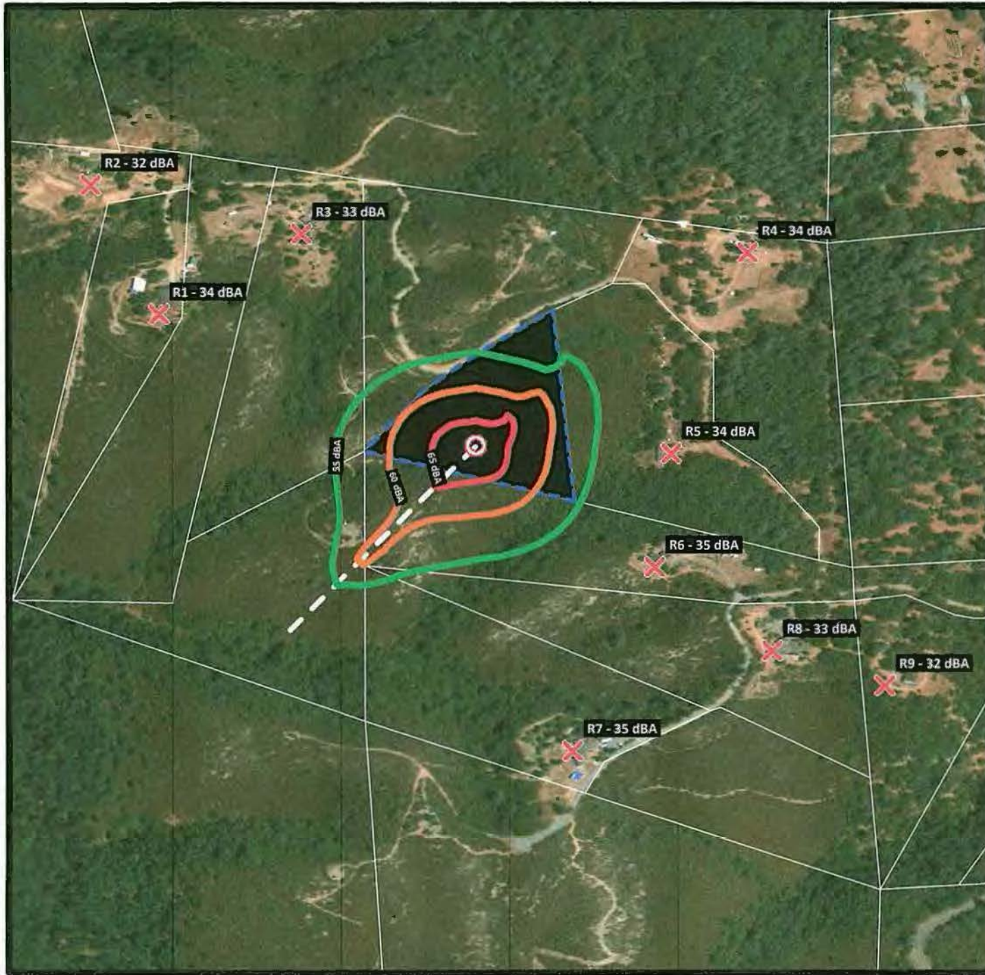
Figure 3: Predicted Aircraft Noise Levels
