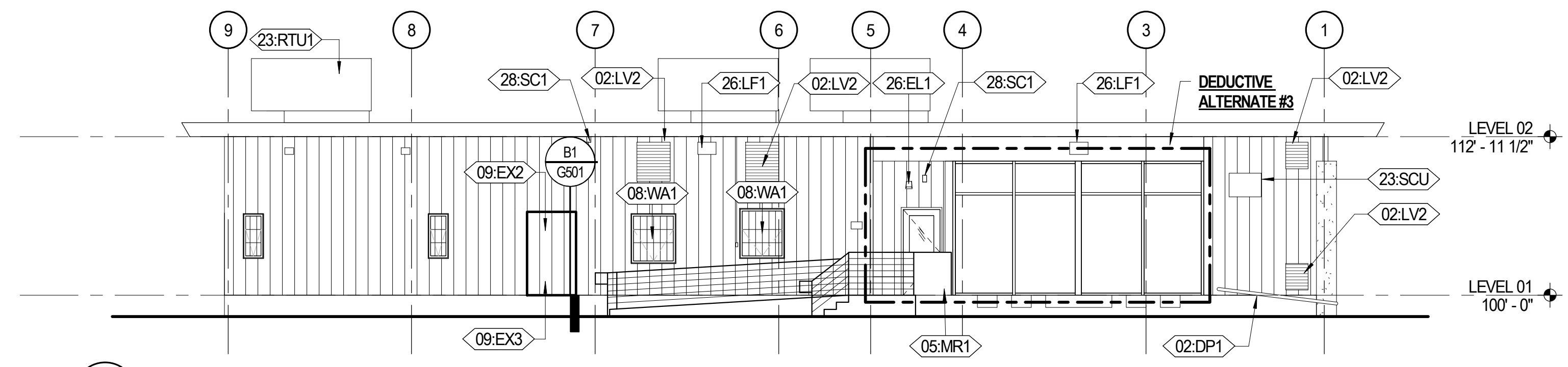
C3 SOUTH ELEVATION A201 1/8" = 1'-0"
