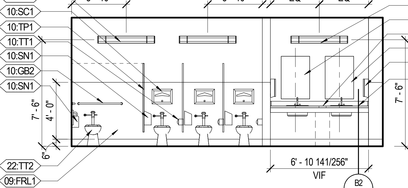
A3 WOMEN'S RESTROOM 114 - NORTH A251 1/4" = 1'-0"
