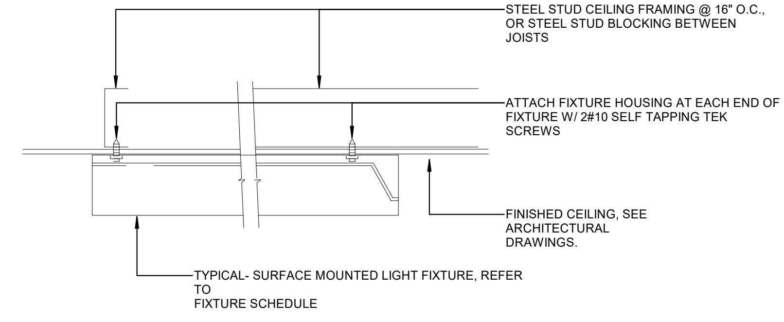
2 Surface Mounted Fixture SCALE: NTS
