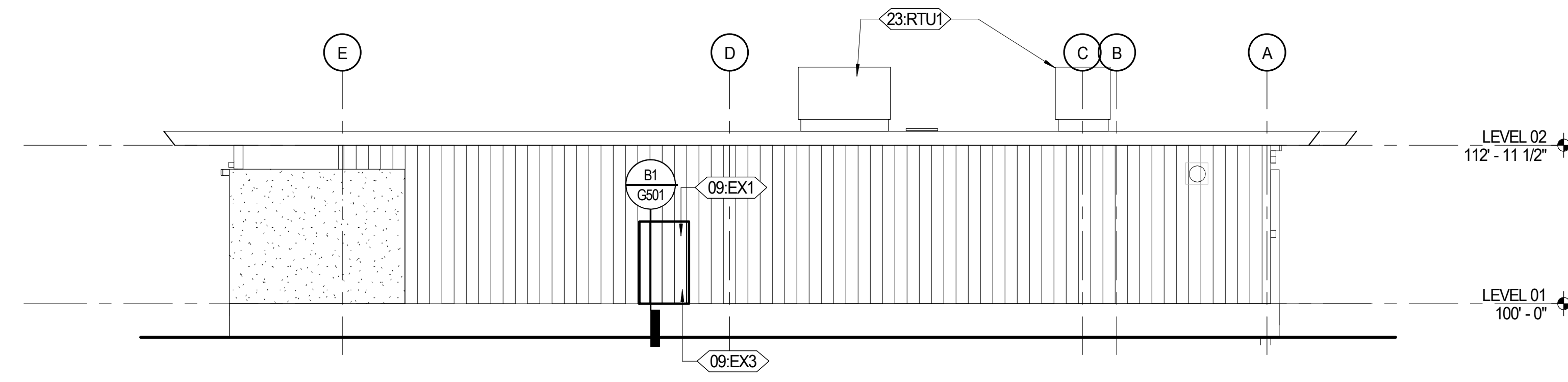
D3 WEST ELEVATION A201 1/8" = 1'-0"
