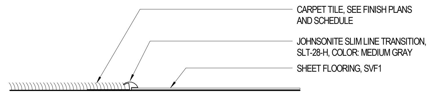
2 CARPET TILE TO RESILIENT FLOORING TRANSITION AI602 1 1/2" = 1'-0"
