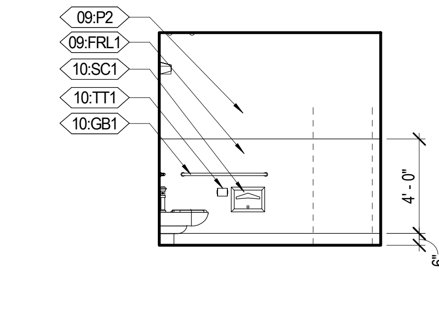
B3 MEN'S RESTROOM 112 - ACC. STALL - WEST A251 1/4" = 1'-0"
