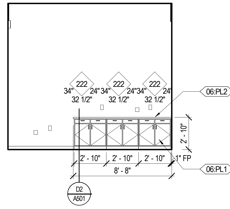
E5 WORK/MAIL 122 - NORTH A252 1/4" = 1'-0"
