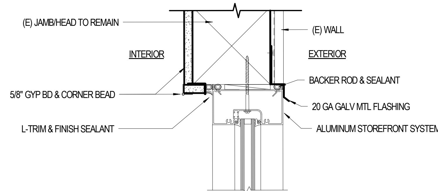
A4 STOREFRONT HEAD/JAMB DEDUCTIVE ALTERNATE #3 A602 3" = 1'-0"
