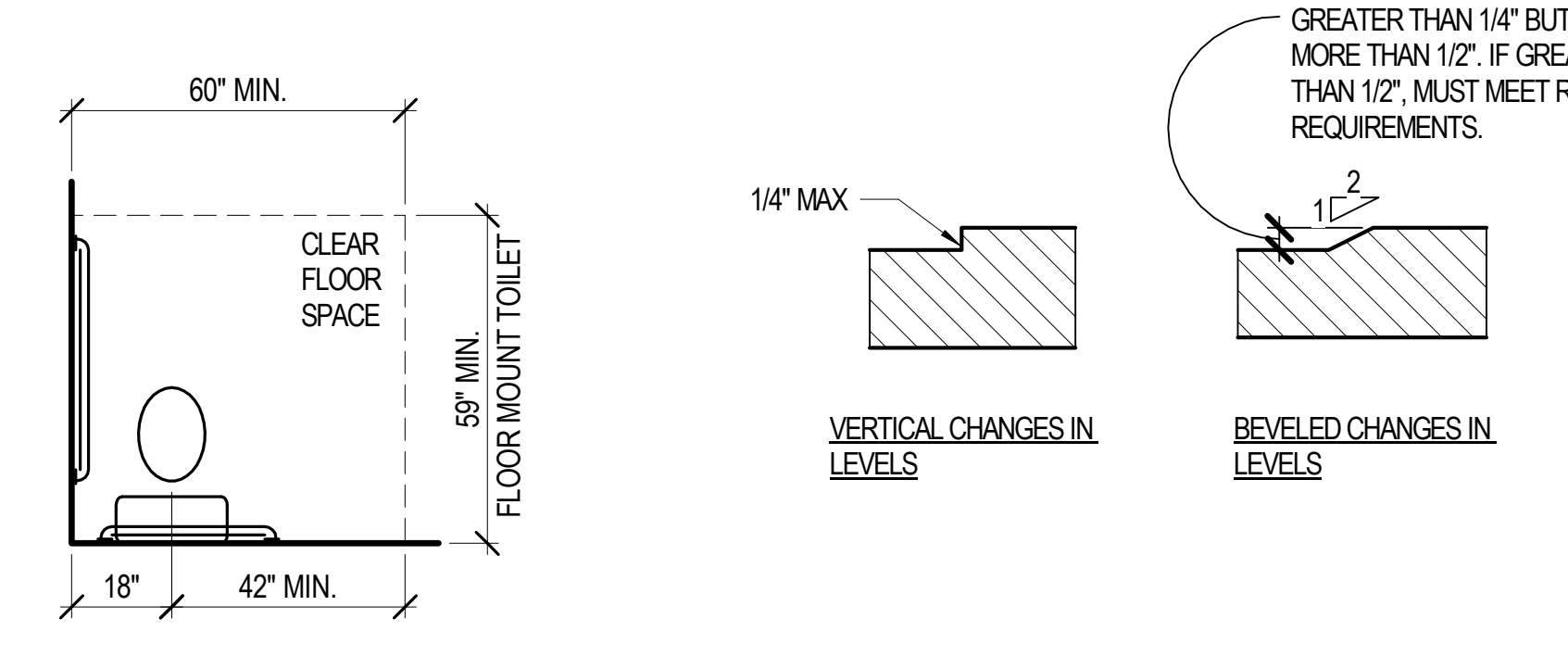
B5 CHANGE IN LEVELS G701 6" = 1'-0"
