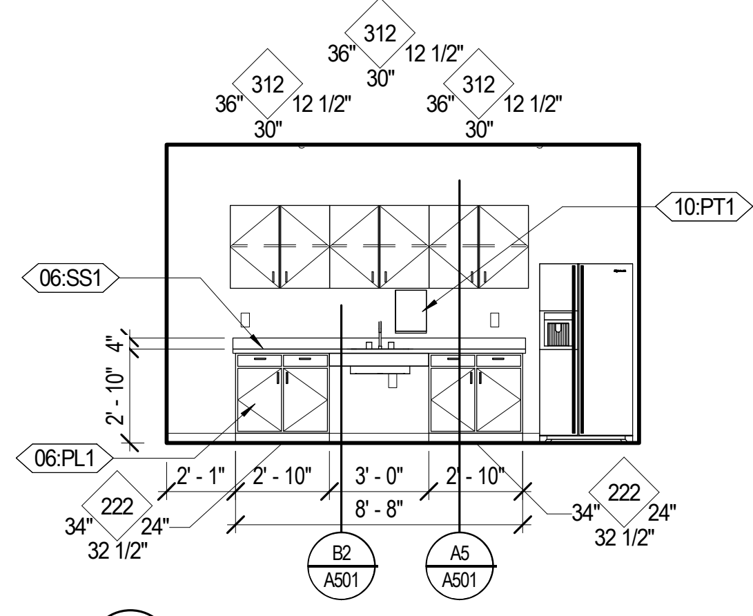
E4 BREAK ROOM 117 - WEST A252 1/4" = 1'-0"
