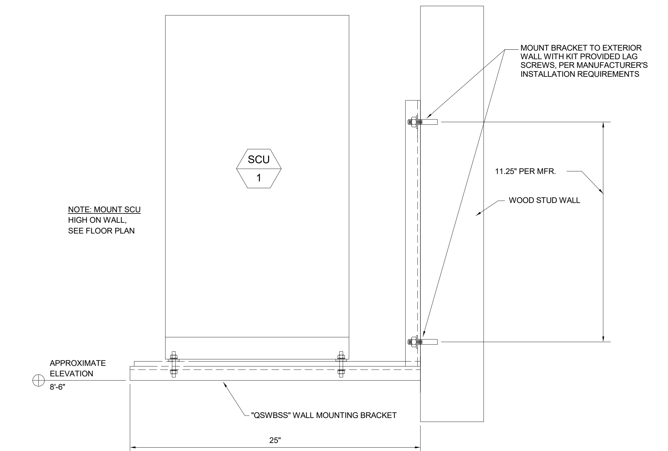
SCU MOUNTING AT EXTERIOR WALL SCALE: NONE
