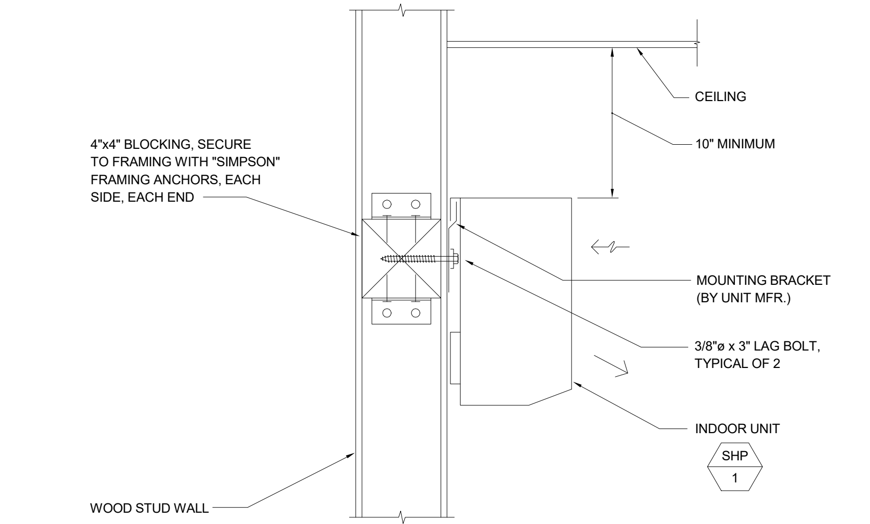
SPLIT SYSTEM INDOOR MOUNTING SCALE: NONE
