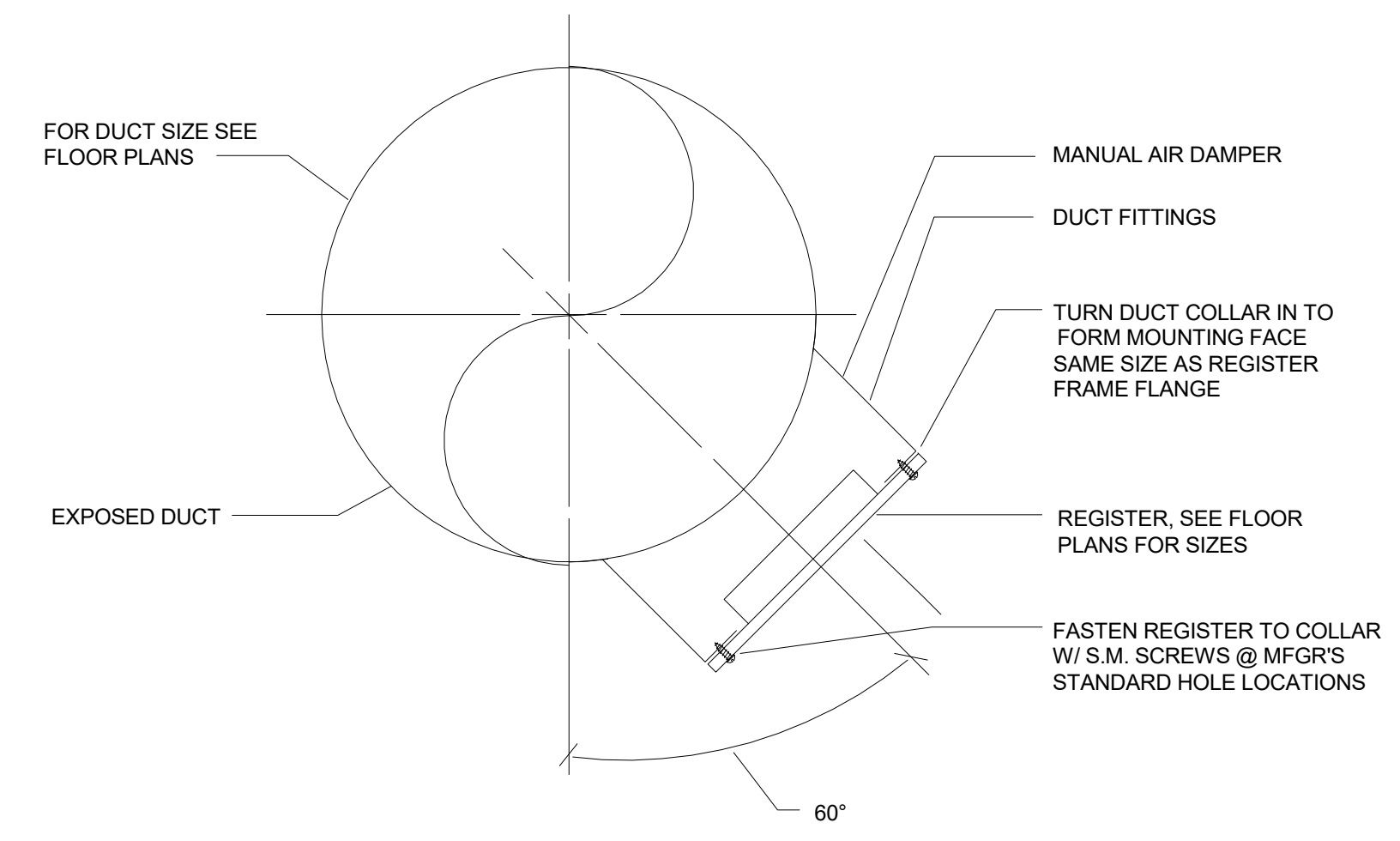
DIFFUSER/GRILLE ON EXPOSED DUCT SCALE: NONE
