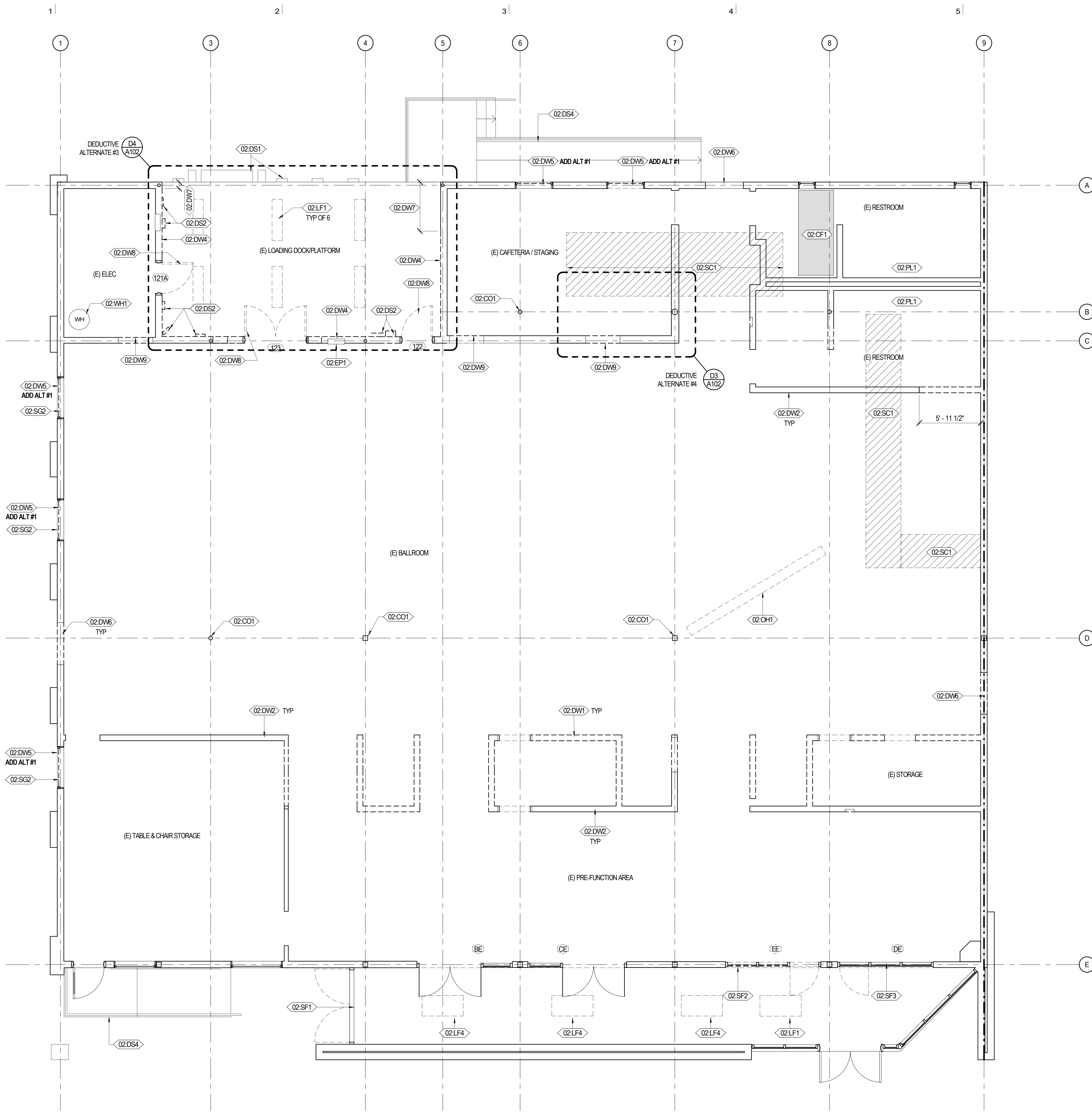
A1 LEVEL 01 - DEMOLITION PLAN AD101 1/4" = 1'-0"
