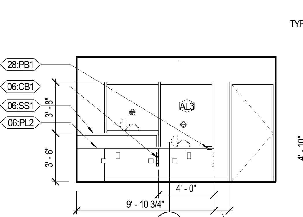
E3 RECEPTION 102 - EAST A251 1/4" = 1'-0"
