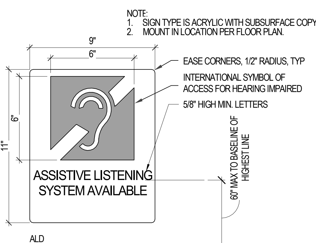
A ASSISTED LISTENING SIGN G701 3" = 1'-0"
