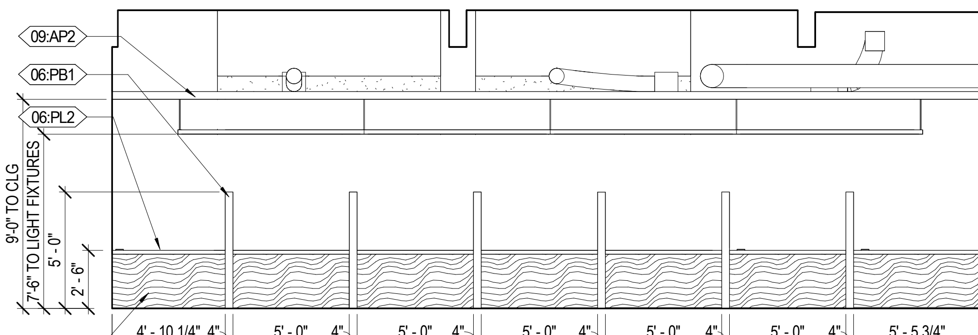
D3 STAFF WORK BOOTHS 105 - NORTH A251 1/4" = 1'-0"
