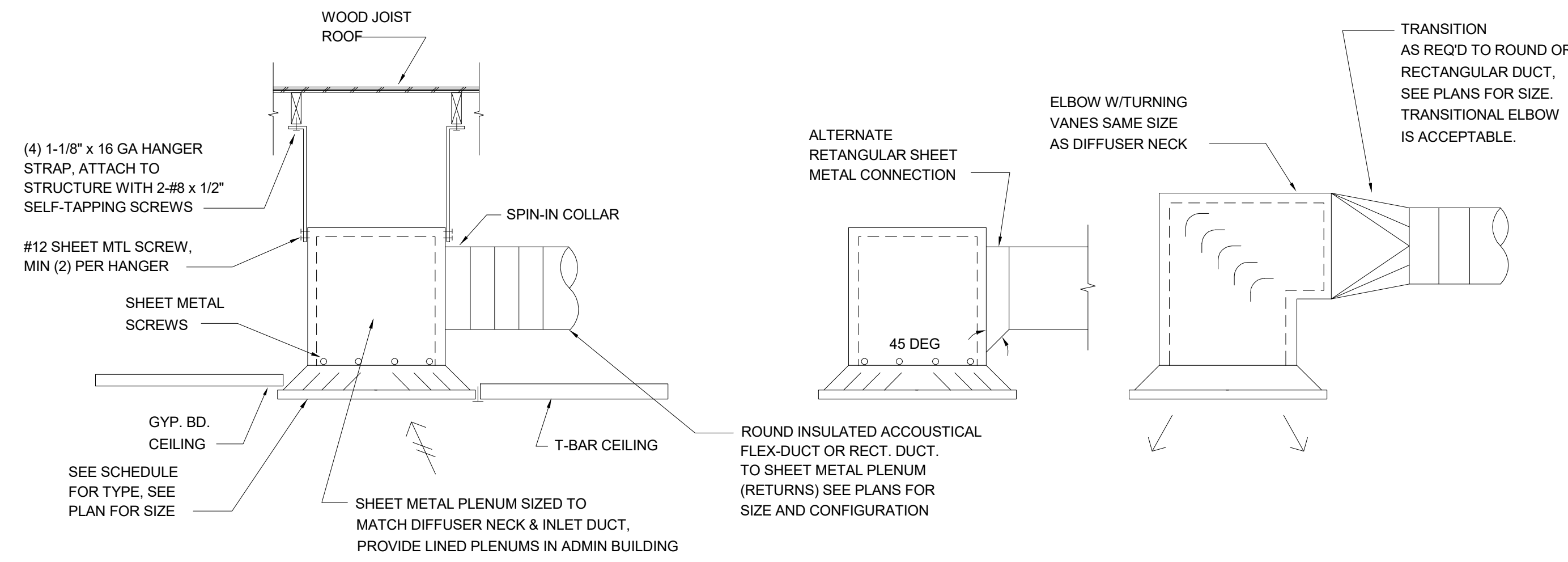
SUPPLY, RETURN, & EXHAUST TERMINAL SCALE: NONE
