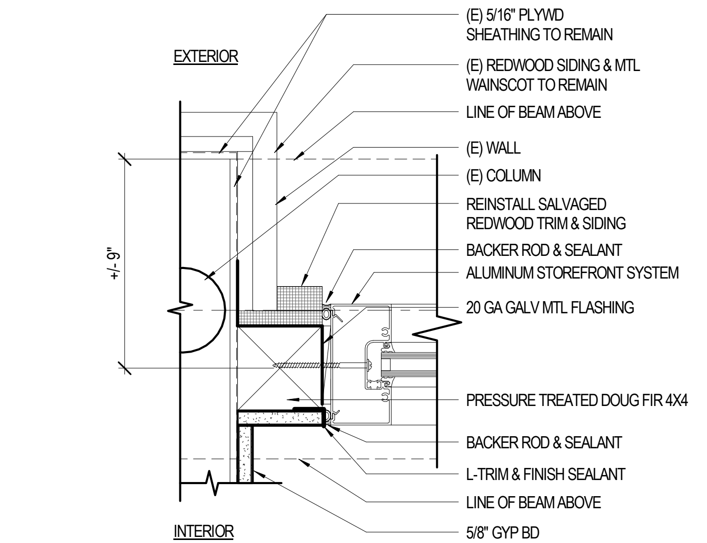
C5 EXTERIOR STOREFRONT JAMB AT EXISTING WALL A602 3" = 1'-0"
