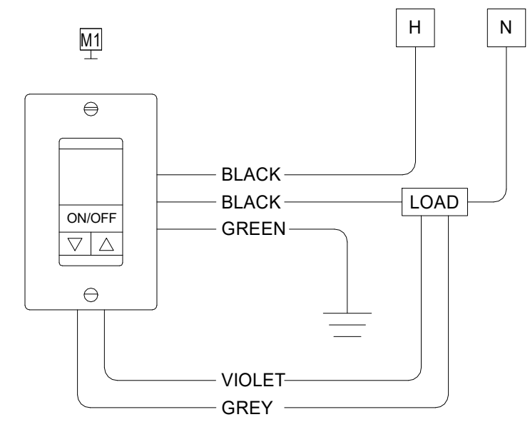
SINGLE RELAY WALL MOUNTED DUAL-TECHNOLOGY OCCUPANCY SENSOR No neutral wiring required at device. Typical at any room with wallbox occupancy sensor U.O.N. Set time delay to 5 min, sensitivity to max. Primary load (switchleg 'a') is automatic on, automatic off Provide 0-10V control wiring to all dimmable fixtures, not shown on plans.
