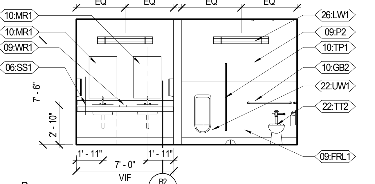
B1 MEN'S RESTROOM 112 - SOUTH A251 1/4" = 1'-0"
