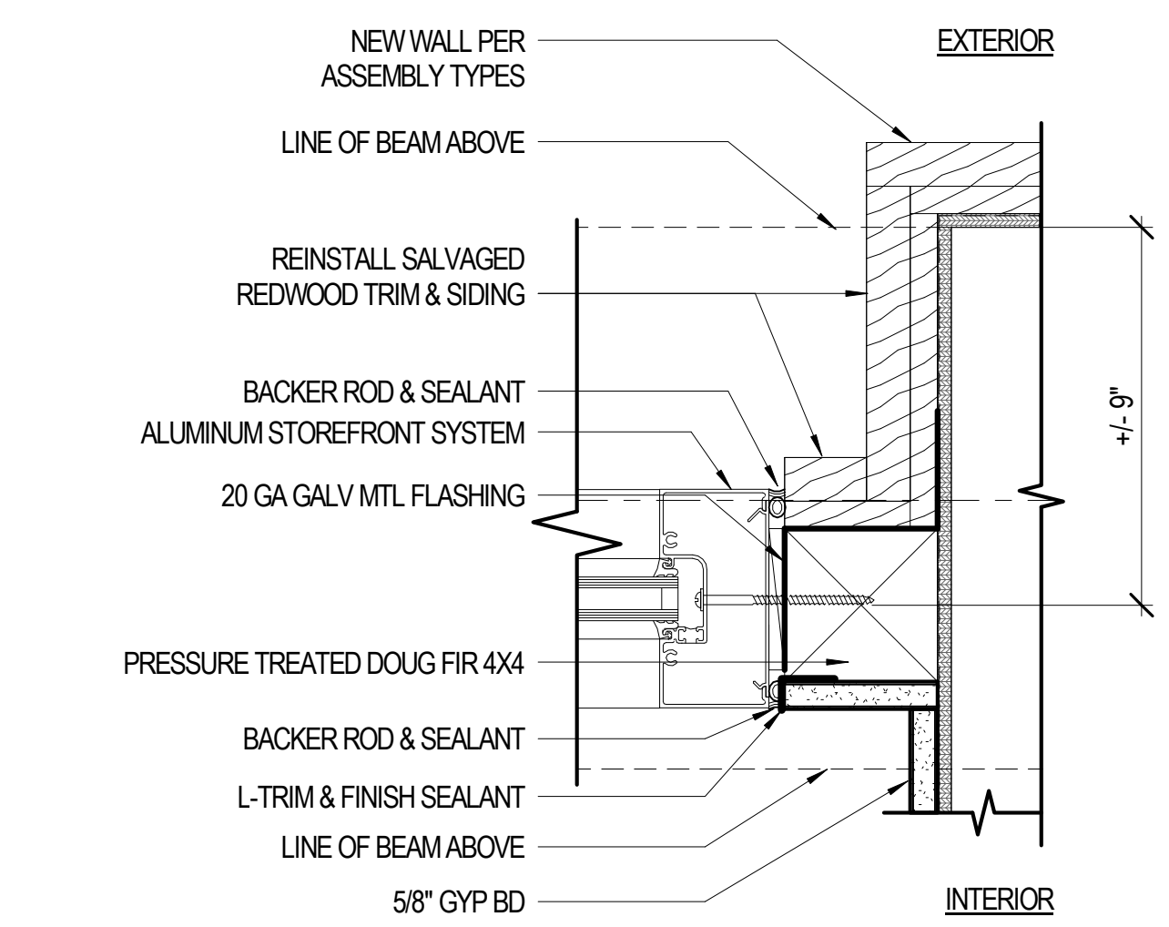
B5 EXTERIOR STOREFRONT JAMB AT NEW WALL A602 3" = 1'-0"
