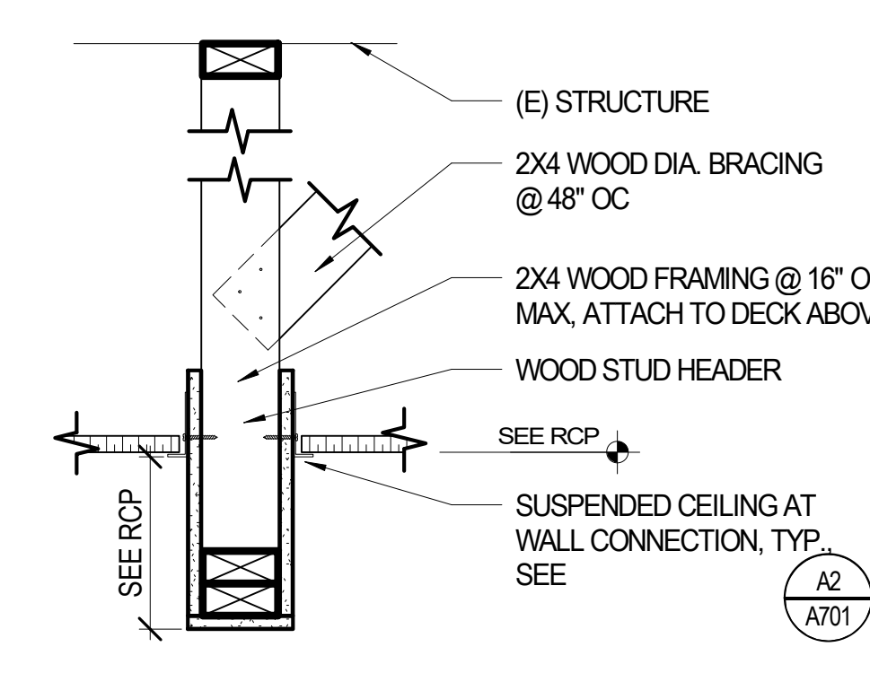
B1 SOFFIT HEADER DETAIL A701 1 1/2" = 1'-0"
