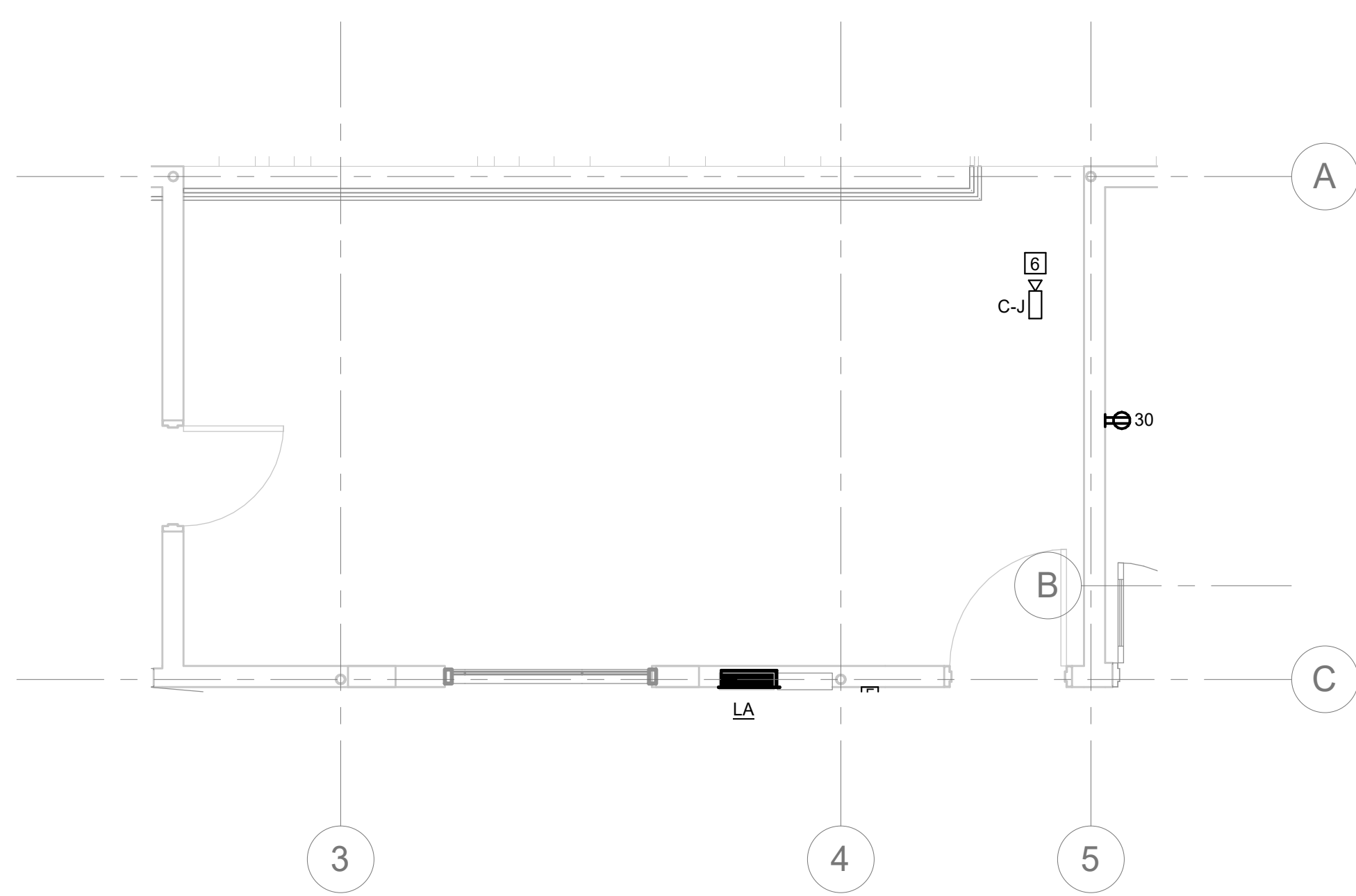
2 POWER & SIGNAL PLAN - ALT#3 SCALE: 1/4" = 1'-0"
