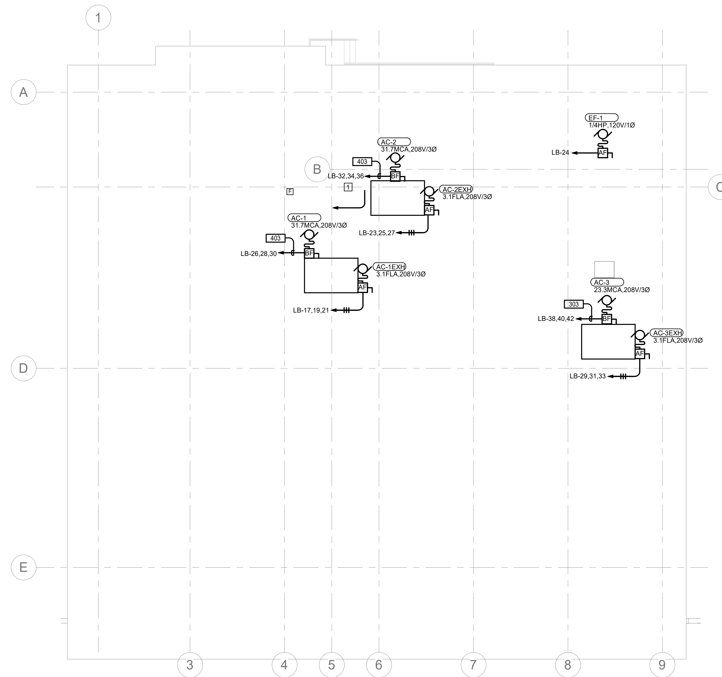
1 POWER & SIGNAL PLAN - ROOF SCALE: 1/8" = 1'-0"
