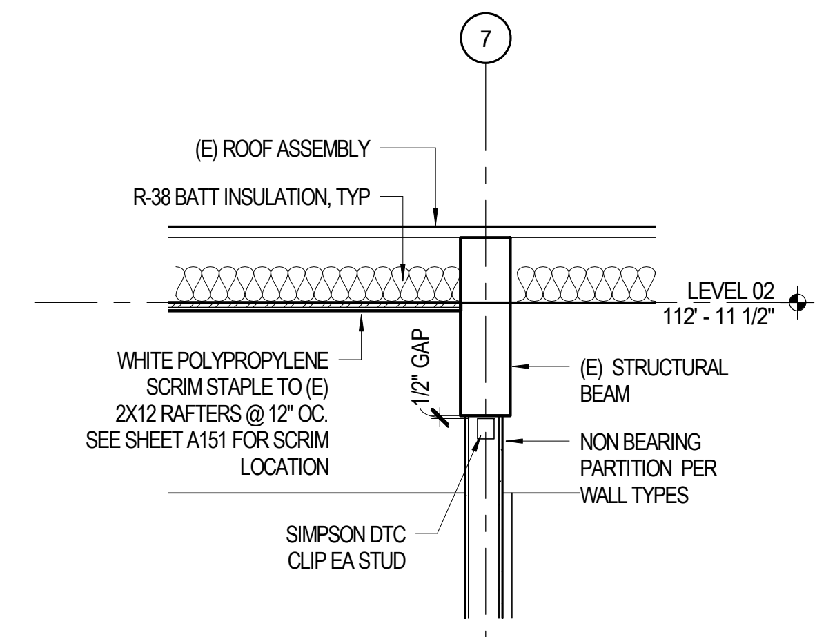
2 (N) WALL TO (E) BEAM G501 1/2" = 1'-0"
