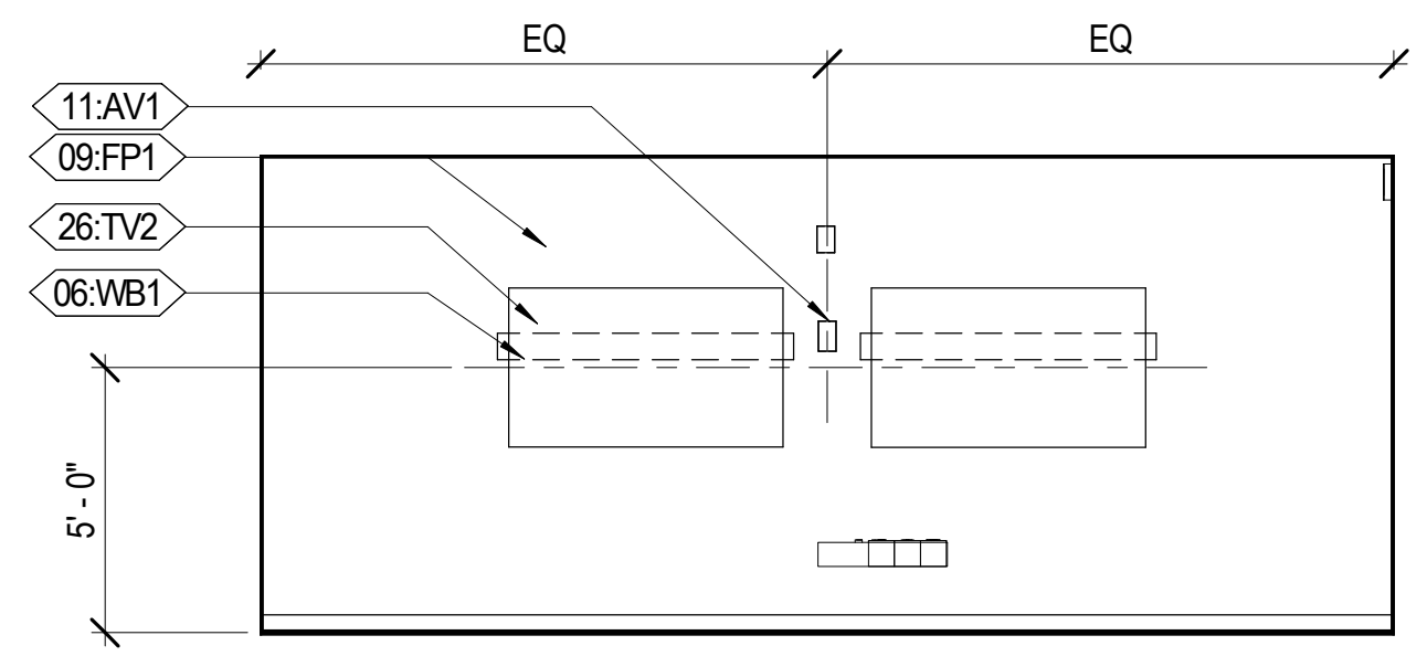
E1 UNISEX STAFF RESTROOM 116 - SOUTH A252 1/4" = 1'-0"
