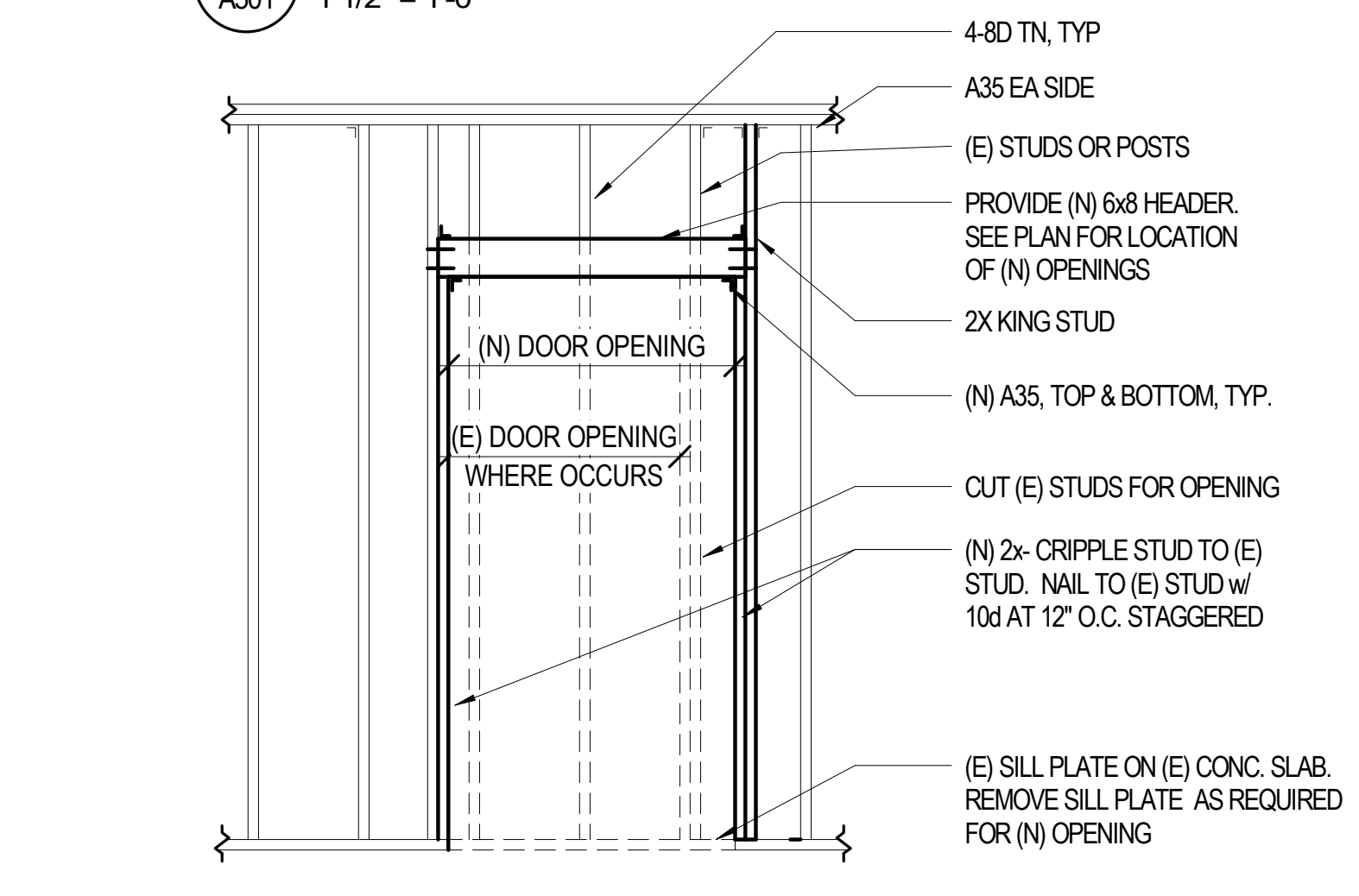
C1 TYPICAL NEW FRAMED WALL OPENING A501 1/2" = 1'-0"
