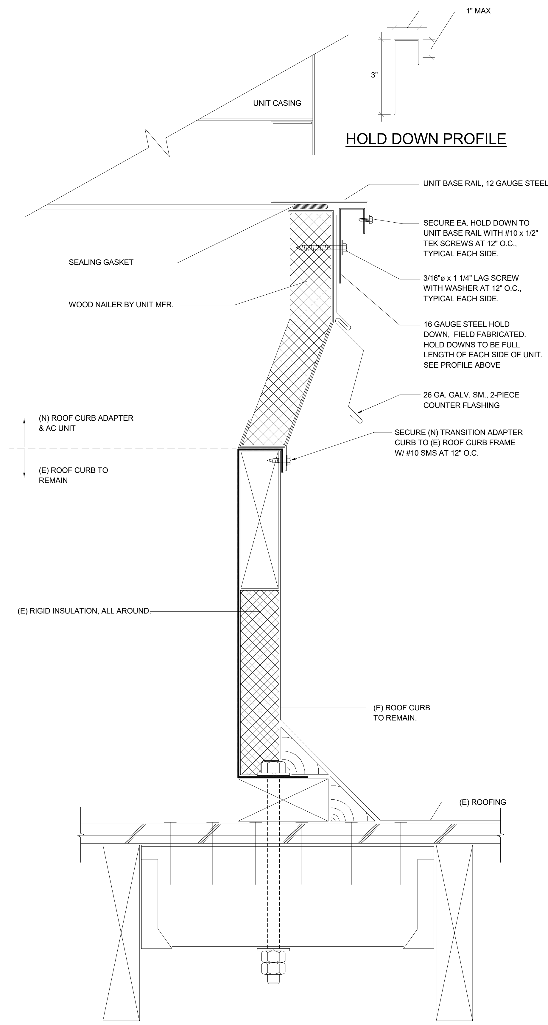
AC UNIT MOUNTING SCALE: NONE
