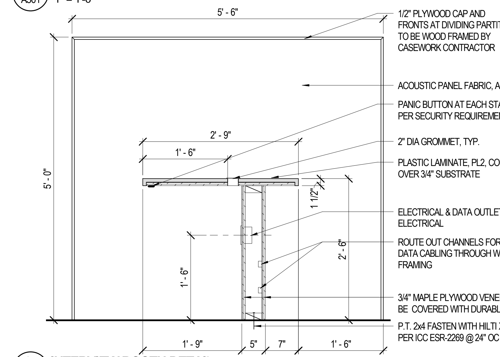
C3 INTERVIEW BOOTH DETAIL A501 1" = 1'-0"
