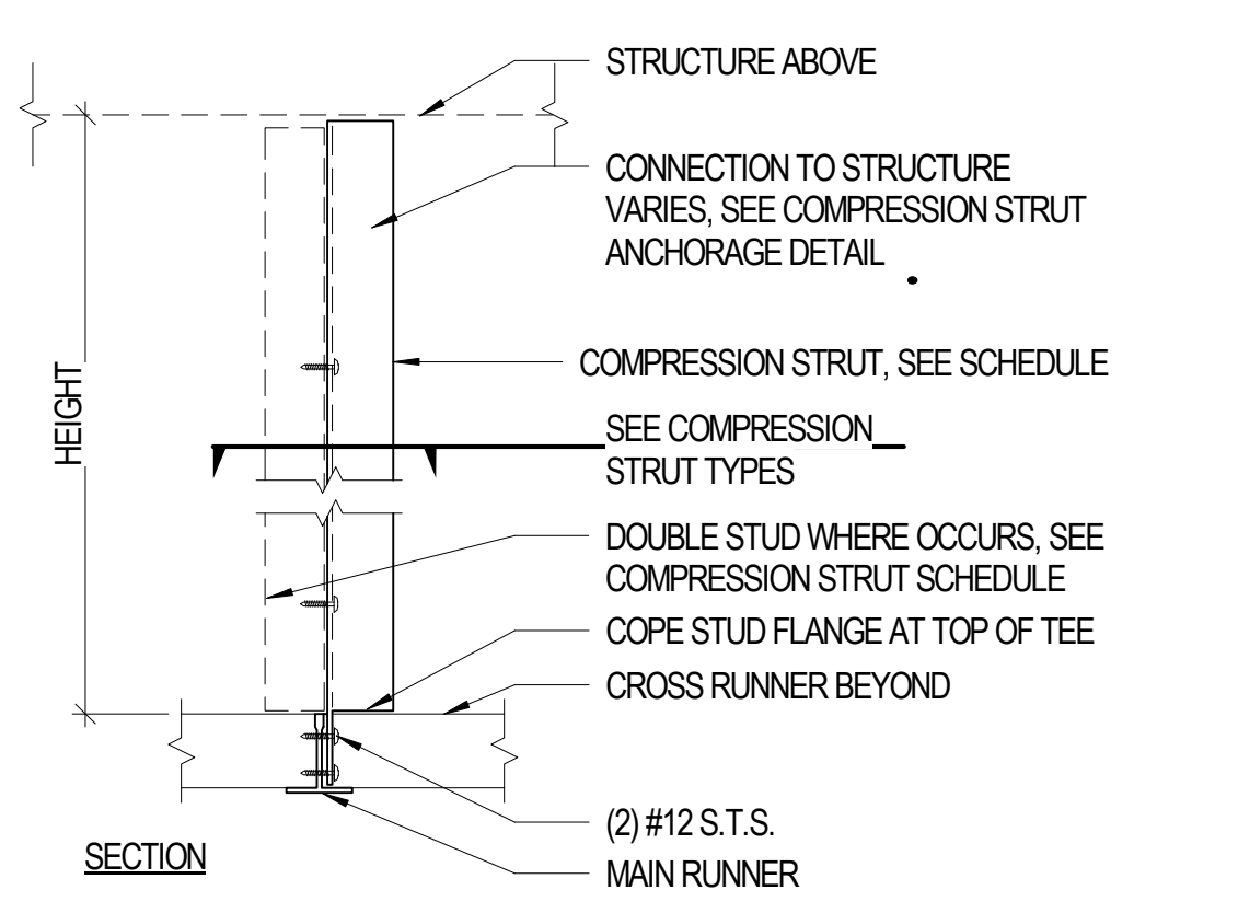
C1 COMPRESSION STRUT A701 3" = 1'-0"
