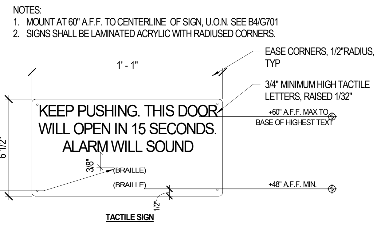
E3 SIGN - DELAYED EGRESS G701 3" = 1'-0"
