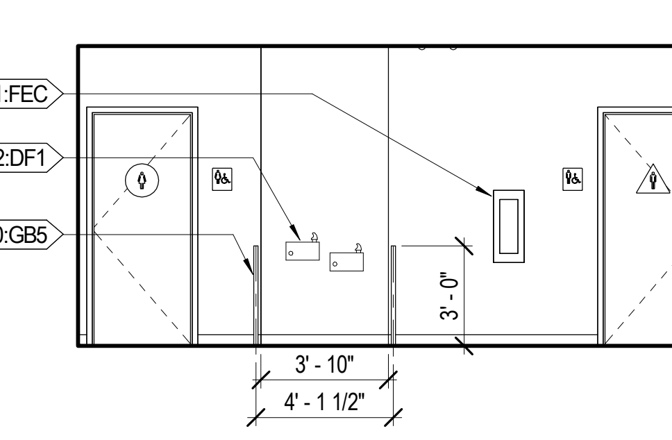
B6 CORRIDOR 113 - WEST A251 1/4" = 1'-0"
