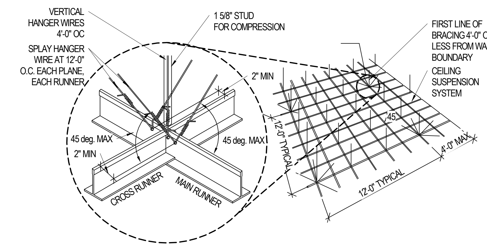
D4 A701 - TYP. SEISMIC BRACING DETAIL A701 3" = 1'-0"
