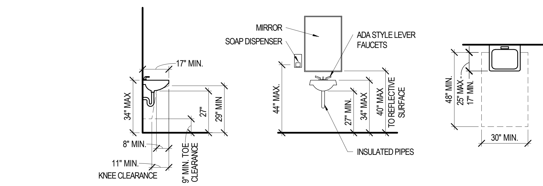
A1 URINAL MOUNTING HEIGHT G701 3/8" = 1'-0"
