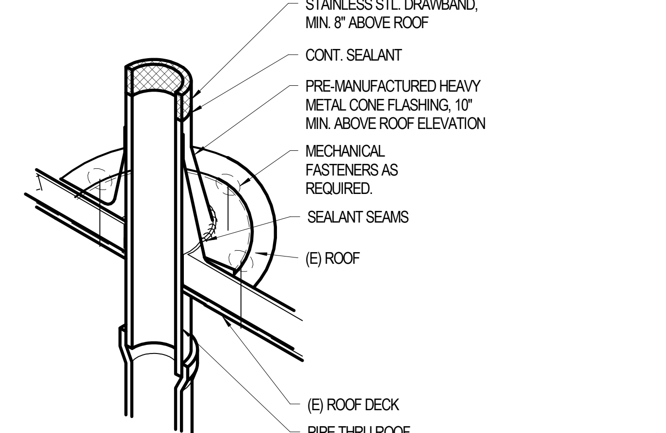
C5 TYPICAL PIPE FLASHING DETAIL A701 3" = 1'-0"
