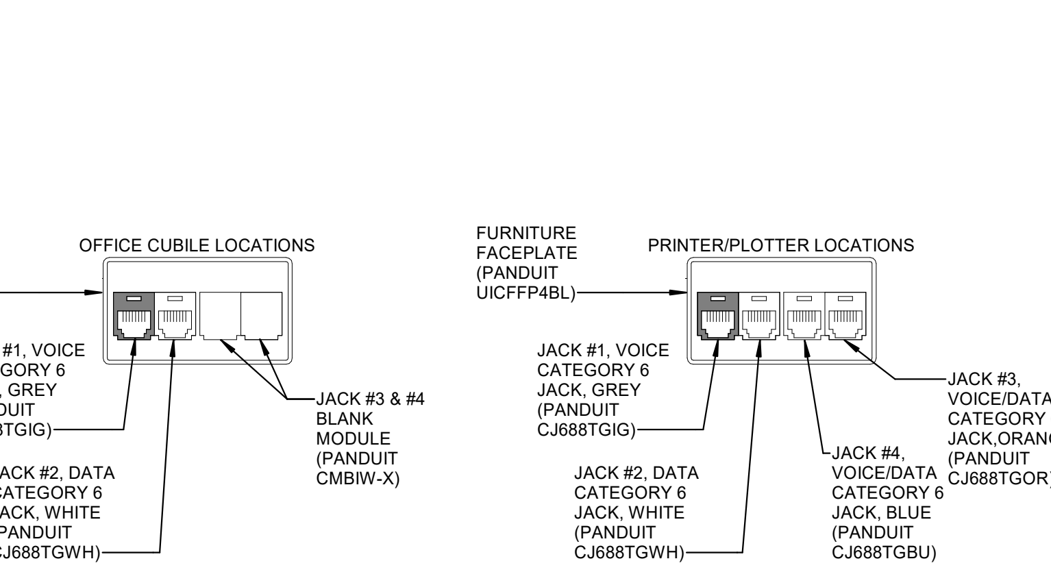
7 Typical Furniture Cable Termination Plate SCALE: NTS
