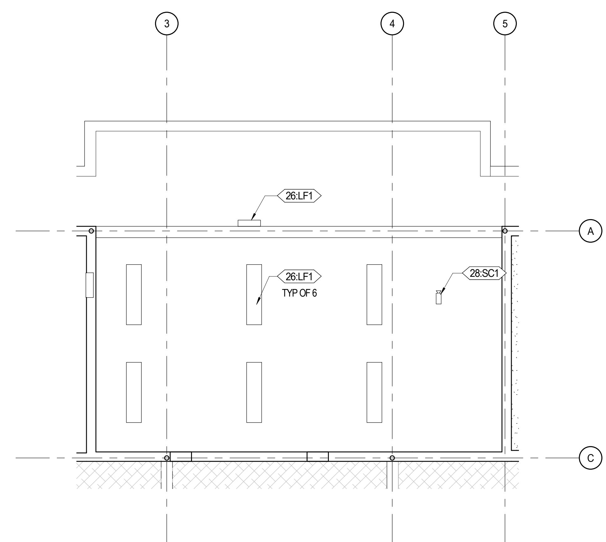
A4 REFLECTED CEILING PLAN DEDUCTIVE ALTERNATE 3 A102 1/4" = 1'-0"
