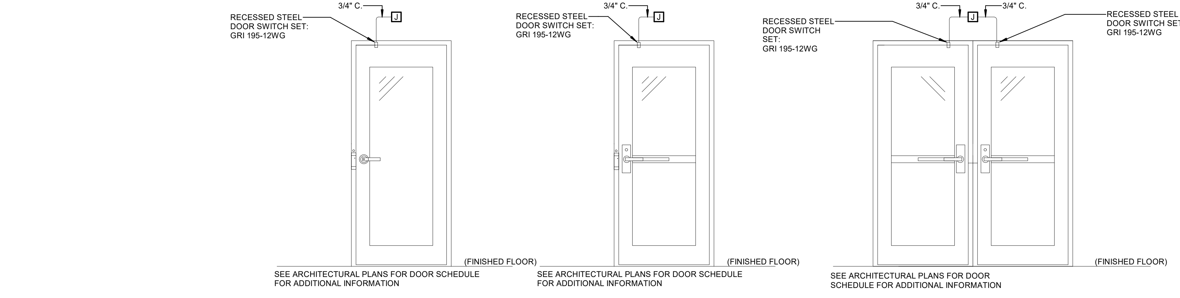
5 Typical Door Elevations-Access and Intrusions SCALE: NTS
