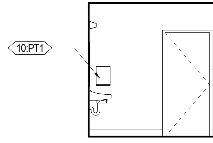
E3 UNISEX STAFF RESTROOM 116 - NORTH A252 1/4" = 1'-0"
