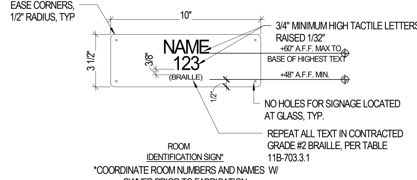
D2 SIGN ROOM IDENTIFICATION G701 3" = 1'-0"
