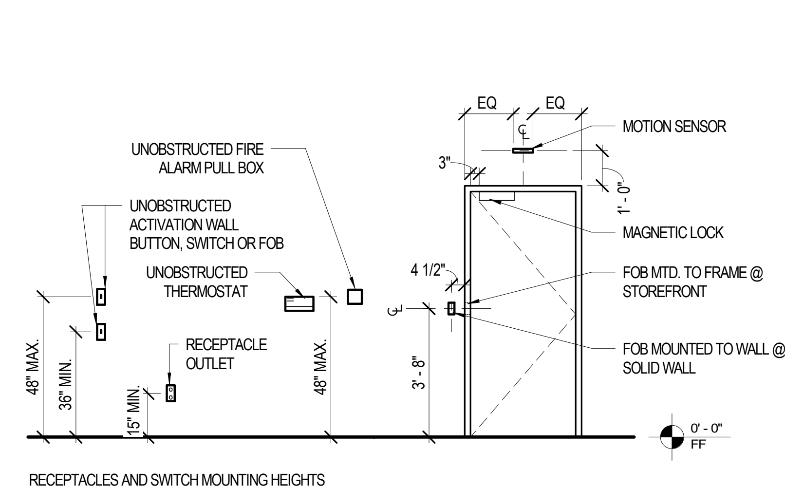
B3 MISC. MOUNTING HEIGHTS G701 3/8" = 1'-0"
