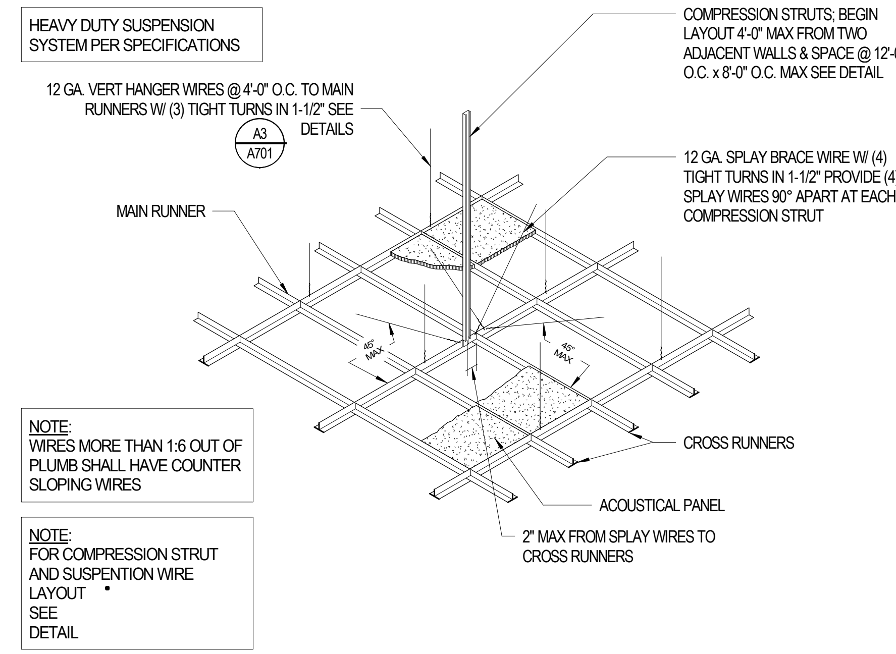
SUSPENDED CEILING GRID SCALE: 1/4" = 1'-0"
