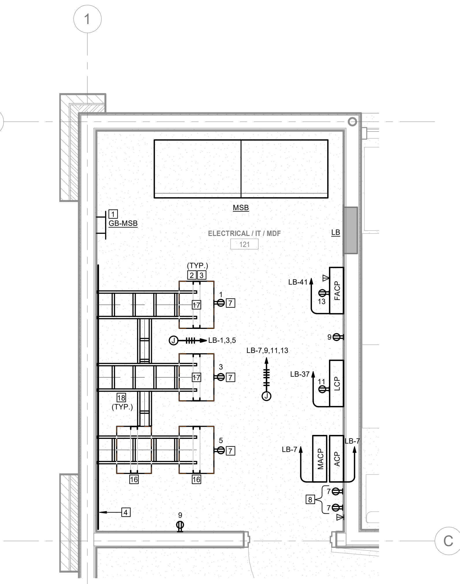
4 ELECTRICAL/IT/MDF ROOM ENLARGEMENT SCALE: 1/2" = 1'-0"
