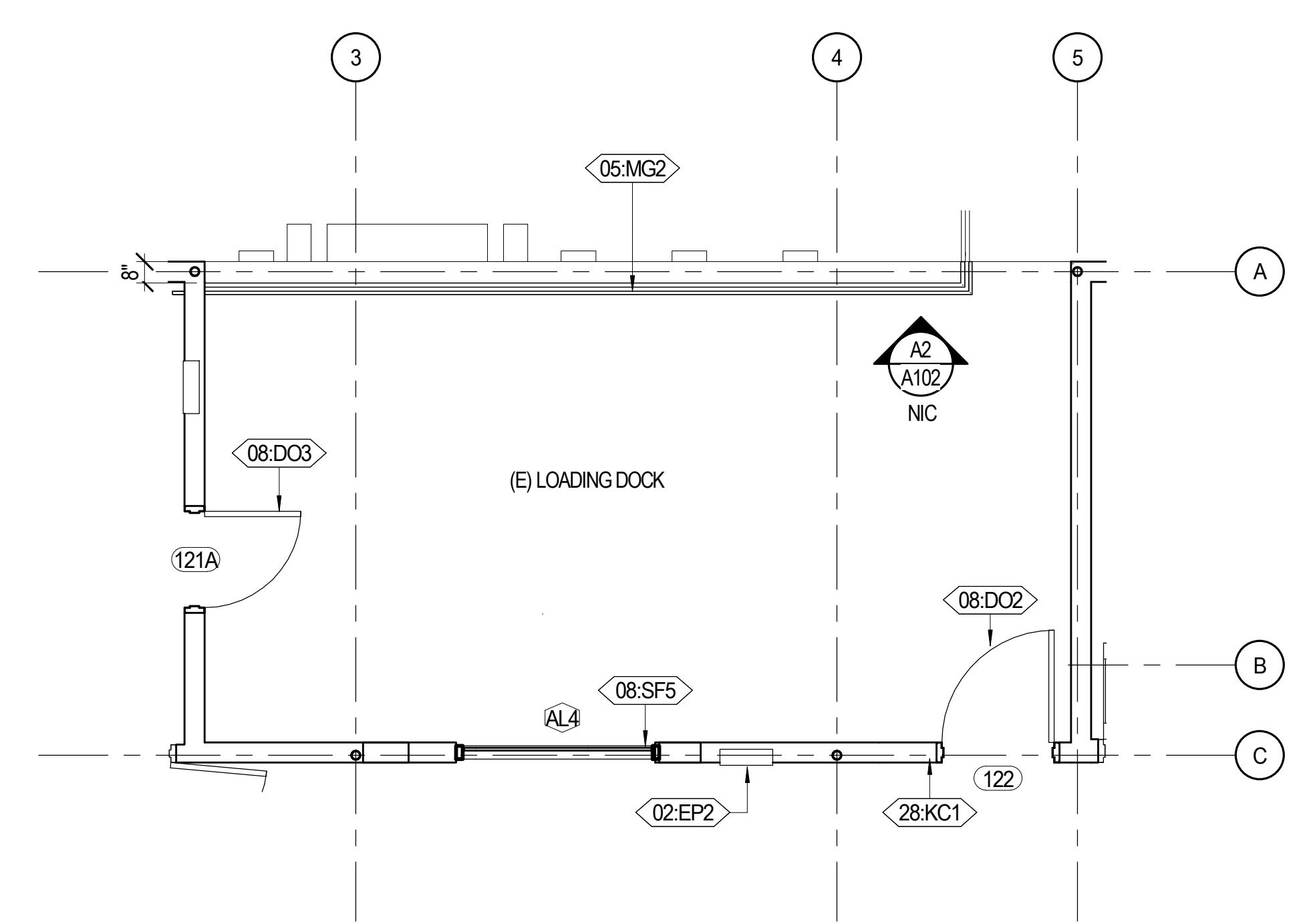
C4 FLOOR PLAN DEDUCTIVE ALTERNATE #3 A102 1/4" = 1'-0"
