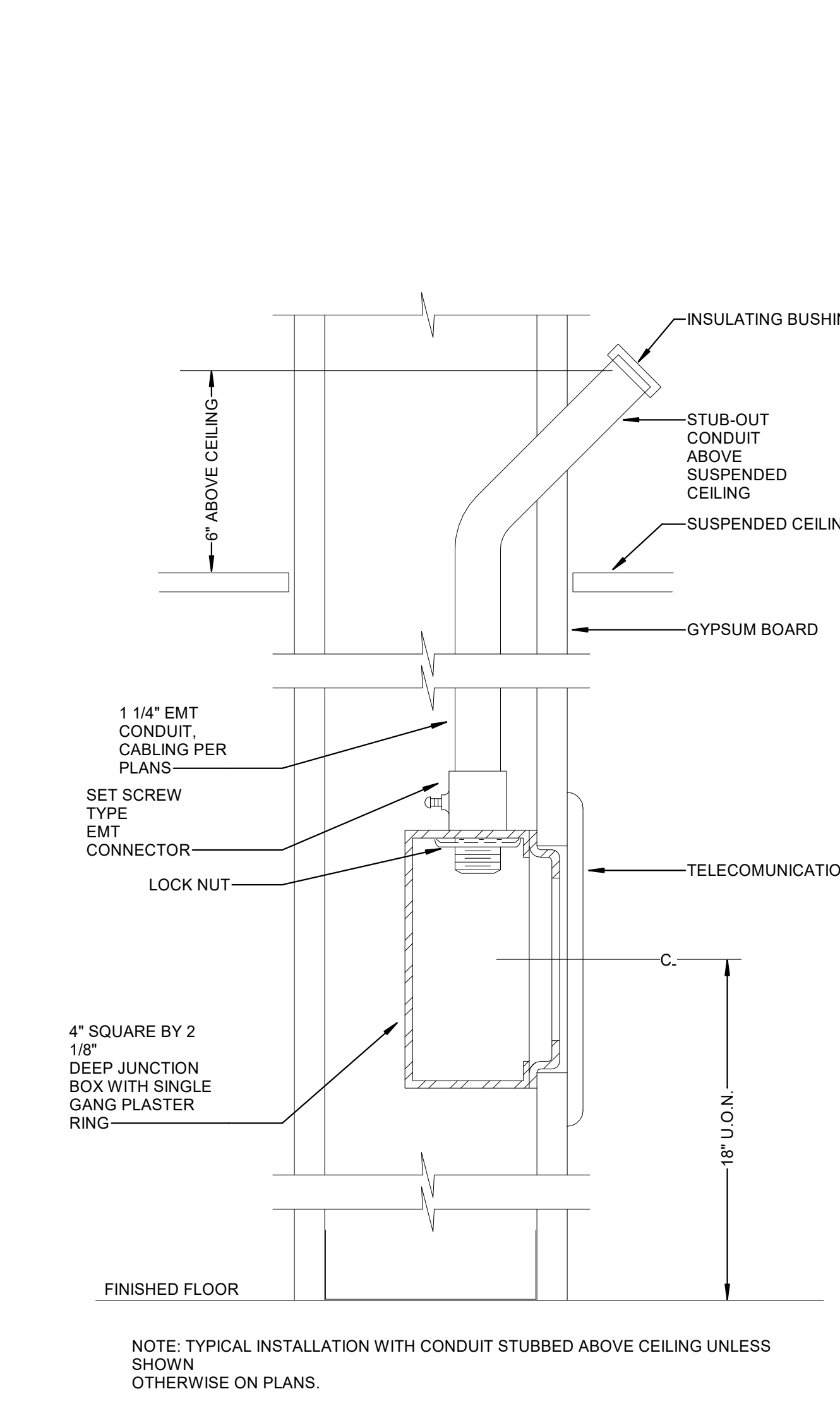
3 Low Voltage Device - Fire Rated Or Insulated Wall Locations SCALE: NTS
