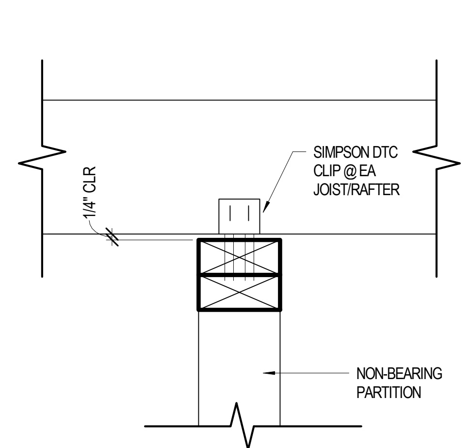
8 NON-BEARING WALL TO JOISTS/RAFTERS G501 3" = 1'-0"
