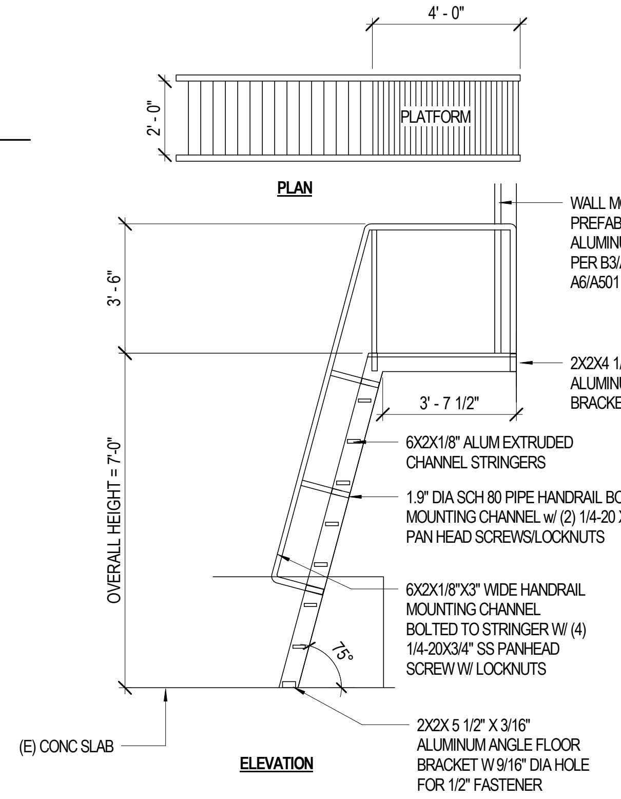
5 SHIPS LADDER WITH LANDING PLATFORM G501 3/8" = 1'-0"
