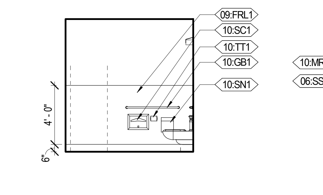
A5 WOMEN'S RESTROOM 114 - ACC A251 1/4" = 1'-0"
