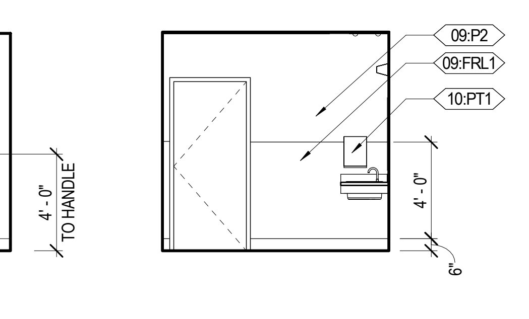
B5 MEN'S RESTROOM 112 - EAST A251 1/4" = 1'-0"
