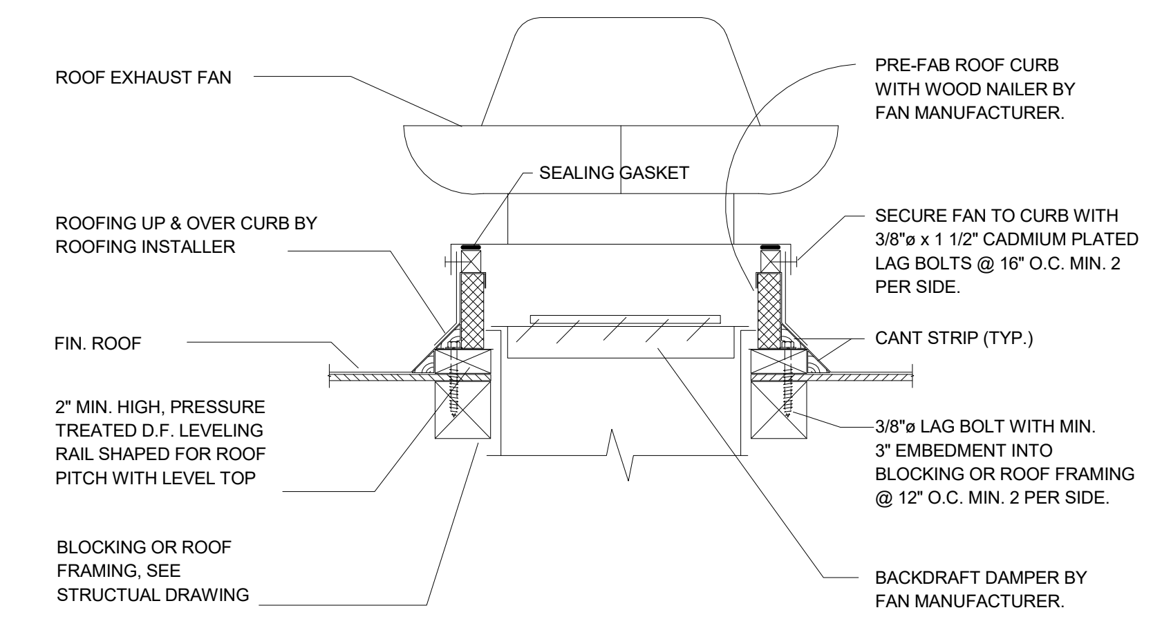
ROOF EXHAUST FAN MOUNTING SCALE: NONE
