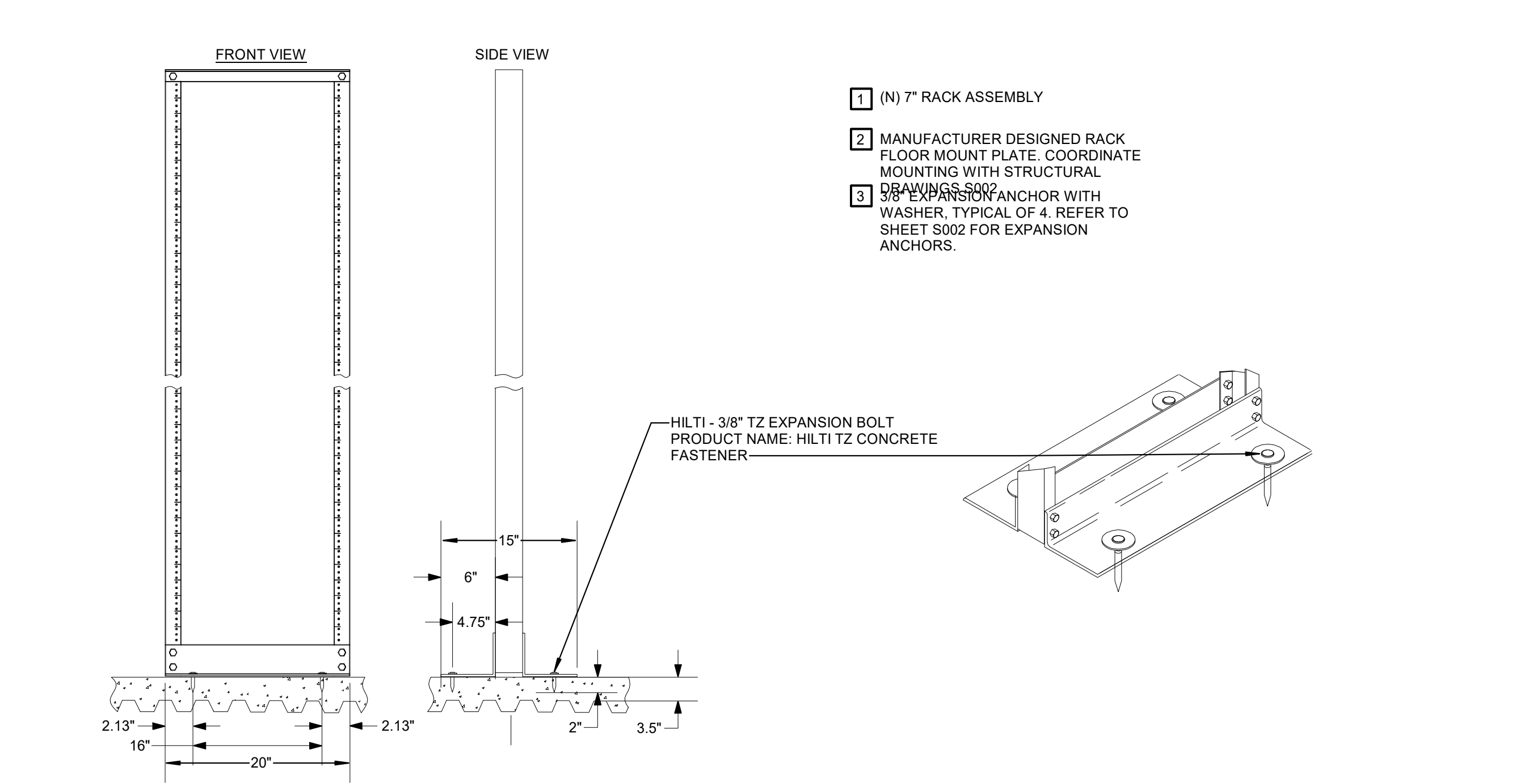
5 Equipment Rack Base Support SCALE: NTS
