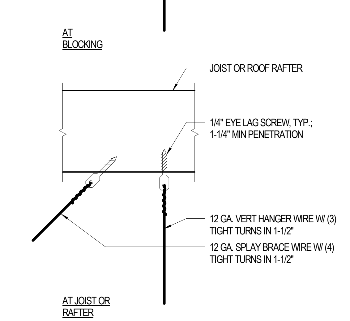
A3 WIRE CONNECTION AT JOIST/RAFTER A701 3" = 1'-0"
