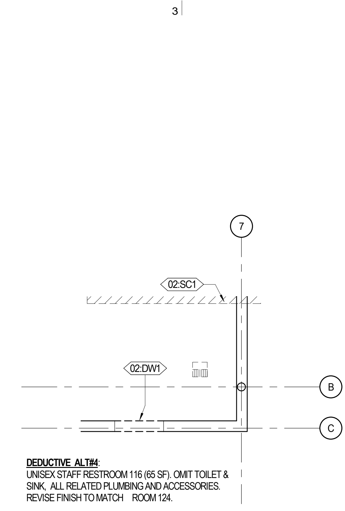
D3 DEMO PLAN DEDUCTIVE ALTERNATE #4 A102 1/4" = 1'-0"
