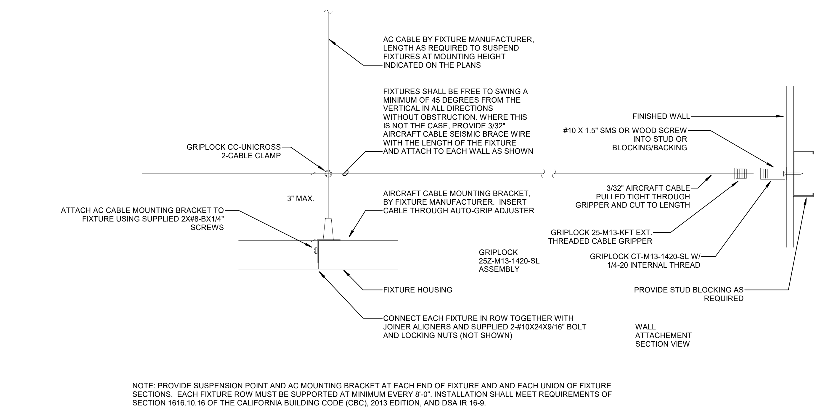
6 Suspended Light Fixtures SCALE: 1/2\" = 1'-0"
