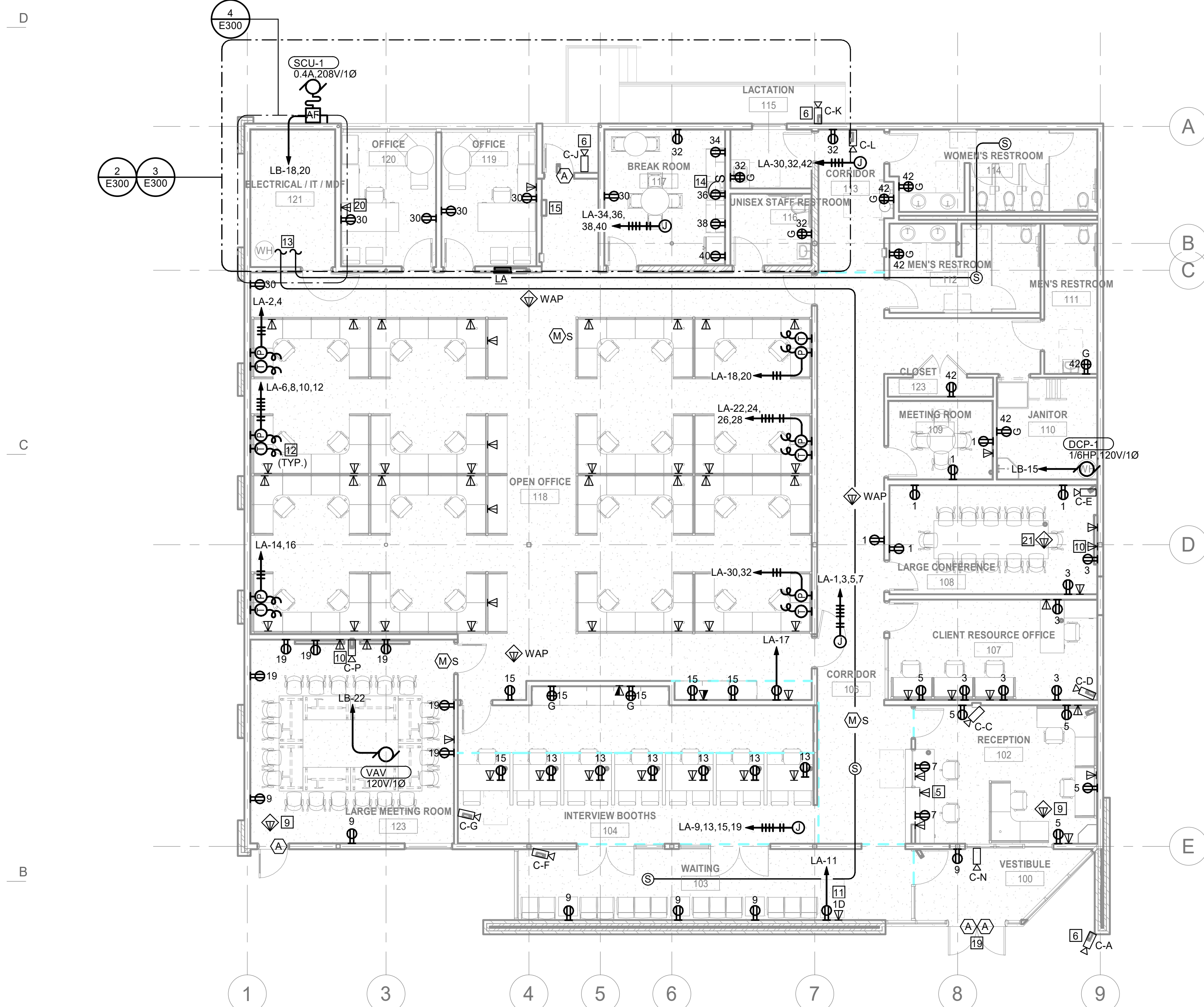
1 POWER & SIGNAL PLAN SCALE: 1/8" = 1'-0"
