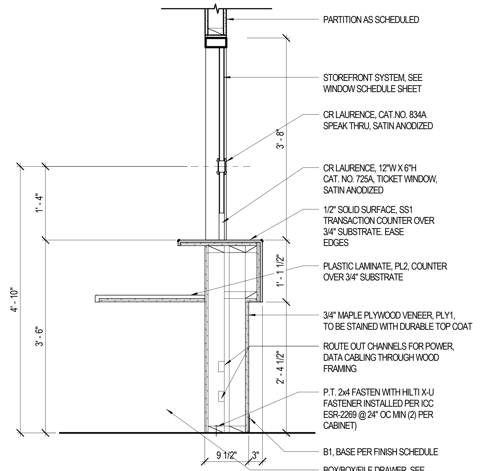
A4 RECEPTION TRANSACTION COUNTER DETAIL A501 1" = 1'-0"
