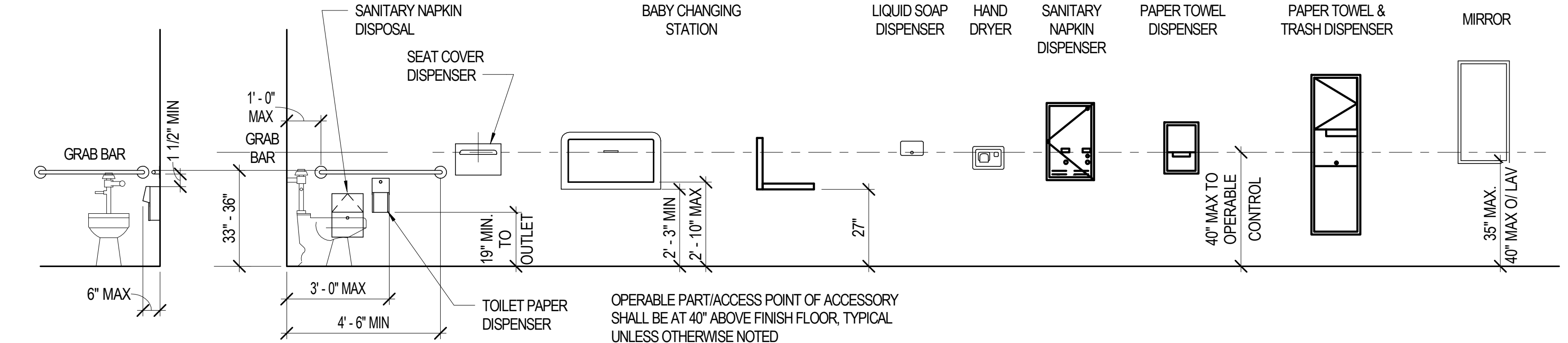
C4 RESTROOM MOUNTING HEIGHTS G701 3/8" = 1'-0"
