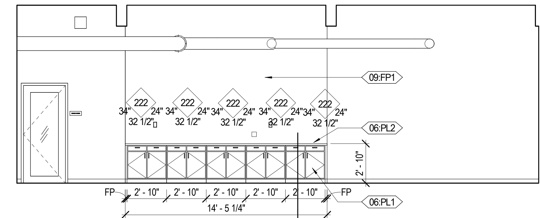
E1 STAFF WORK BOOTHS 105 - NORTH A251 1/4" = 1'-0"
