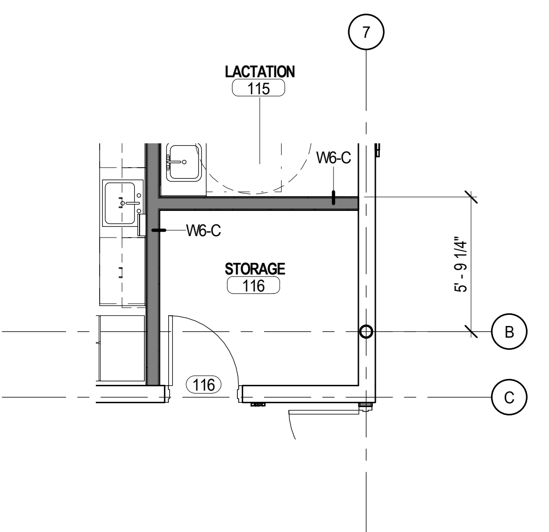
C3 FLOOR PLAN DEDUCTIVE ALTERNATE #4 A102 1/4" = 1'-0"
