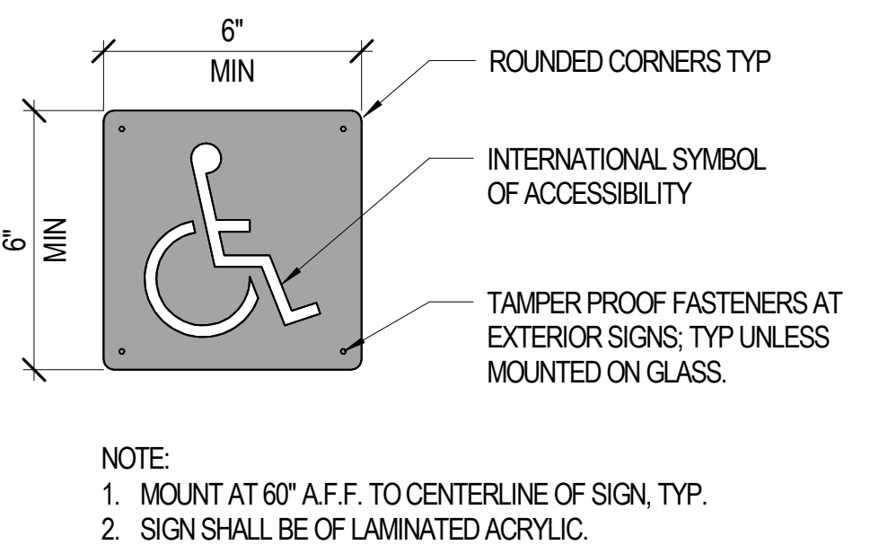
C1 SYMBOL OF ACC. SIGN G701 3" = 1'-0"
