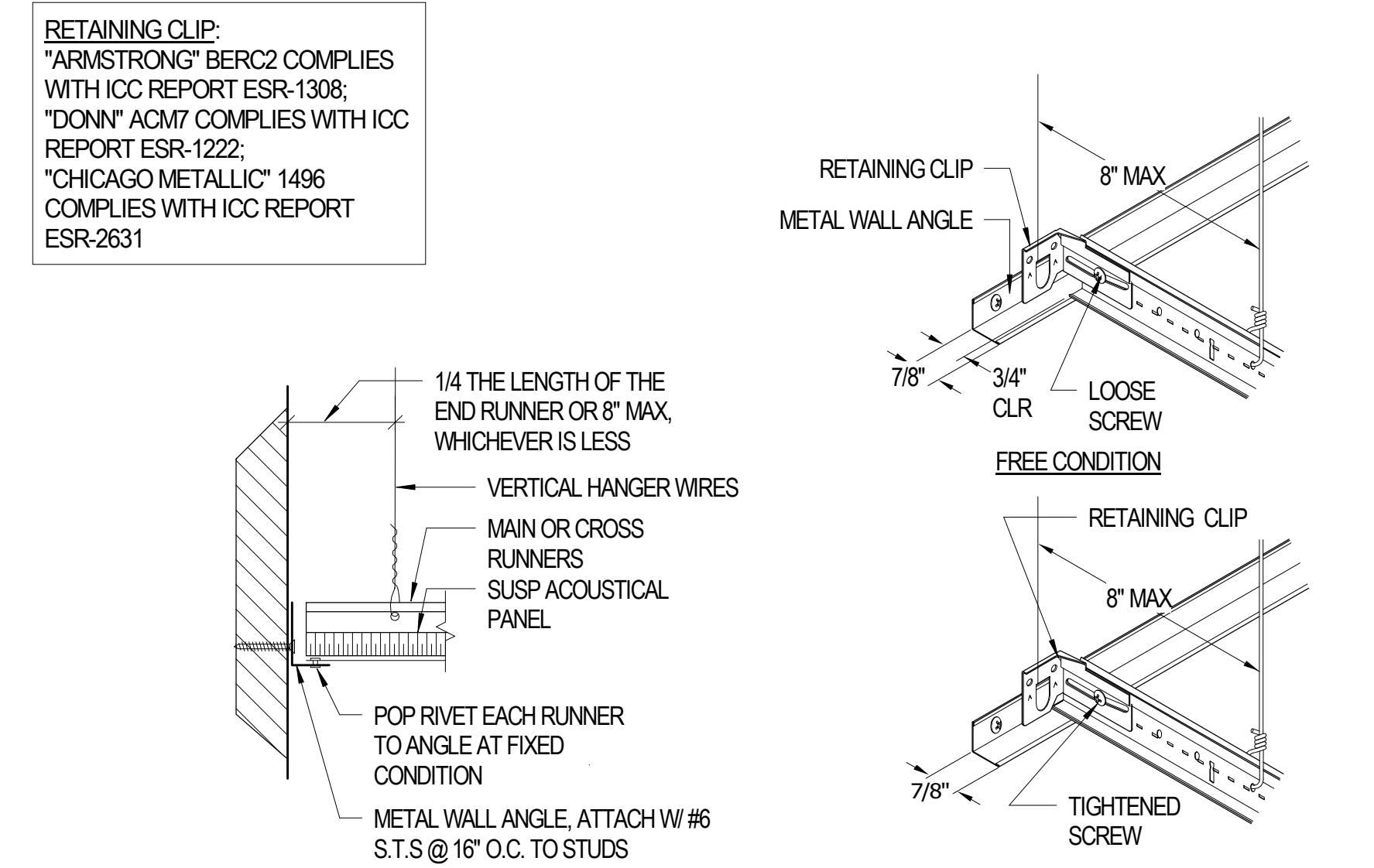
SUSPENDED CEILING AT WALL SCALE: 3" = 1'-0"
