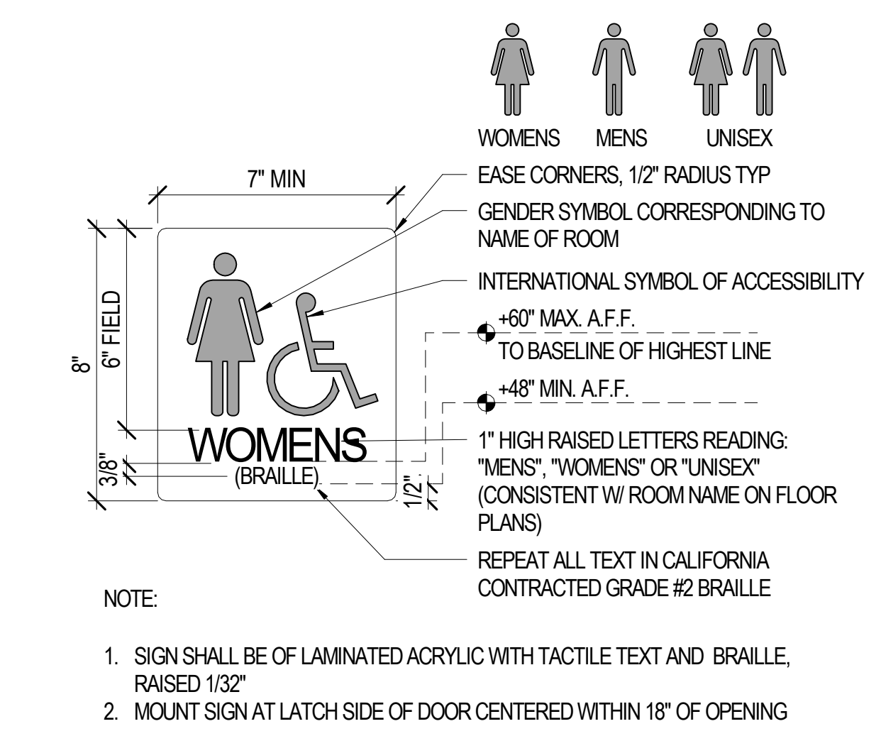
B6 TOILET ROOM IDENTIFICATION SIGN G701 3" = 1'-0"
