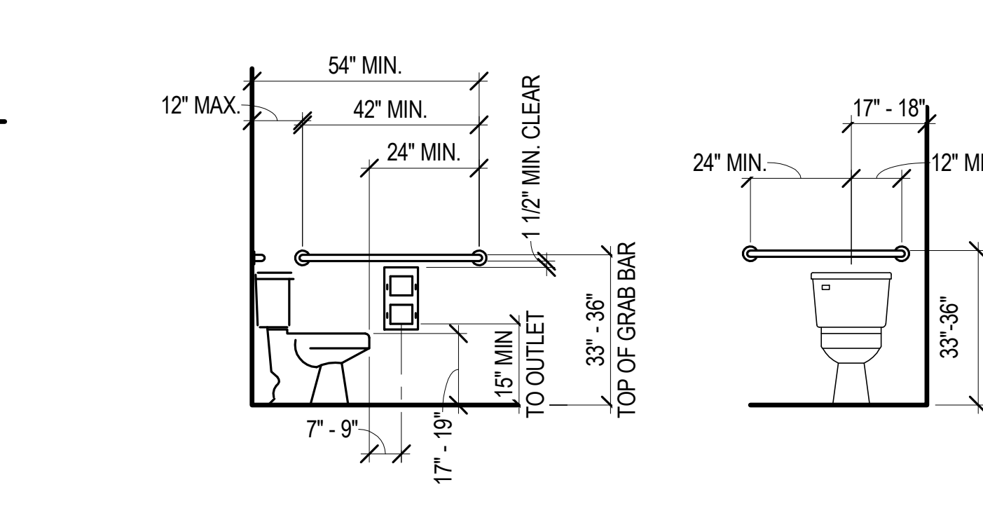
A3 ACCESSIBLE FLOOR MOUNTED TOILET DETAIL G701 3/8" = 1'-0"
