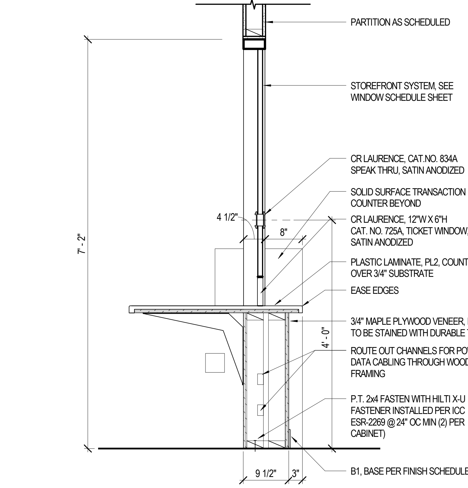
A3 RECEPTION ACCESSIBLE COUNTER DETAIL A501 1" = 1'-0"
