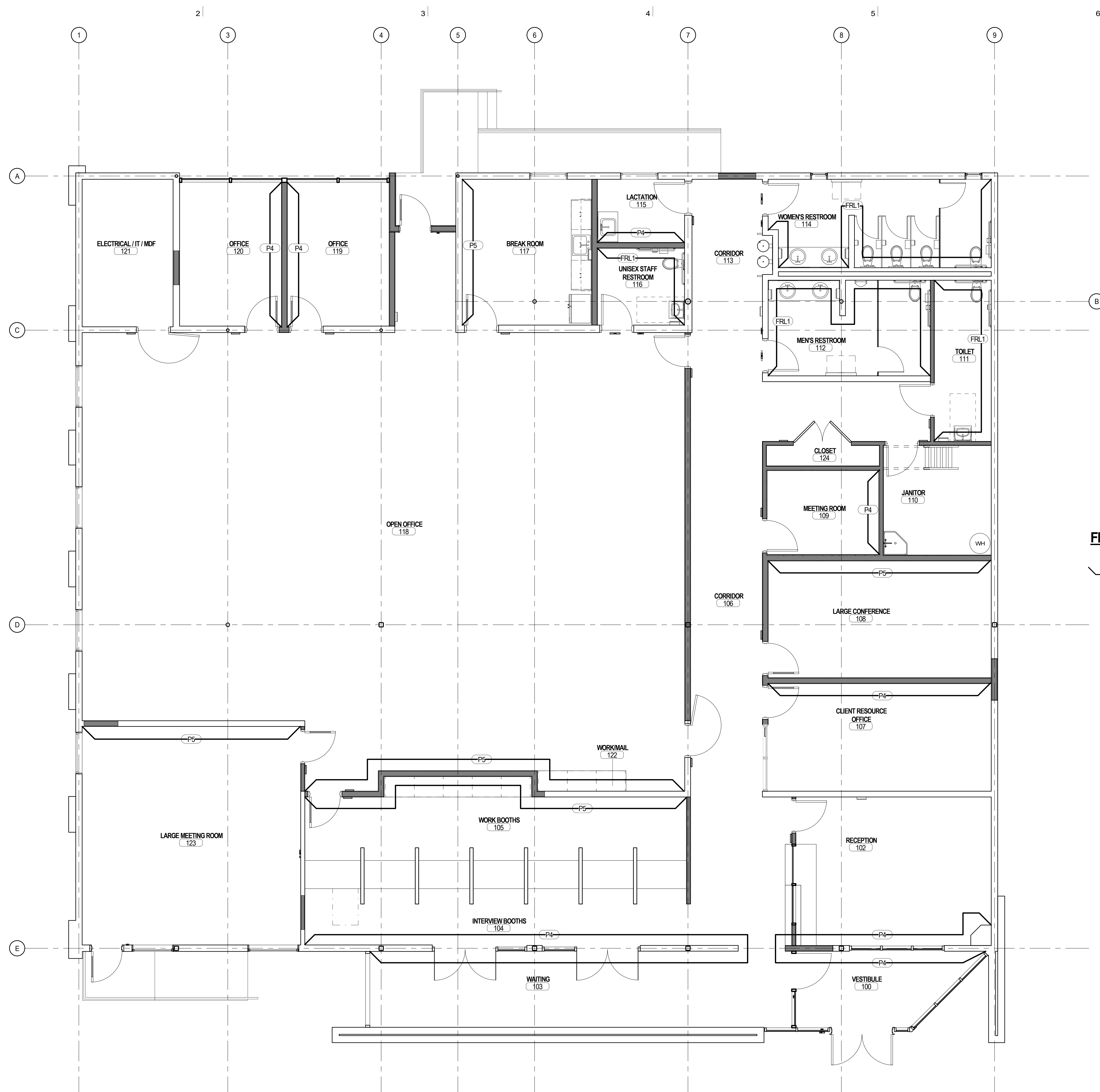
A1 LEVEL 01 - FINISH FLOOR PLAN 1/4" = 1'-0"
