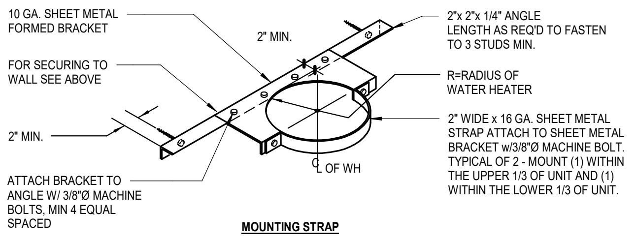
4 WATER HEATER STRAP MOUNTING SCALE: NOT TO SCALE
