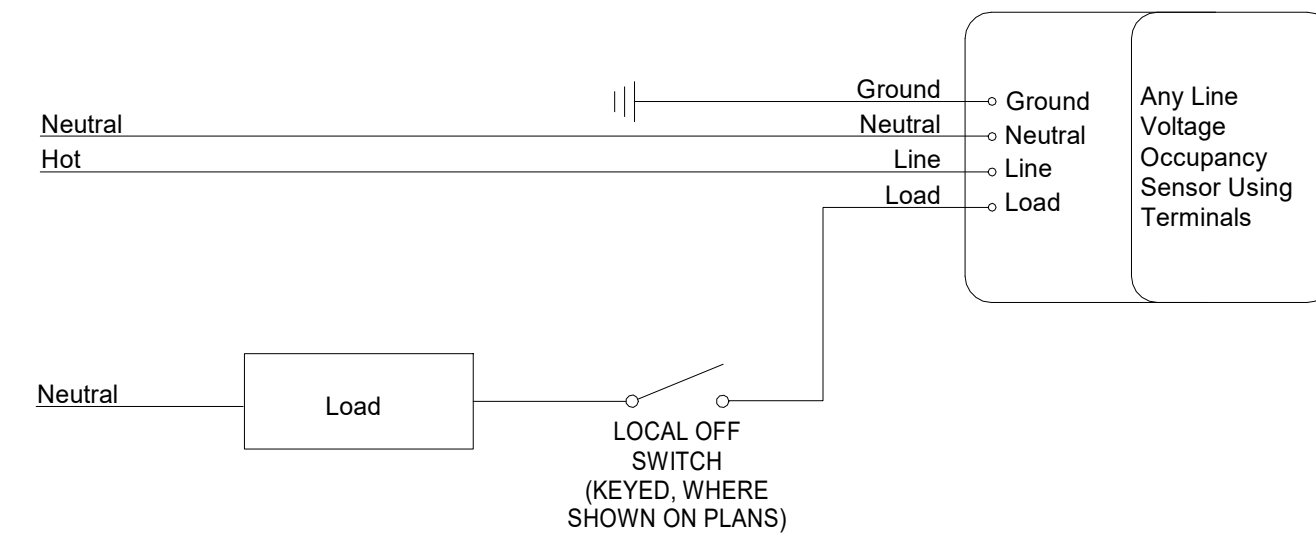
LINE VOLTAGE CEILING MOUNTED DUAL-TECHNOLOGY OCCUPANCY SENSOR Typical at multi-user restrooms Set time delay to 20 min., sensitivity to max.
