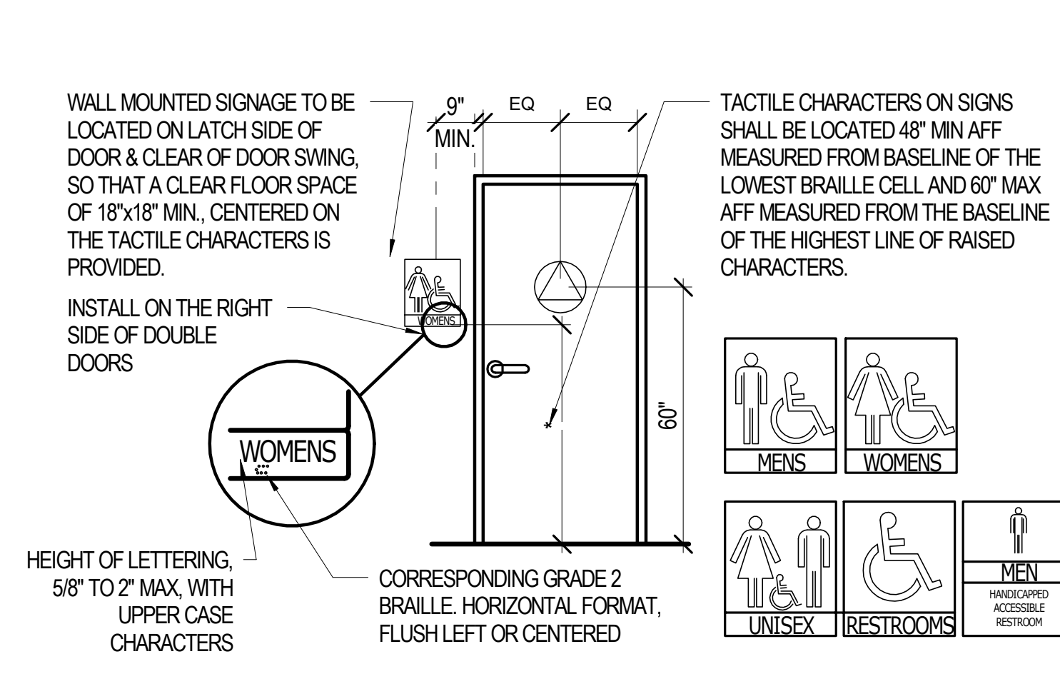
C4 RESTROOM MOUNTING HEIGHTS G701 3/8" = 1'-0"
