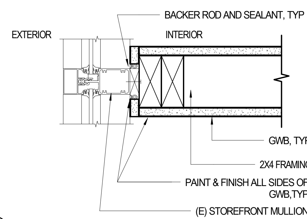
C3 INTERIOR STOREFRONT JAMB A A602 3" = 1'-0"
