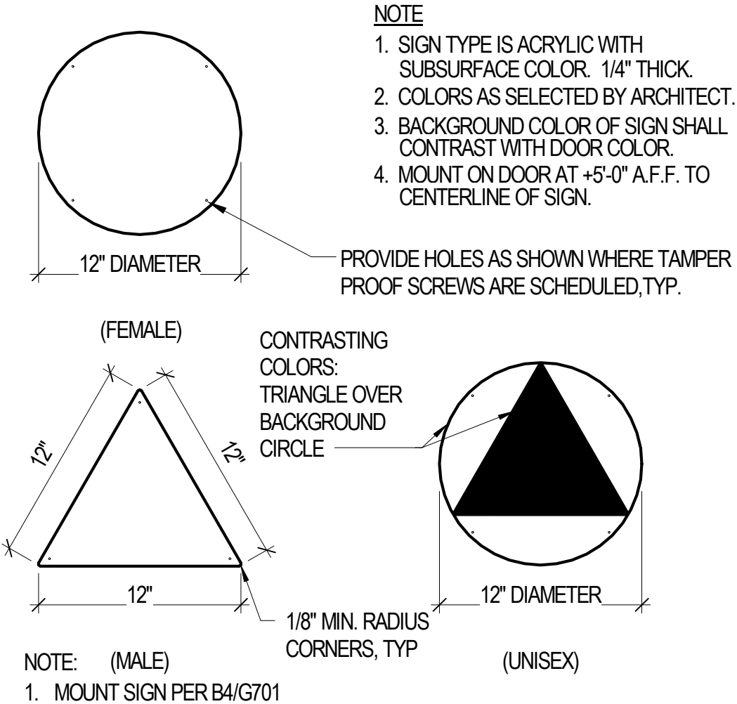
B1 TOILET ROOM DOOR SIGNS G701 1 1/2" = 1'-0"
