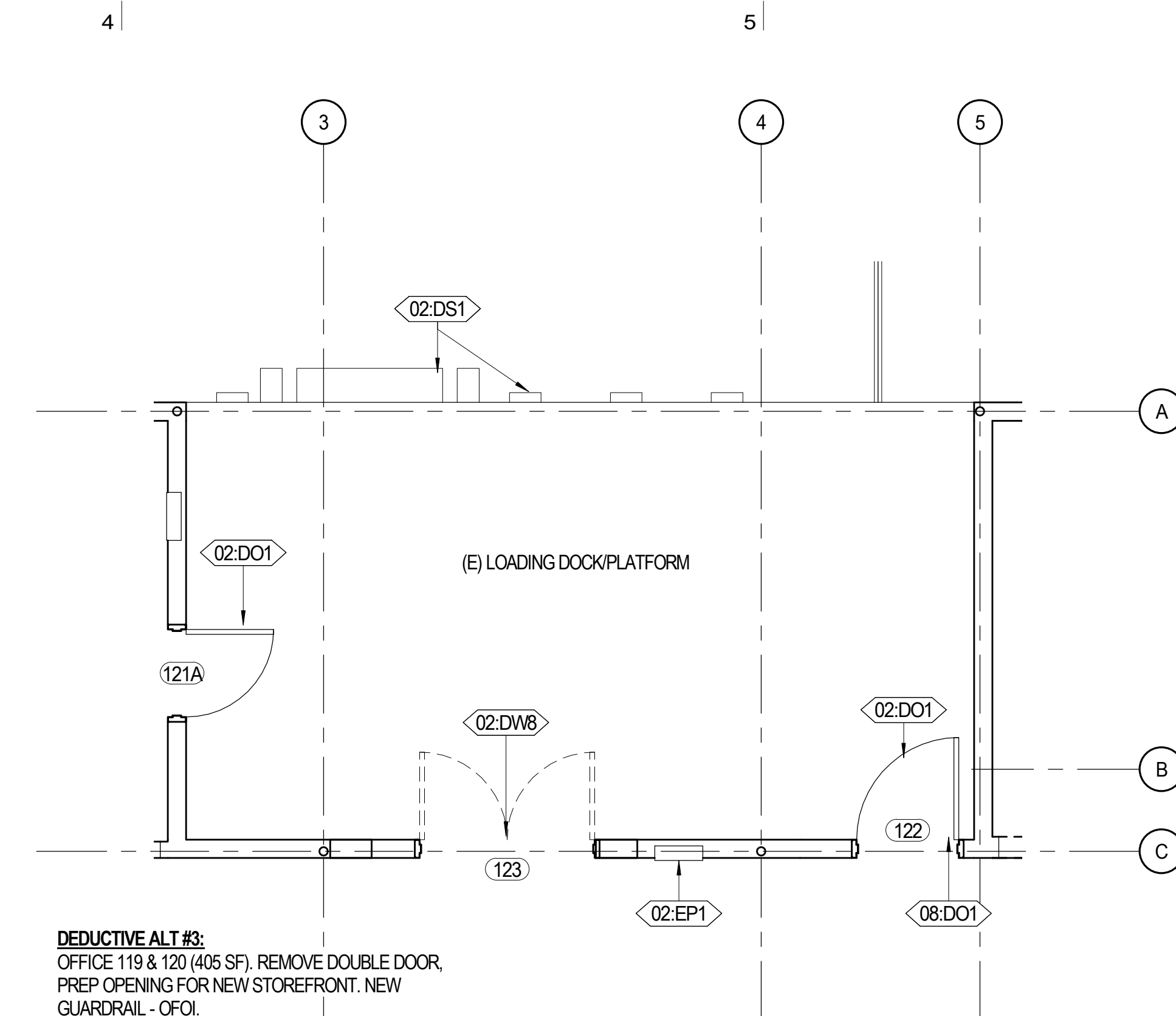
D4 DEMO FLOOR PLAN DEDUCTIVE ALTERNATE #3 A102 1/4" = 1'-0"
