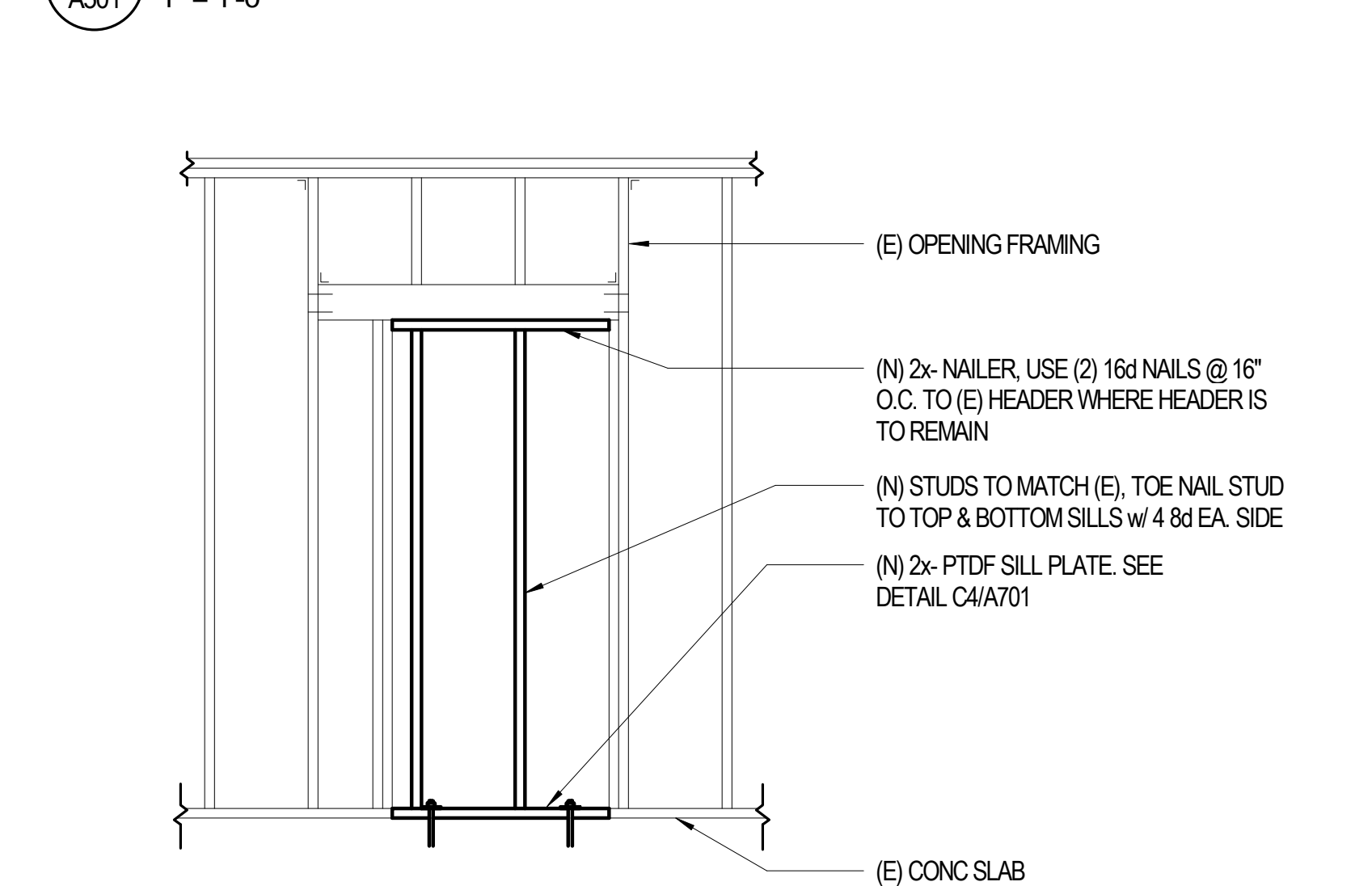
C2 TYPICAL INFILL FRAMING A501 1/2" = 1'-0"
