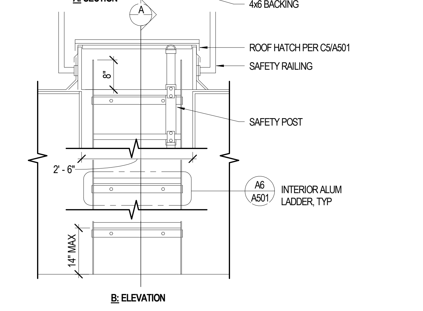
B3 ROOF HATCH LADDER A501 3/4" = 1'-0"
