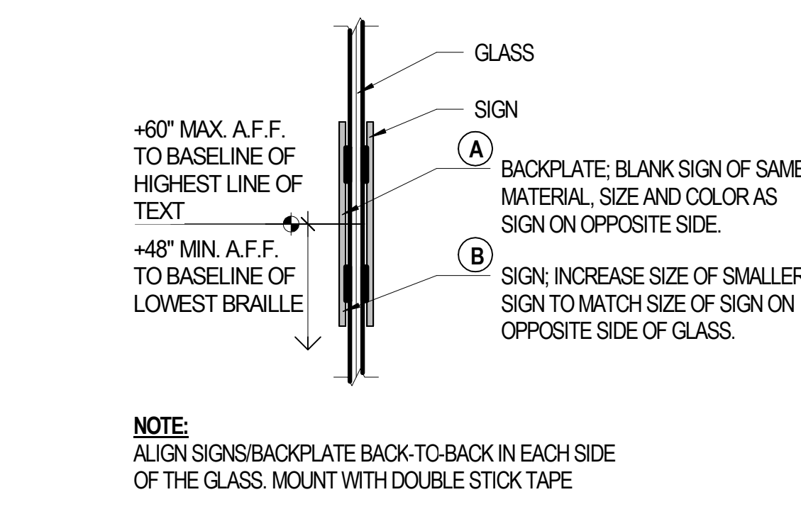
D3 SIGN MOUNTED ON GLASS G701 6" = 1'-0"
