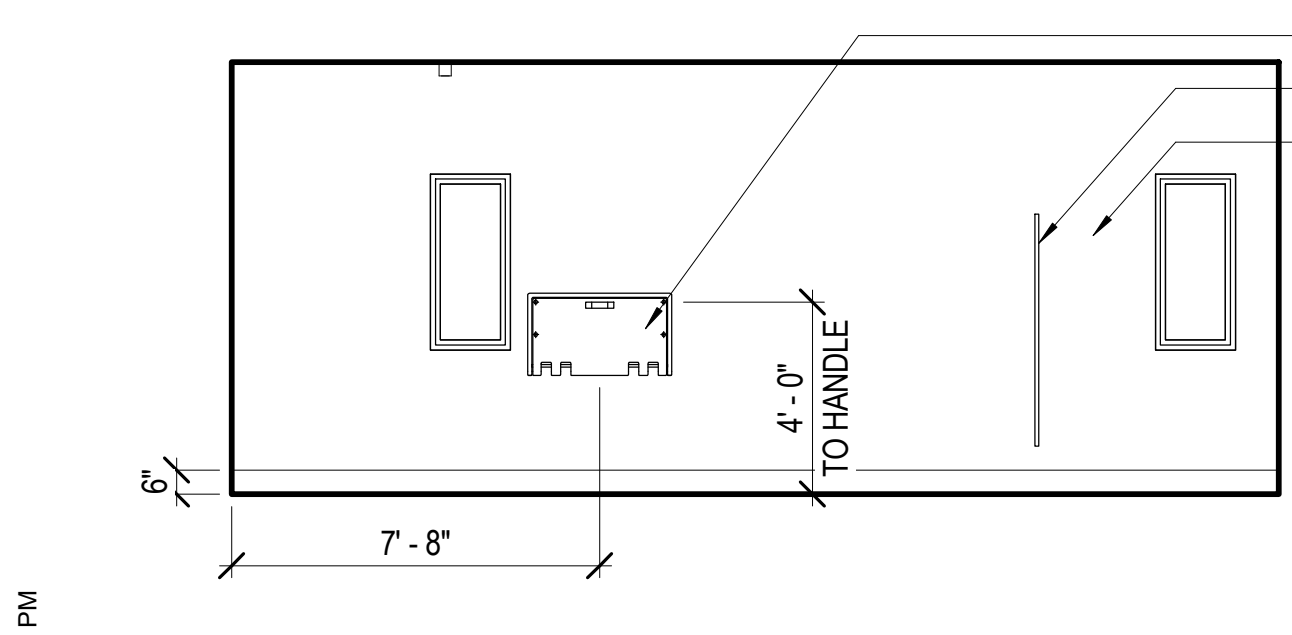
A1 WOMEN'S RESTROOM 114 - SOUTH A251 1/4" = 1'-0"
