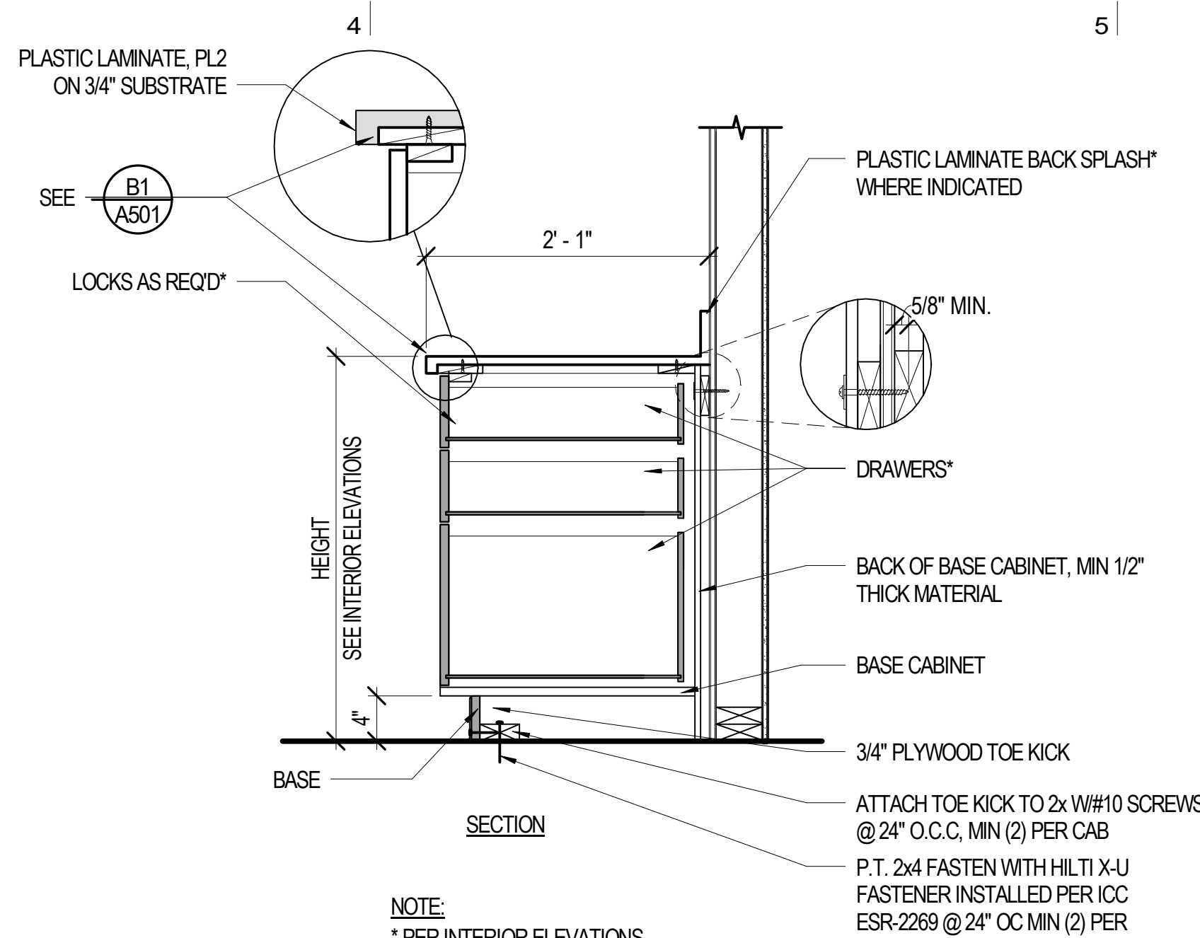
D3 BASE CABINETS - DRAWERS A501 1" = 1'-0"
