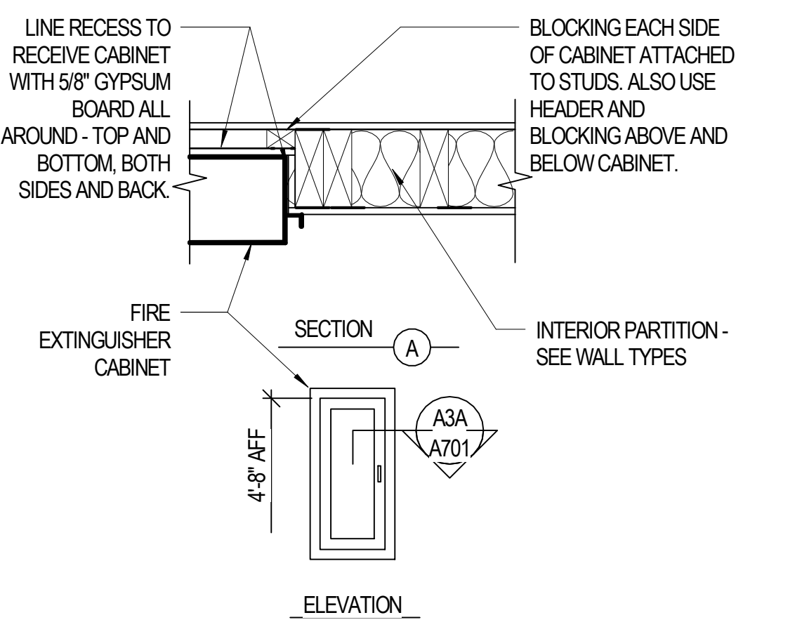
C3 FIRE EXTINGUISHER CAB. DETAIL 02 A701 3" = 1'-0"
