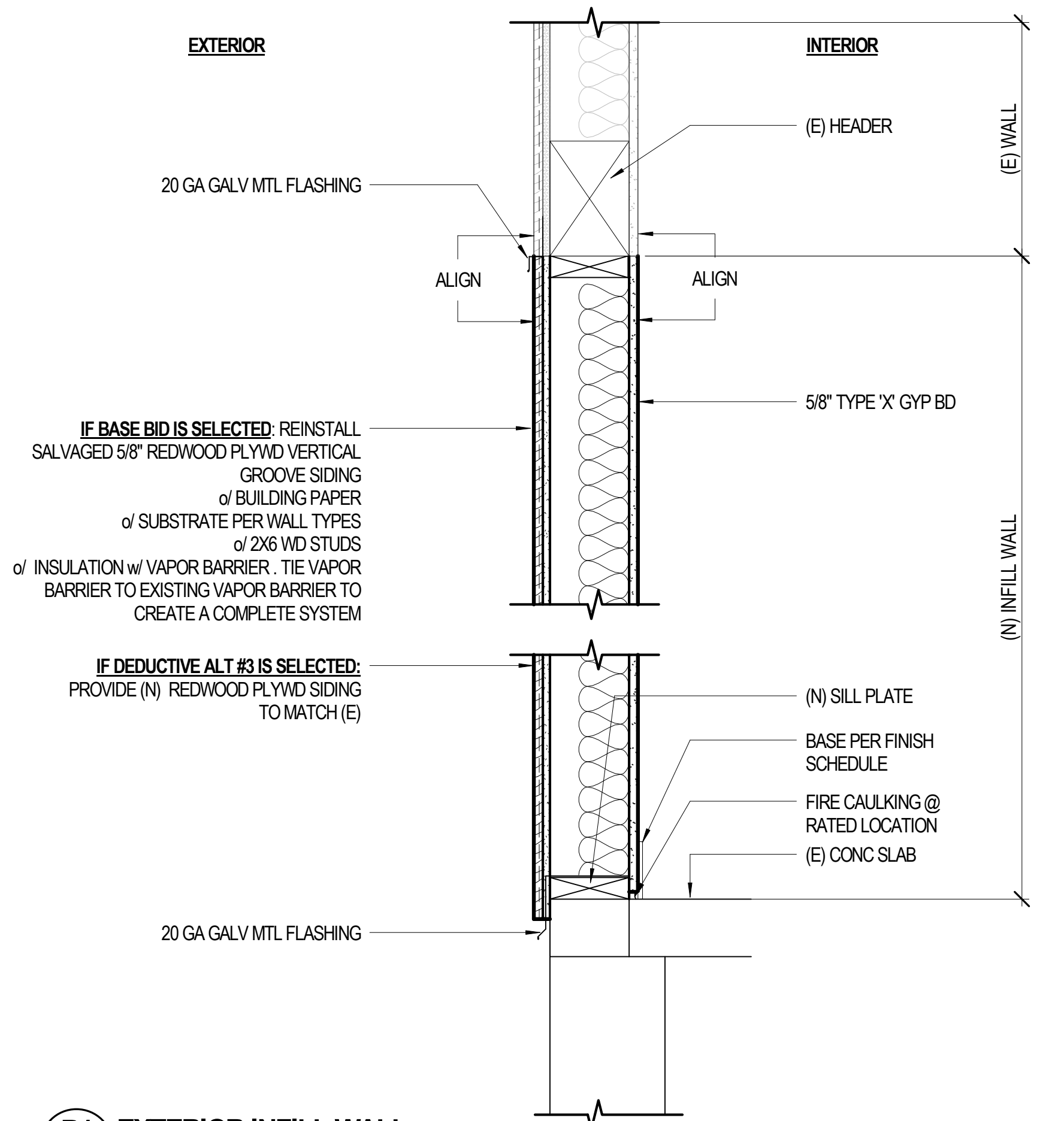
B1 EXTERIOR INFILL WALL G501 1 1/2" = 1'-0"
