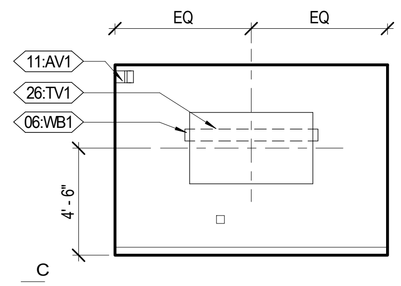
C1 LARGE CONFERENCE 108 - WEST A251 1/4" = 1'-0"
