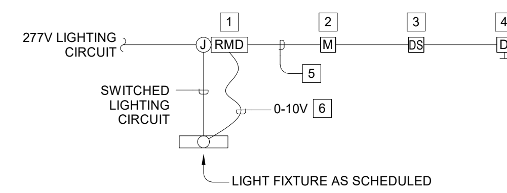
STAND-ALONE NETWORK LIGHTING CONTROLS Not all devices shown on this wiring diagram will be used in each room, refer to plans for actual device requirements. All zones automatic on, time delay 15 minutes. Daylight Harvesting set point at 35 foot candles. Typical.
