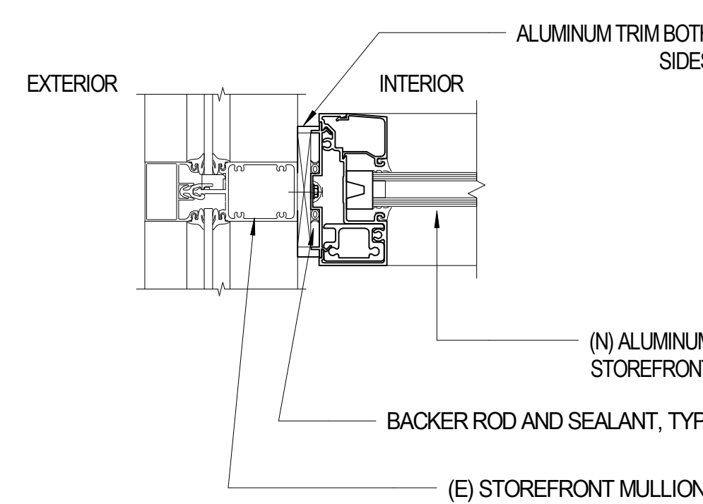
B3 INTERIOR STOREFRONT JAMB B A602 3" = 1'-0"
