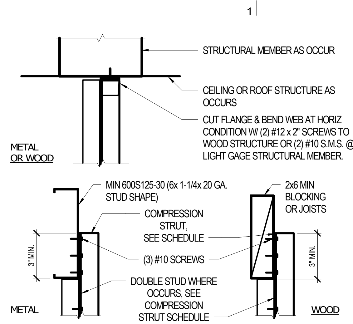
E2 COMPRESSION STRUT ANCHORAGE A701 3" = 1'-0"
