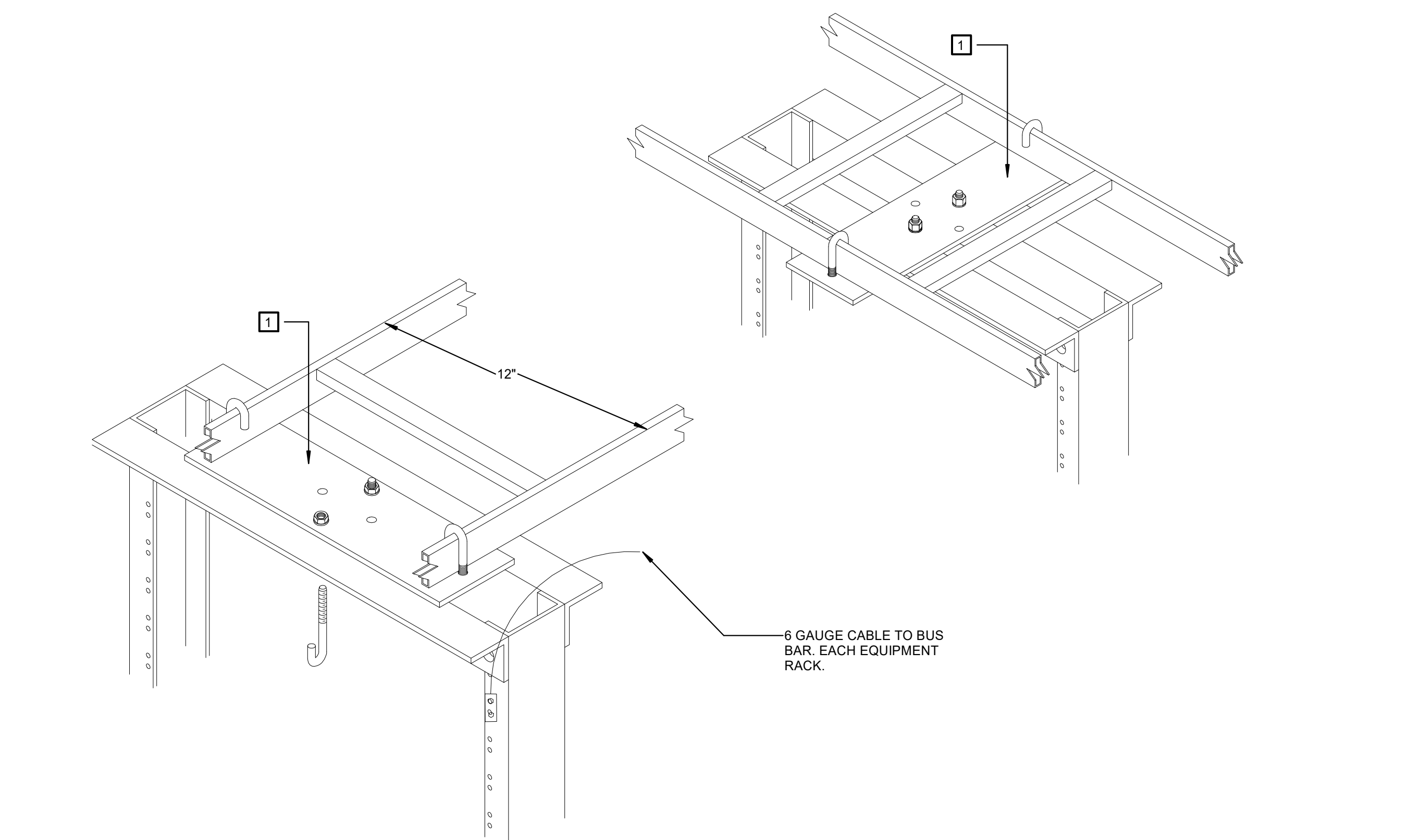
7 Ladder to Rack Support SCALE: NTS
