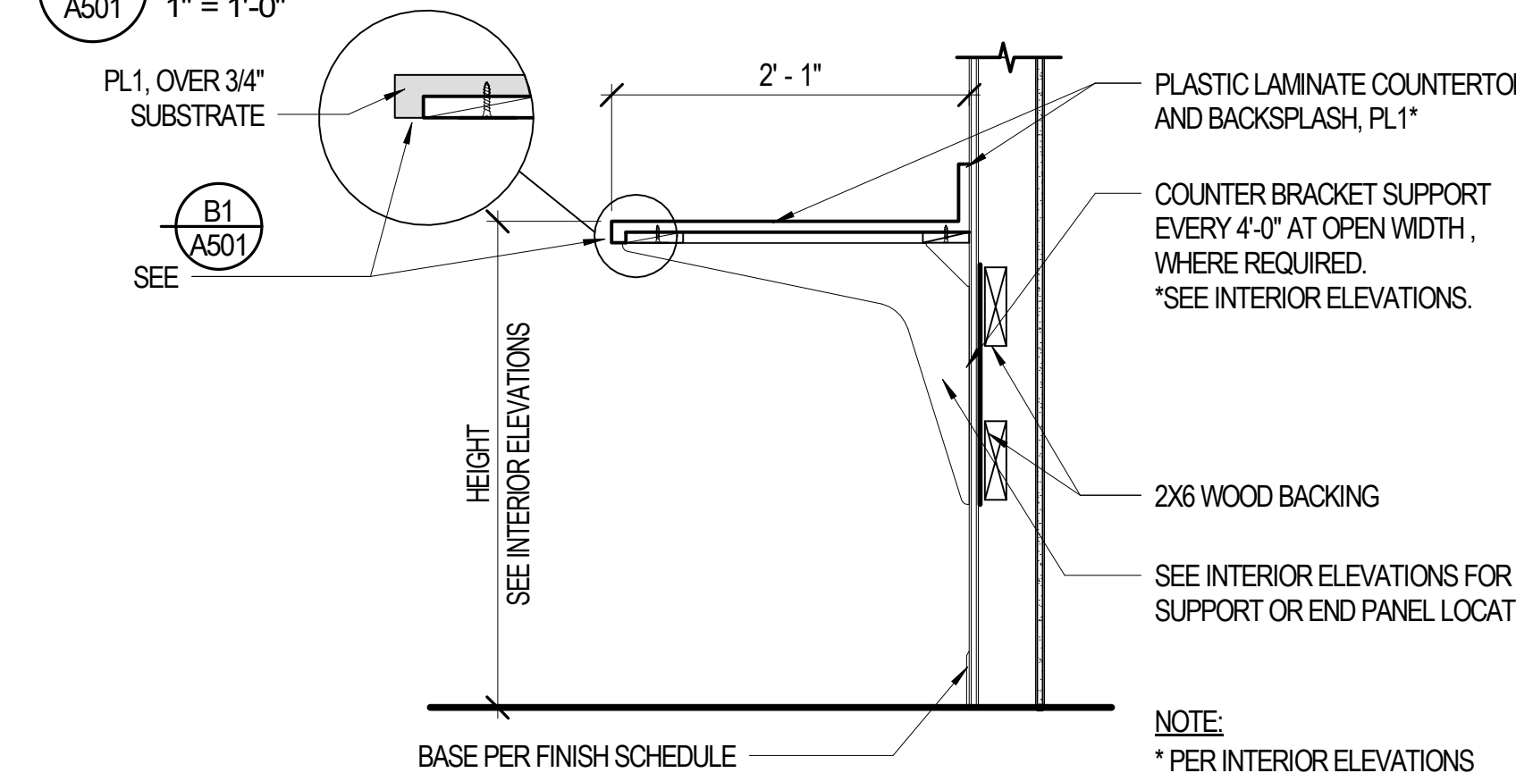
2 OPEN COUNTERTOP WITH SUPPORT A501 1" = 1'-0"
