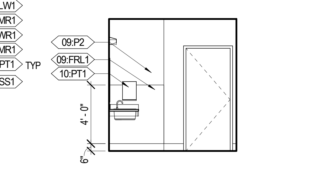
A4 WOMEN'S RESTROOM 114 - EAST A251 1/4" = 1'-0"
