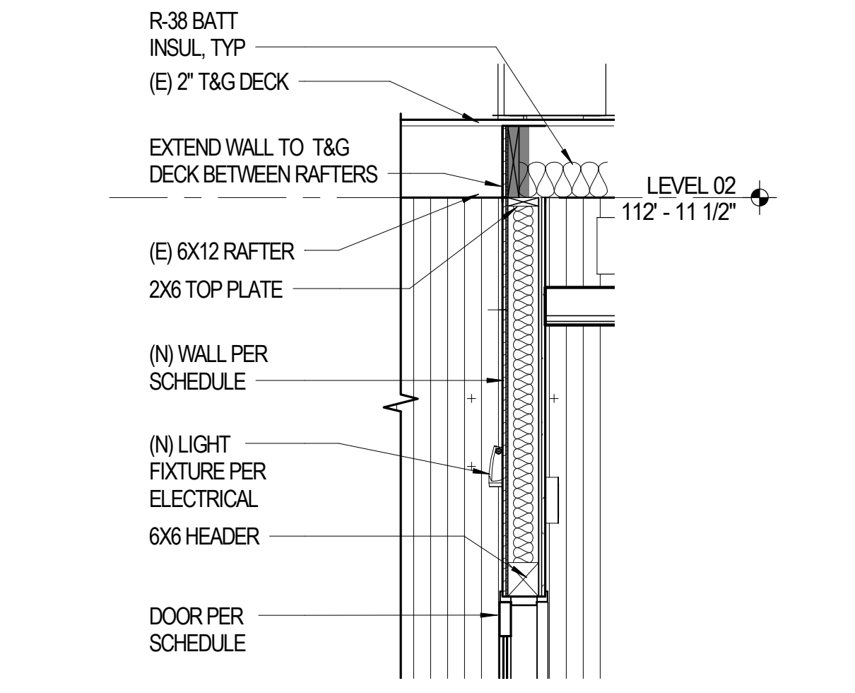
4 WALL SECTION G501 1/2" = 1'-0"
