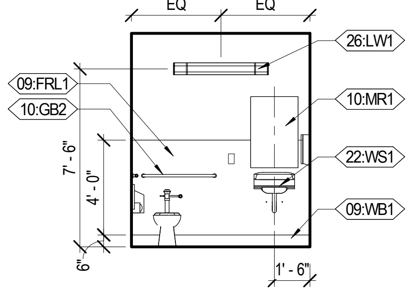
E2 UNISEX STAFF RESTROOM 116 - WEST A252 1/4" = 1'-0"
