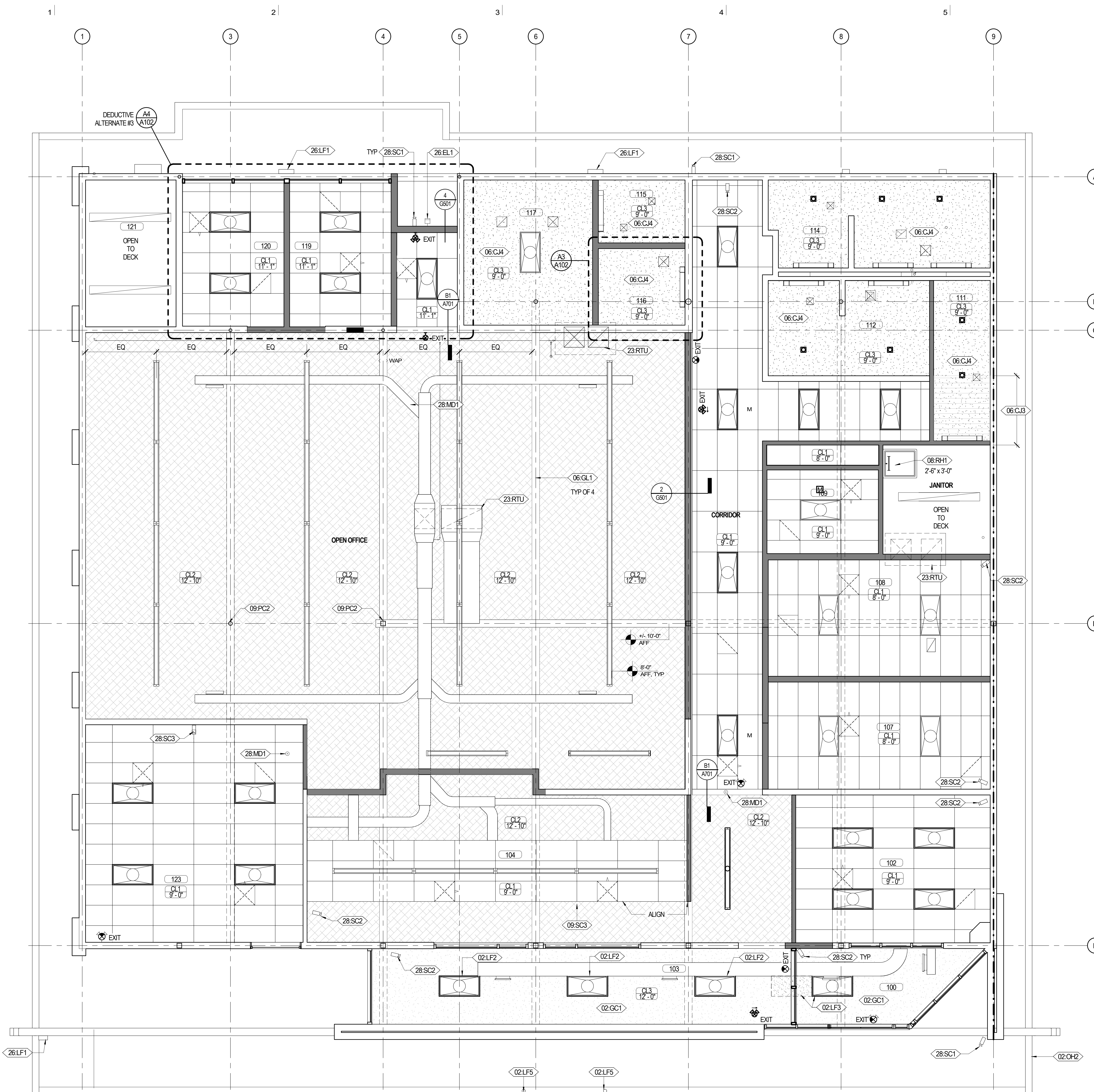
A1 LEVEL 01 - REFLECTED CEILING PLAN A151 1/4" = 1'-0"
