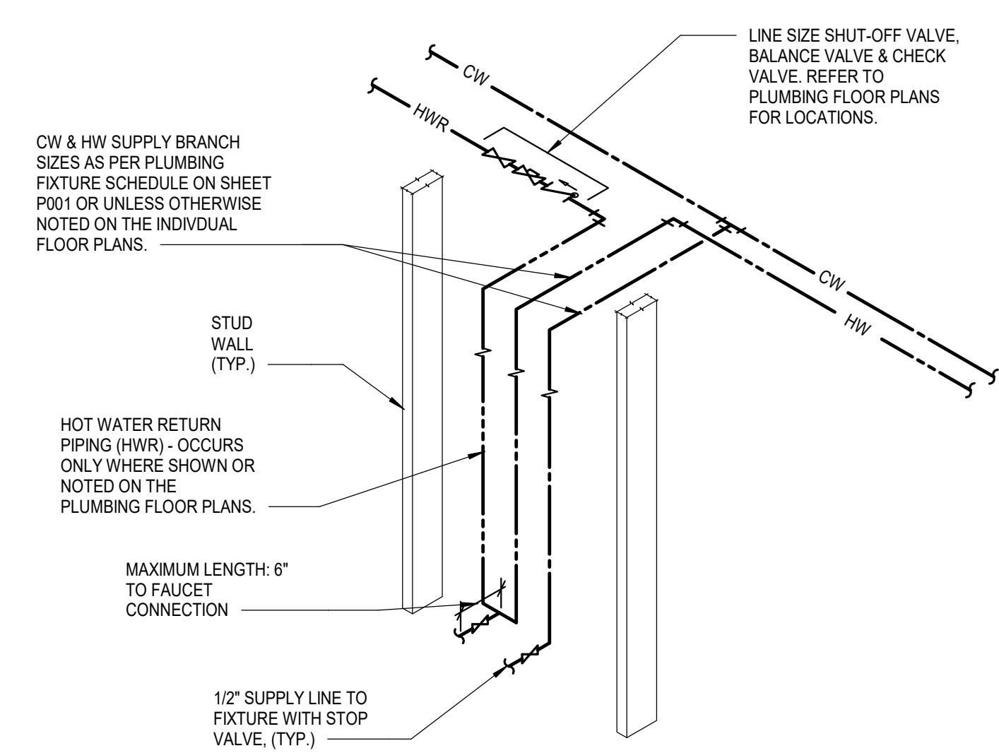
2 TRAP PRIMER TO FLOOR DRAIN SCALE: NOT TO SCALE
