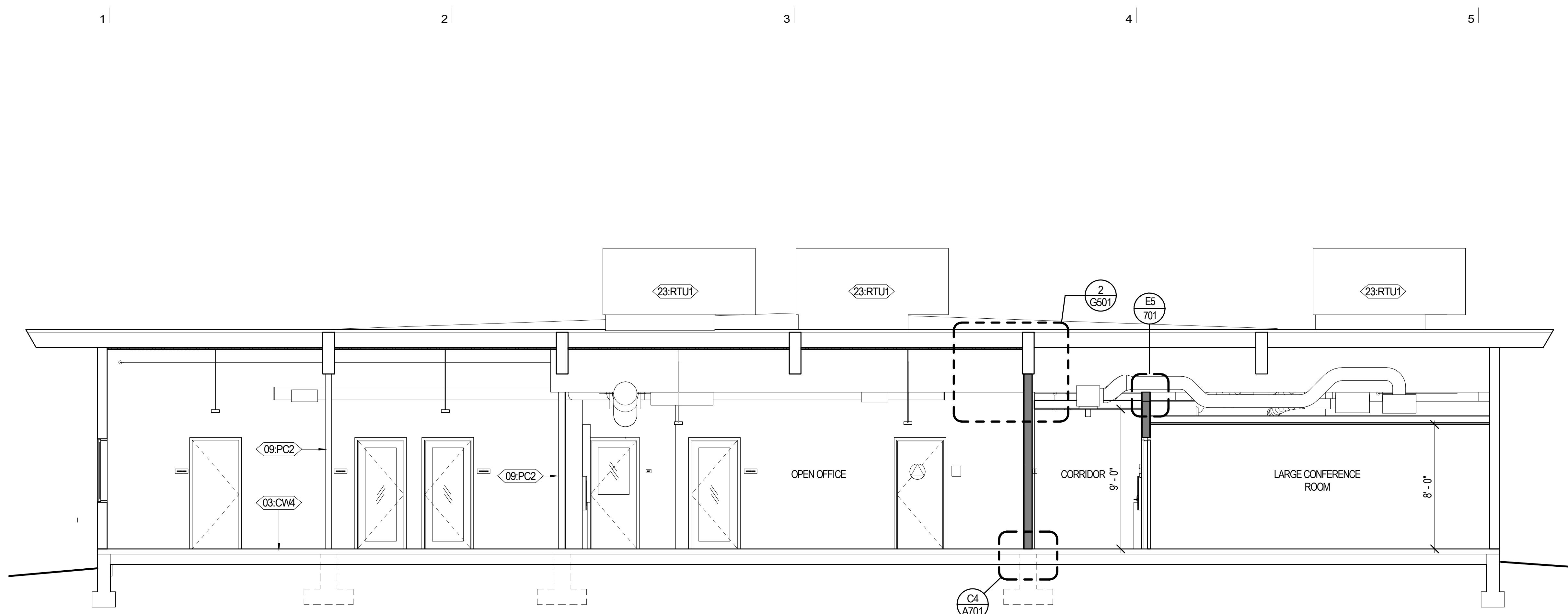
D1 BUILDING SECTION A A301 1/4" = 1'-0"
