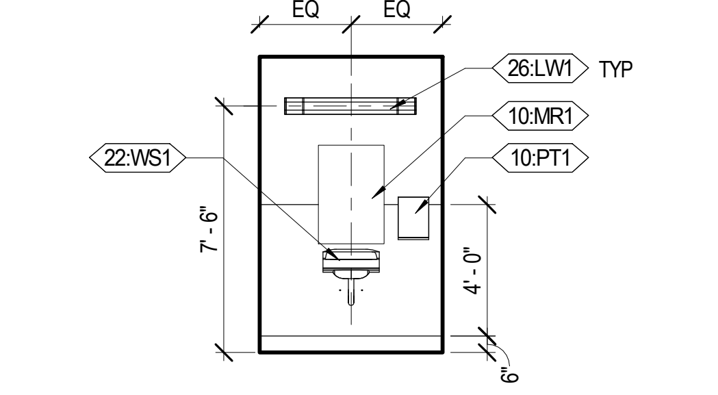
C5 TOILET 111 - NORTH A251 1/4" = 1'-0"
