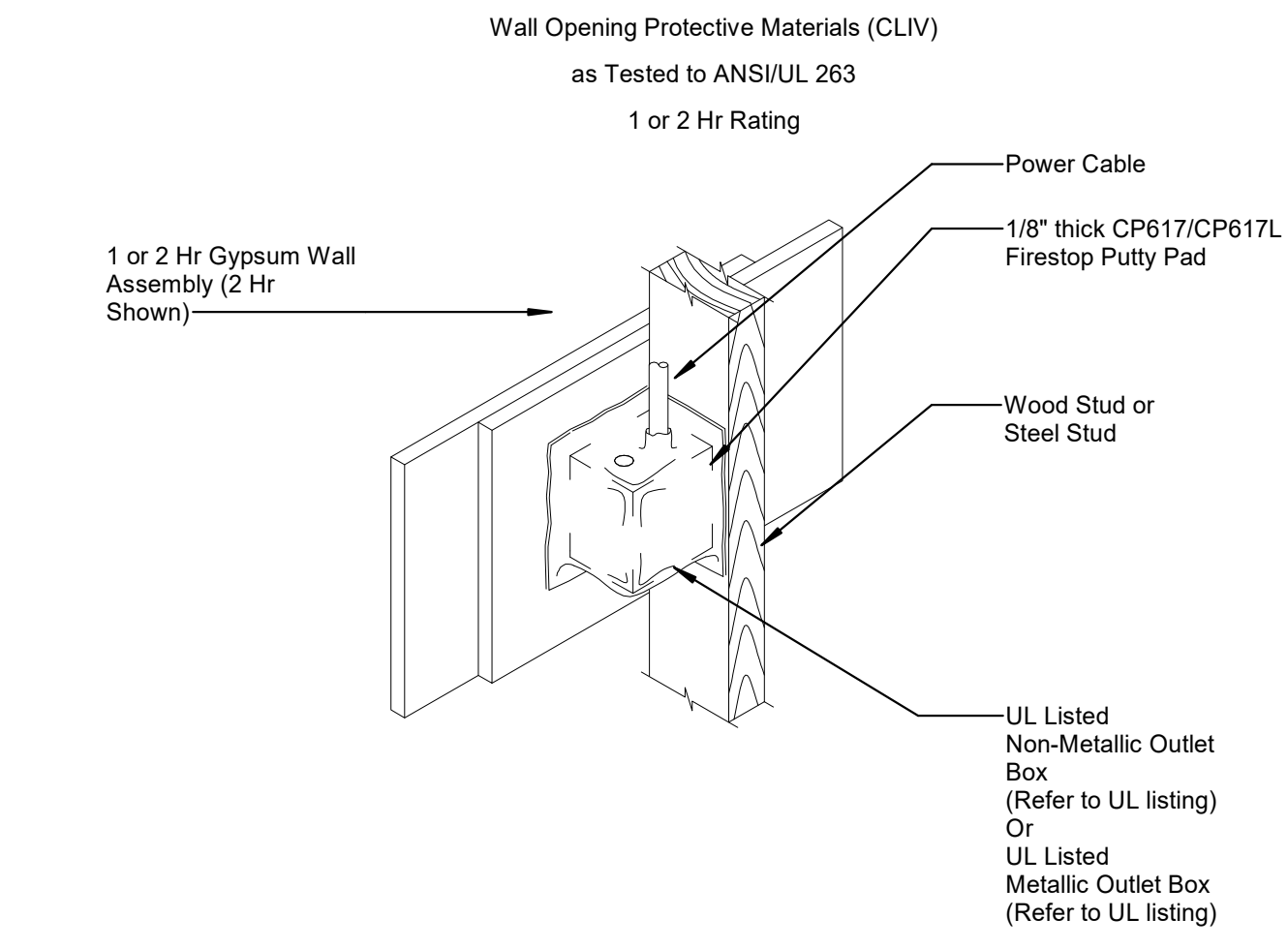
1 Rated Penetration Detail SCALE: NTS
