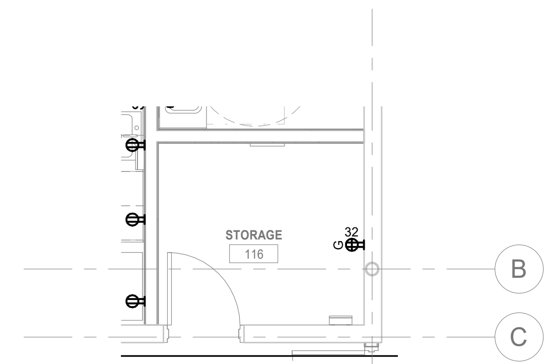
2 POWER & SIGNAL PLAN - ALT#3 SCALE: 1/4" = 1'-0"
