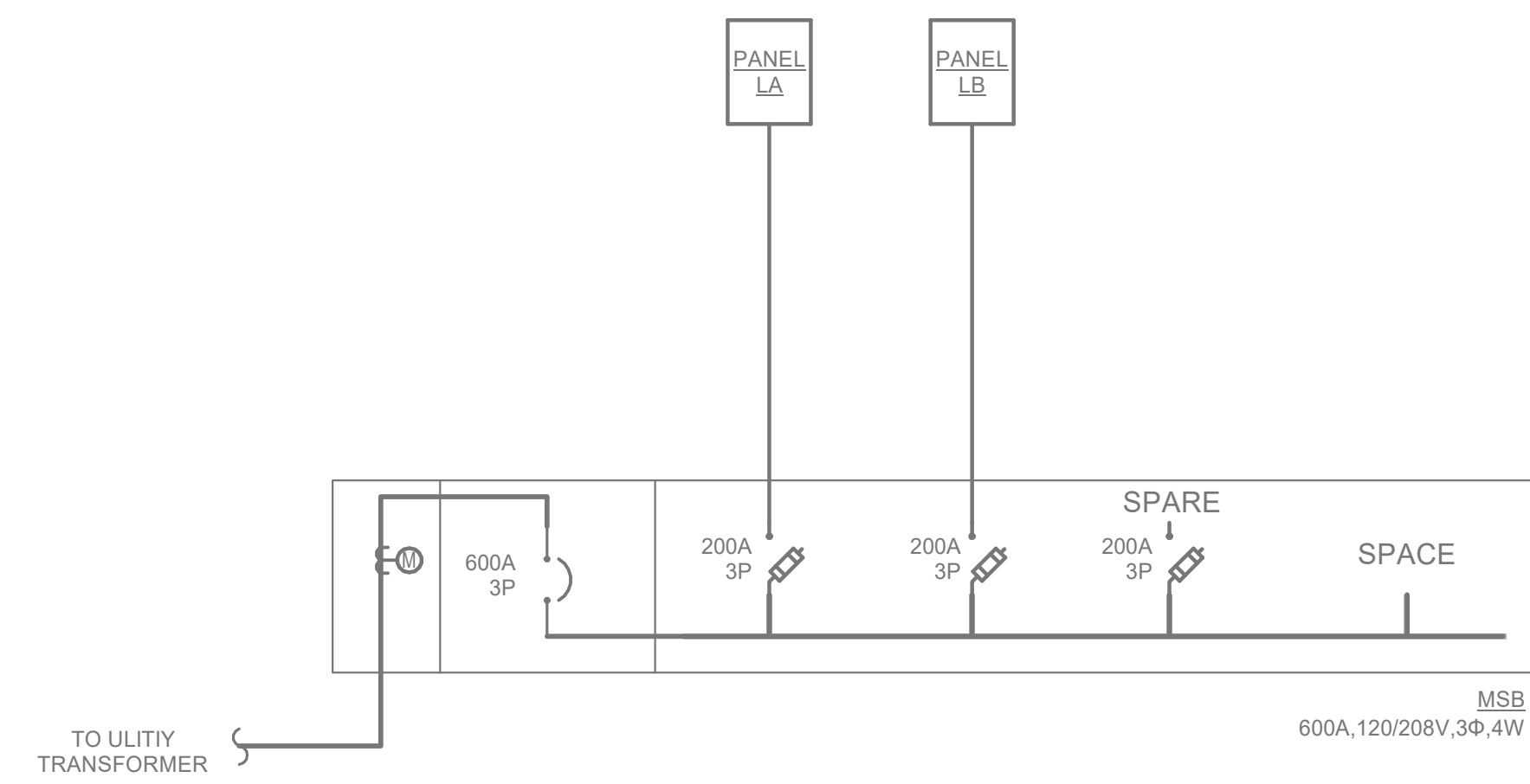
1 POWER ONE-LINE DIAGRAM SCALE: 12" = 1'-0"
