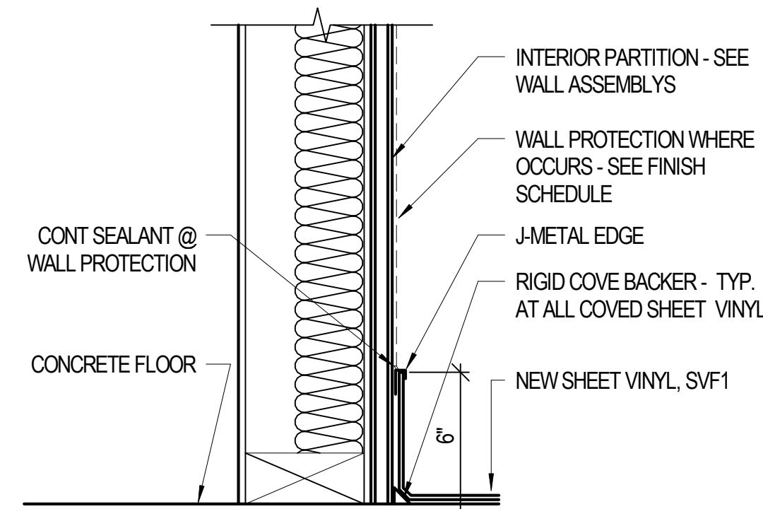
1 INTEGRAL COVERED BASE DETAIL AI602 3" = 1'-0"
