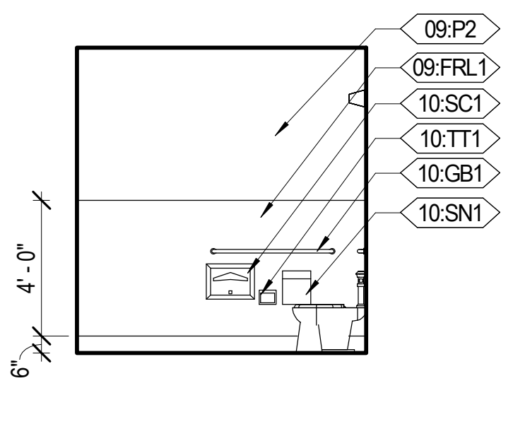
E1 UNISEX STAFF RESTROOM 116 - SOUTH A252 1/4" = 1'-0"
