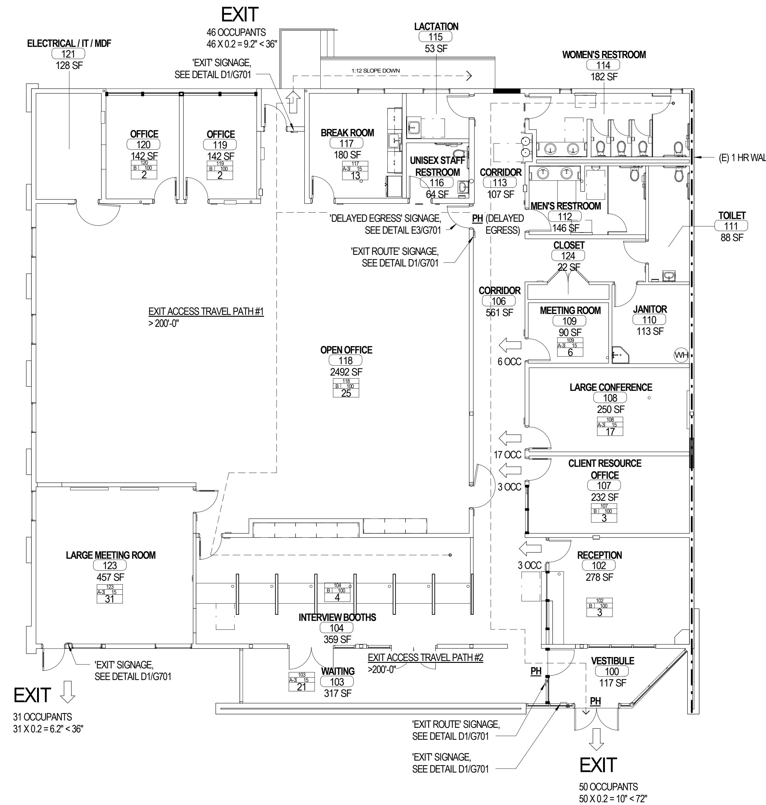
B1 LEVEL 01 - EXITING AND OCCUPANCY PLANS G101 1/8" = 1'-0"
