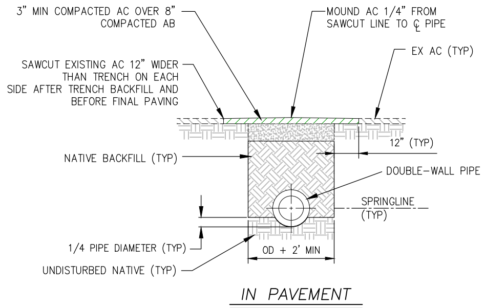
3 PIPE TRENCH NO SCALE
