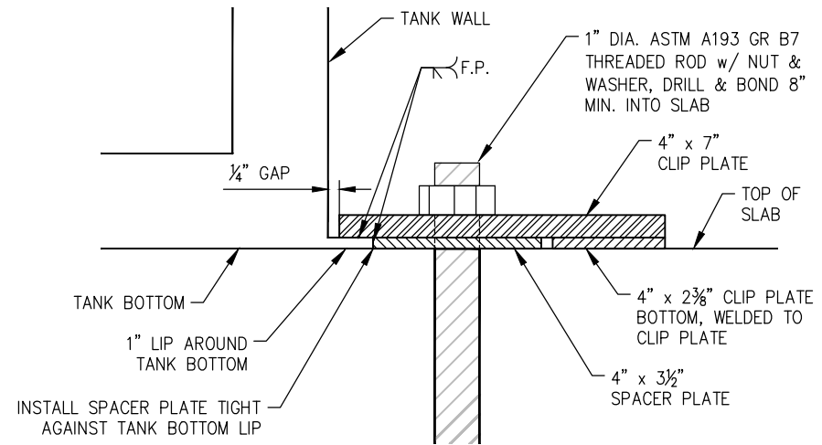
2 ANCHORAGE DETAIL NO SCALE
