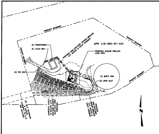
3 OVERALL SITE PLAN SCALE: 1" = 60'
