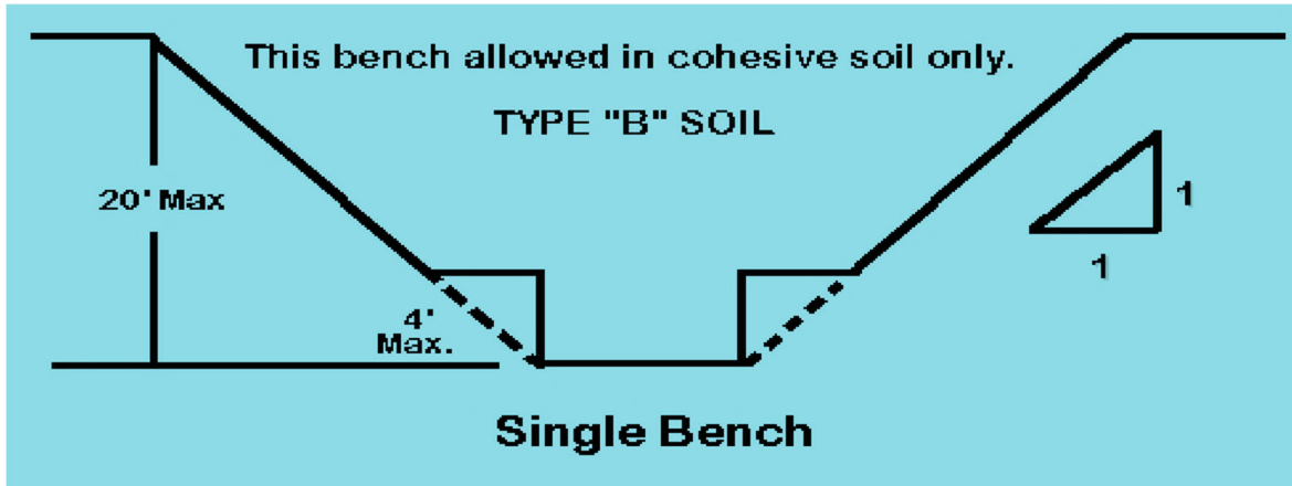
Figure 3: All benched excavations 20 feet or less in depth shall have a maximum allowable slope of 1:1. Benching is not allowed in type C soil.
