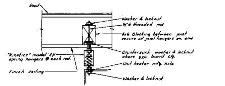
UNIT HEATER MTG. DETAIL No Scale
