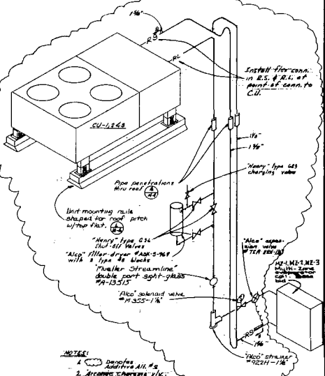
CU-1213 REFRIGERANT PIPING DIAGRAM No scale
