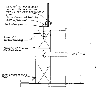
CU-4 MOUNTING DETAIL No scale
