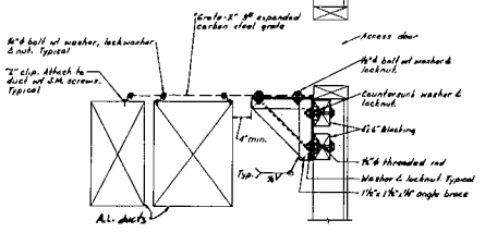
GRATE SUPPORT @ MECH. RM No Scale
