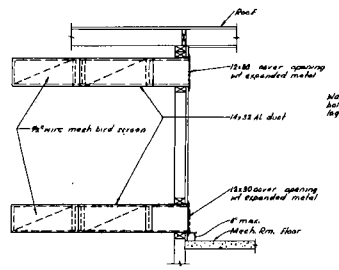
SECTION @ COMBUSTION AIR OPEN'GS Scale 1/4" = 1'-0"
