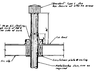
TYPICAL FLUE THRU ROOF DETAIL No Scale
