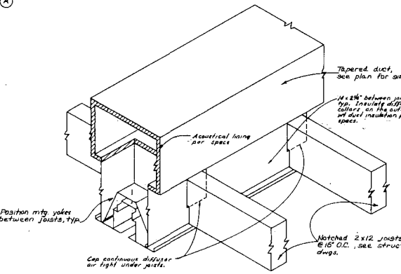
LINEAR DIFFUSER MOUNTING DETAIL No scale
