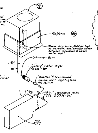
CU-4 REFRIGERANT PIPING DIAGRAM No scale
