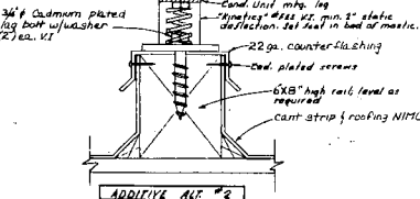
CU-1213 MOUNTING DETAIL No scale
