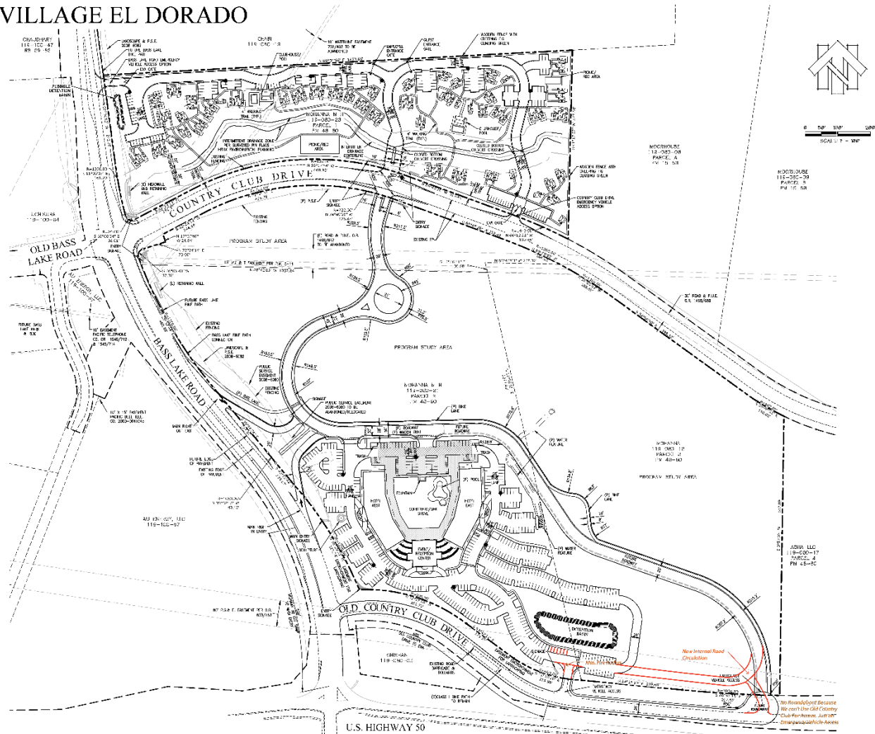
Figure 2. Preliminary Project-Development area site plan
