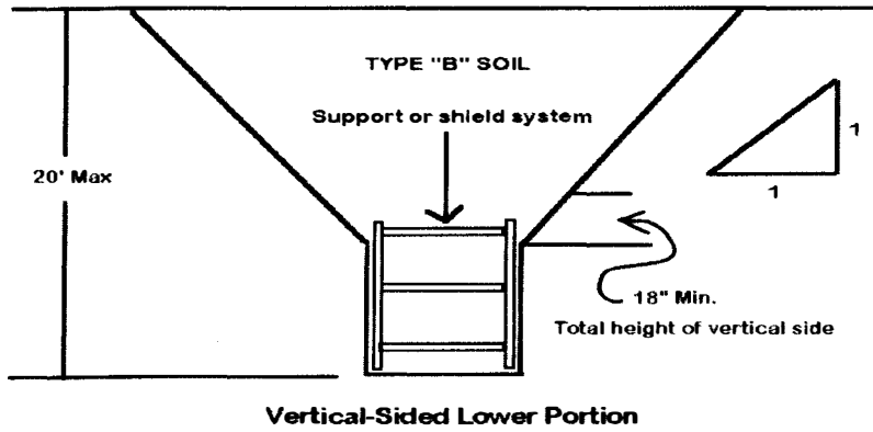
Figure 4: Illustrations of shielding systems in B and C type soils
