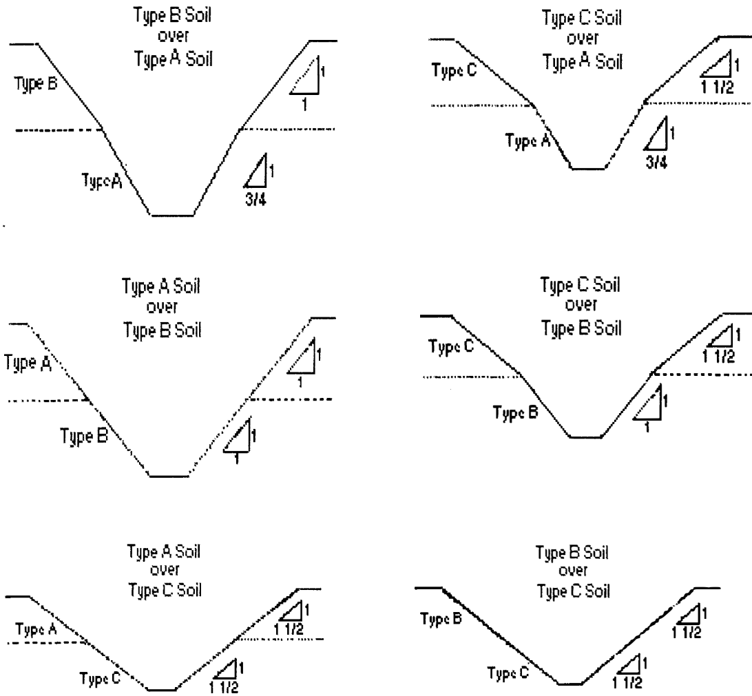
Figure 2: Illustrations of slope configurations in layered soils
