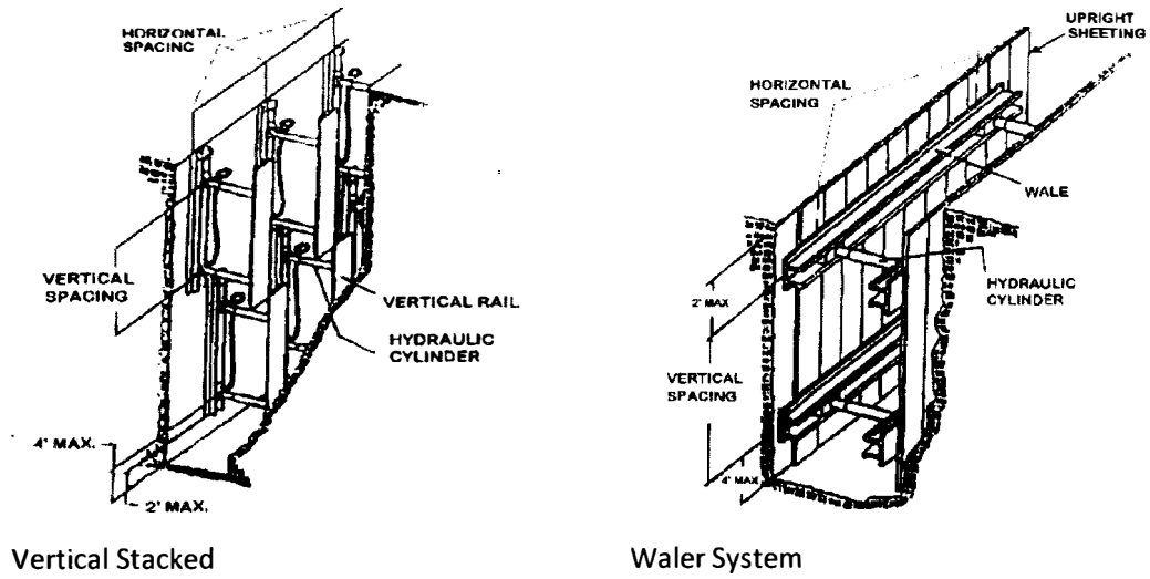
Figure 5: Illustrations of Aluminum hydraulic shoring systems
