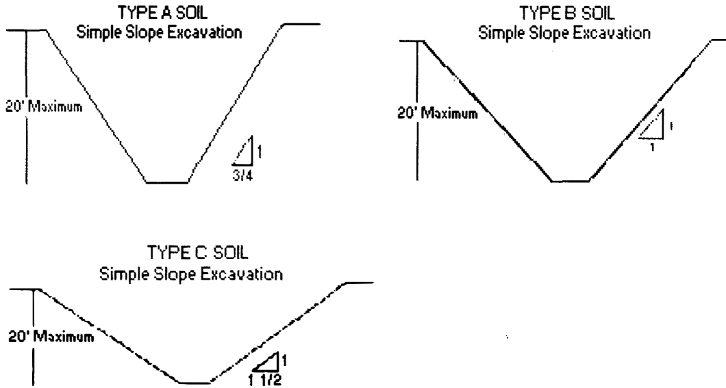
Figure 1: Illustrations of simple slope trenching in A, B and C type soils
