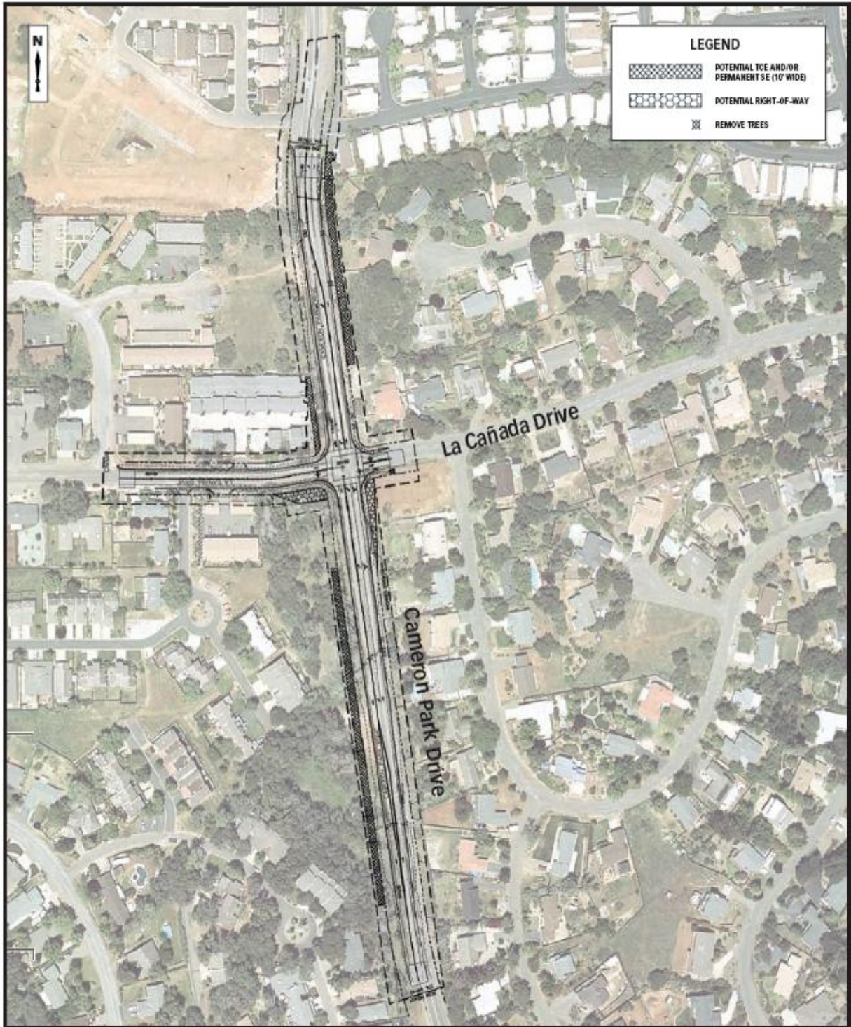
FIGURE 2 Proposed Project Cameron Park Drive / La Cañada Drive Intersection
