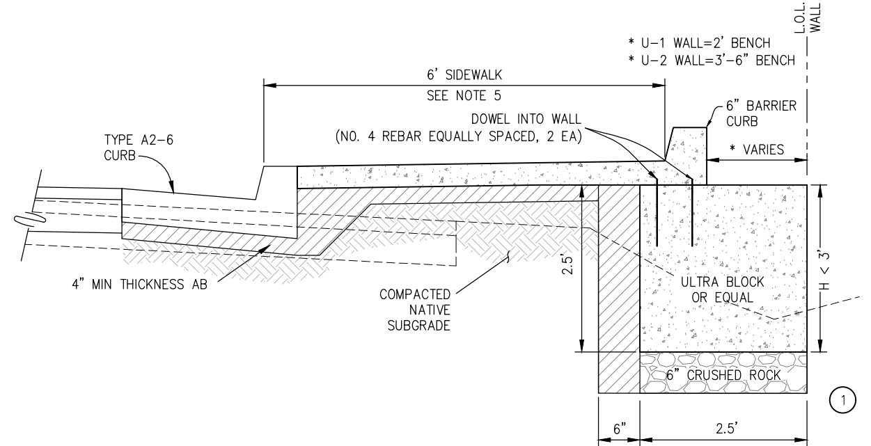
RETAINING WALL BLOCK WALL ALTERNATIVE NTS
