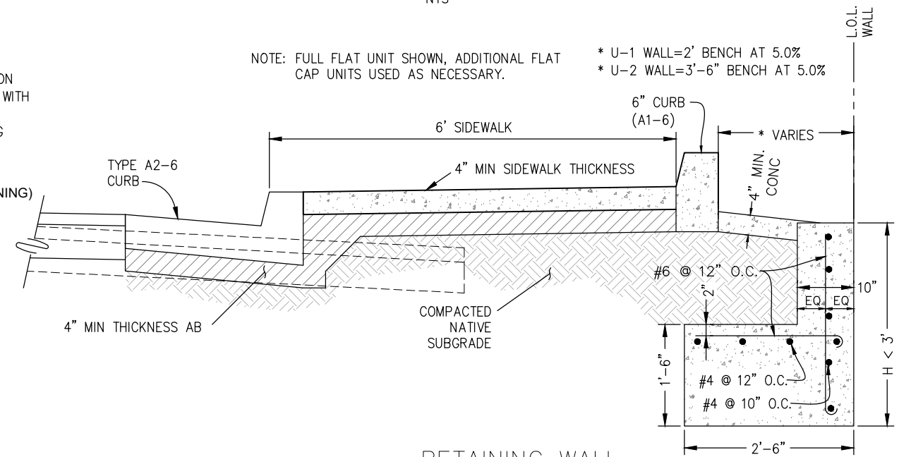
RETAINING WALL MODIFIED TYPE 5 WALL ALTERNATIVE NTS
