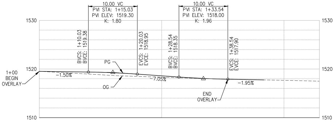
PROFILE — 'MS-2' SCALE: 1"=5' H,V
