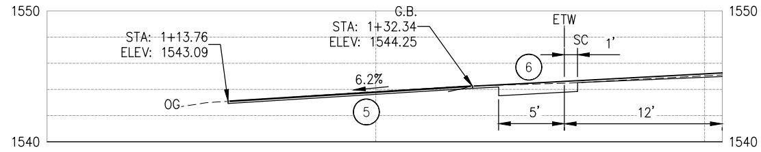
PROFILE FOURSQUARE CHURCH - DRIVEWAY 3838 PONDEROSA RD. APN:070-250-006 NTS
