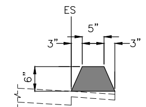
TYPE A ASPHALT DIKE NTS NOTE: VARIOUS DRIVEWAYS ON RIGHT SIDE
