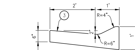
TYPE E CURB NTS NOTE: VARIOUS DRIVEWAYS ON RIGHT SIDE
