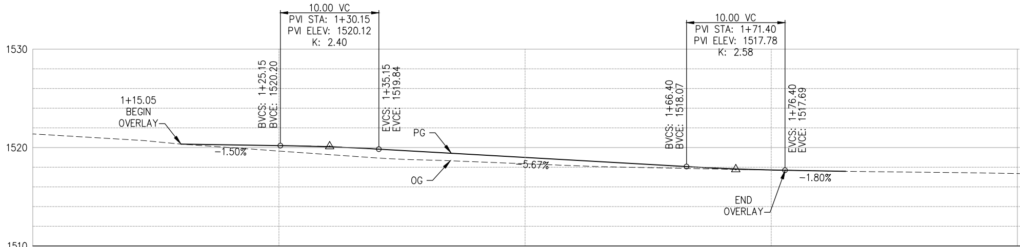
PROFILE — 'MS-1' SCALE: 1"=5' H,V
