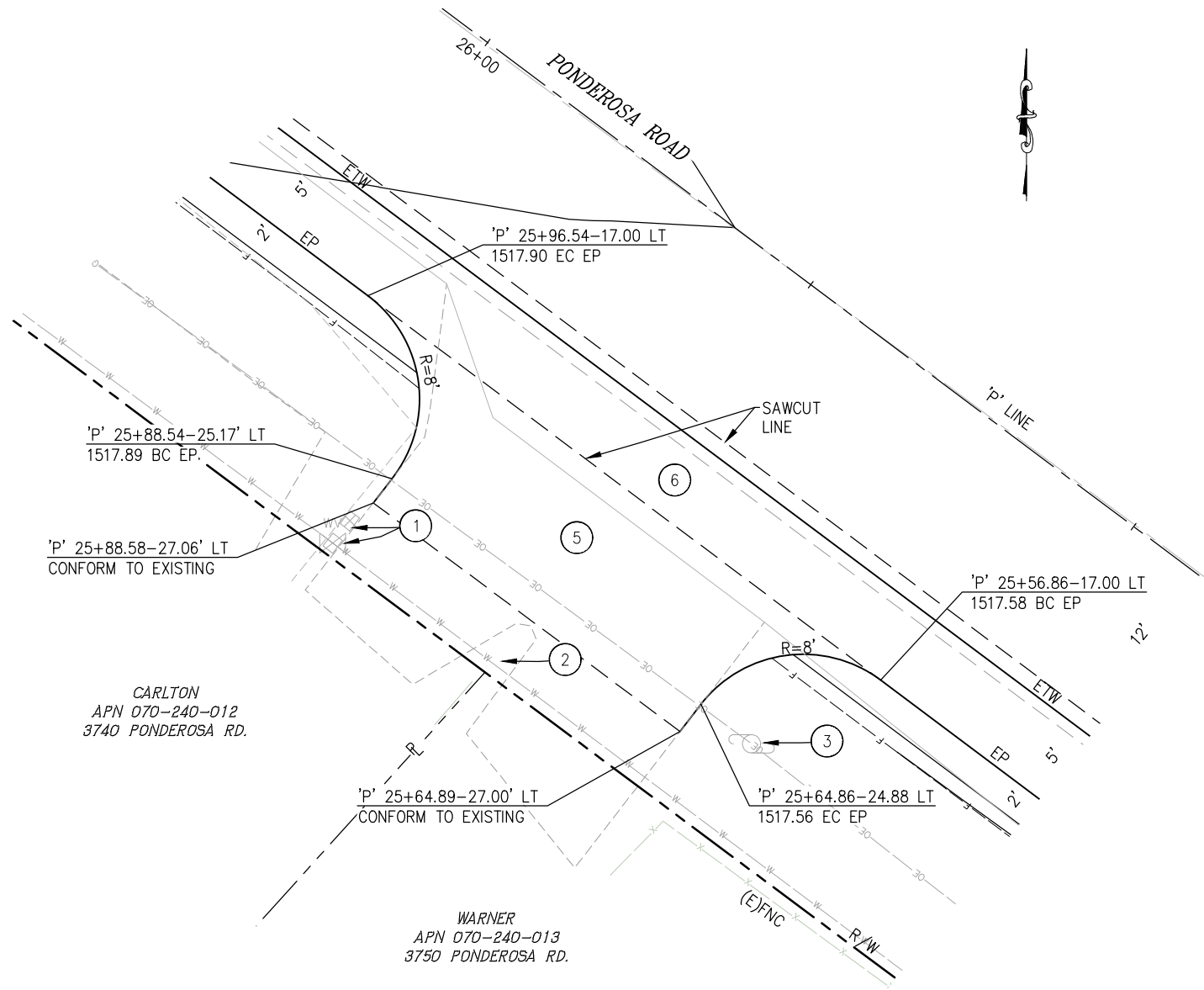
1 PLAN DRIVEWAYS AT 3740 & 3750 PONDEROSA RD. APN: 070-240-012 & 013 SCALE: 1"=5'
