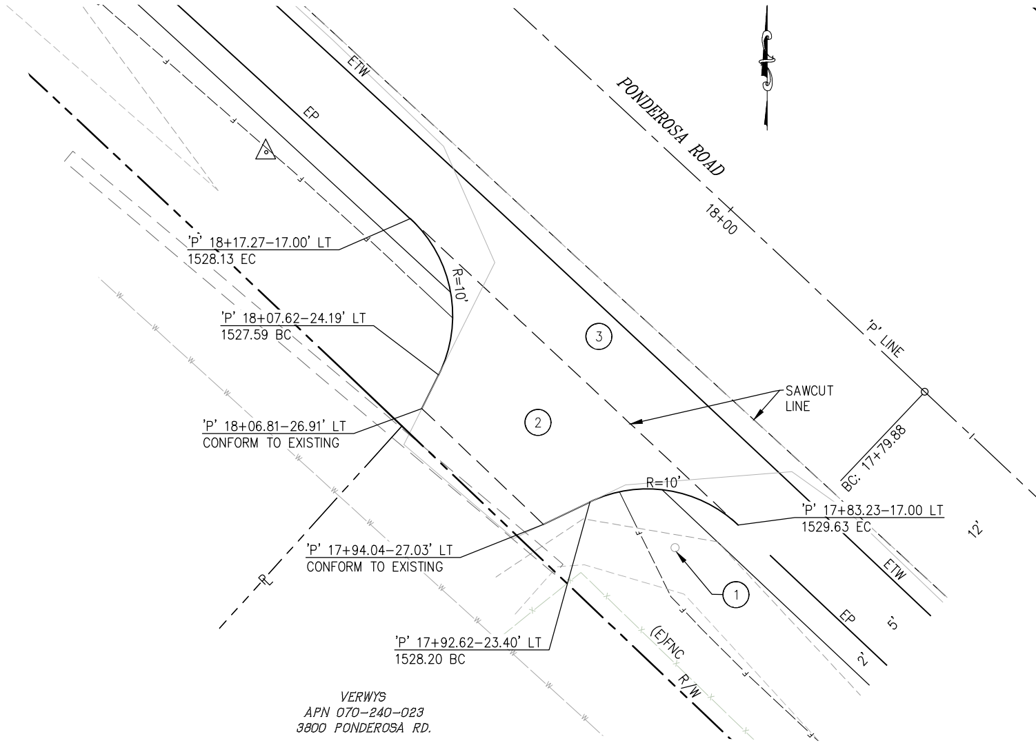
1 PLAN DRIVEWAY AT 3800 PONDEROSA RD. APN: 070-240-023 SCALE: 1"=5'
