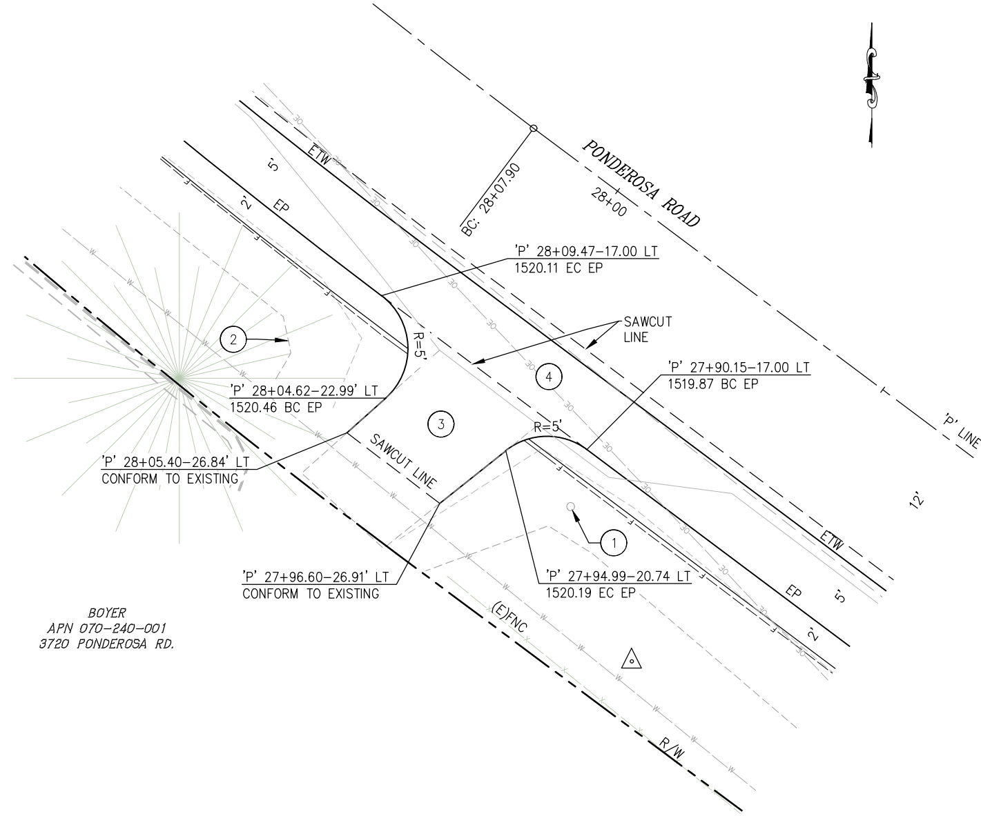
1 PLAN DRIVEWAY AT 3720 PONDEROSA RD. APN: 070-240-001 SCALE: 1"=5'
