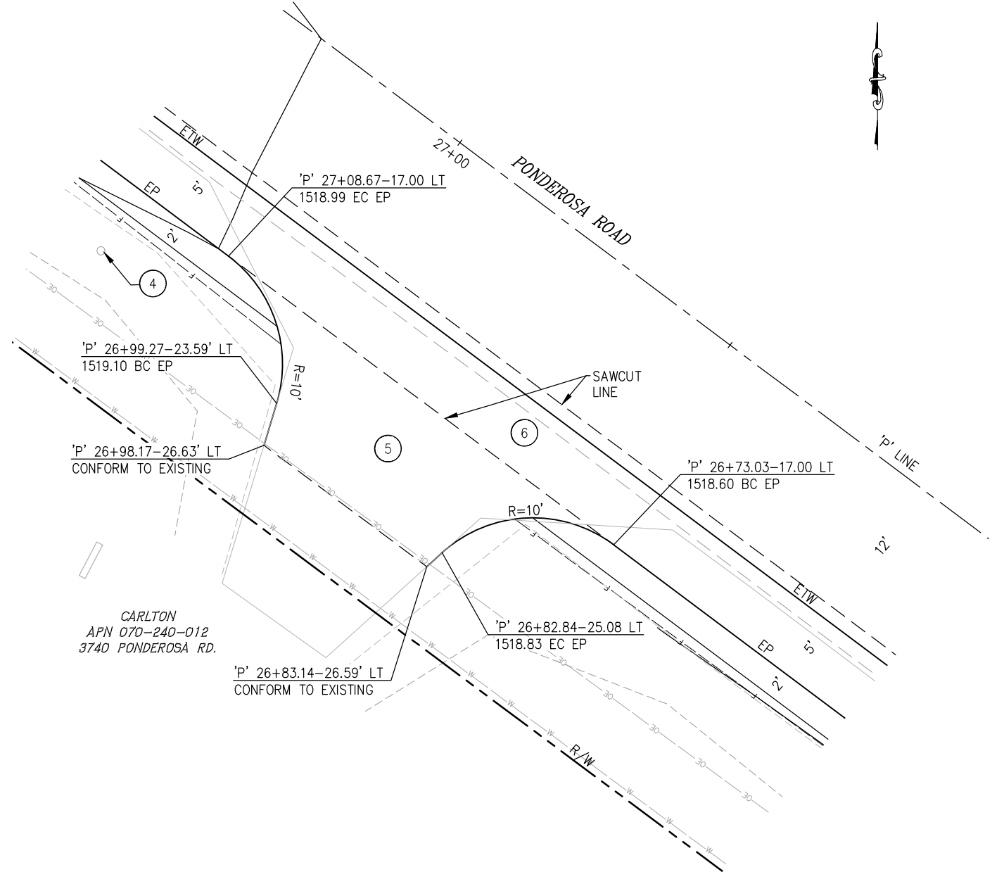
2 PLAN DRIVEWAY AT 3740 PONDEROSA RD. APN: 070-240-012 SCALE: 1"=5'
