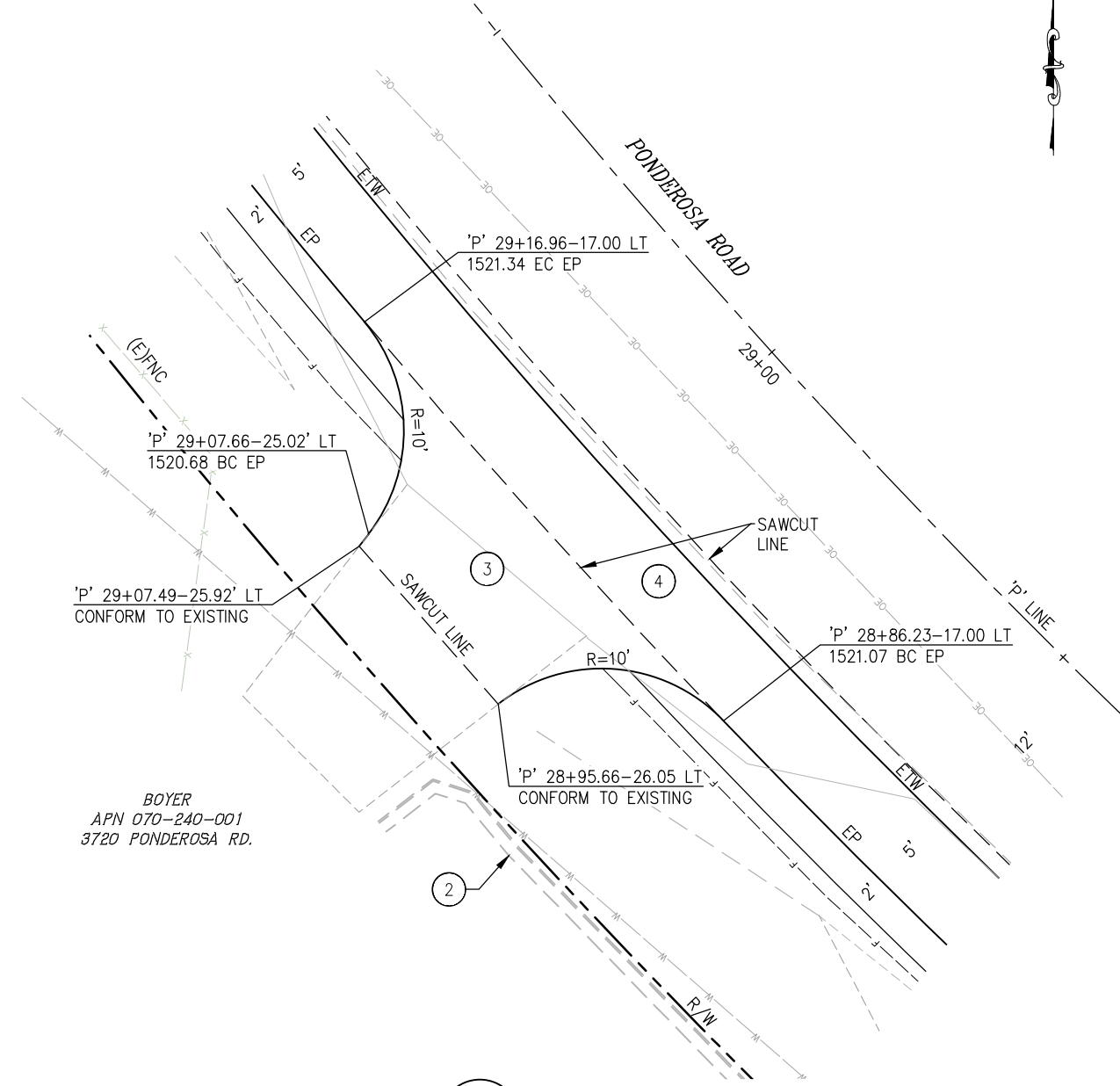
2 PLAN DRIVEWAY AT 3720 PONDEROSA RD. APN: 070-240-001 SCALE: 1"=5'
