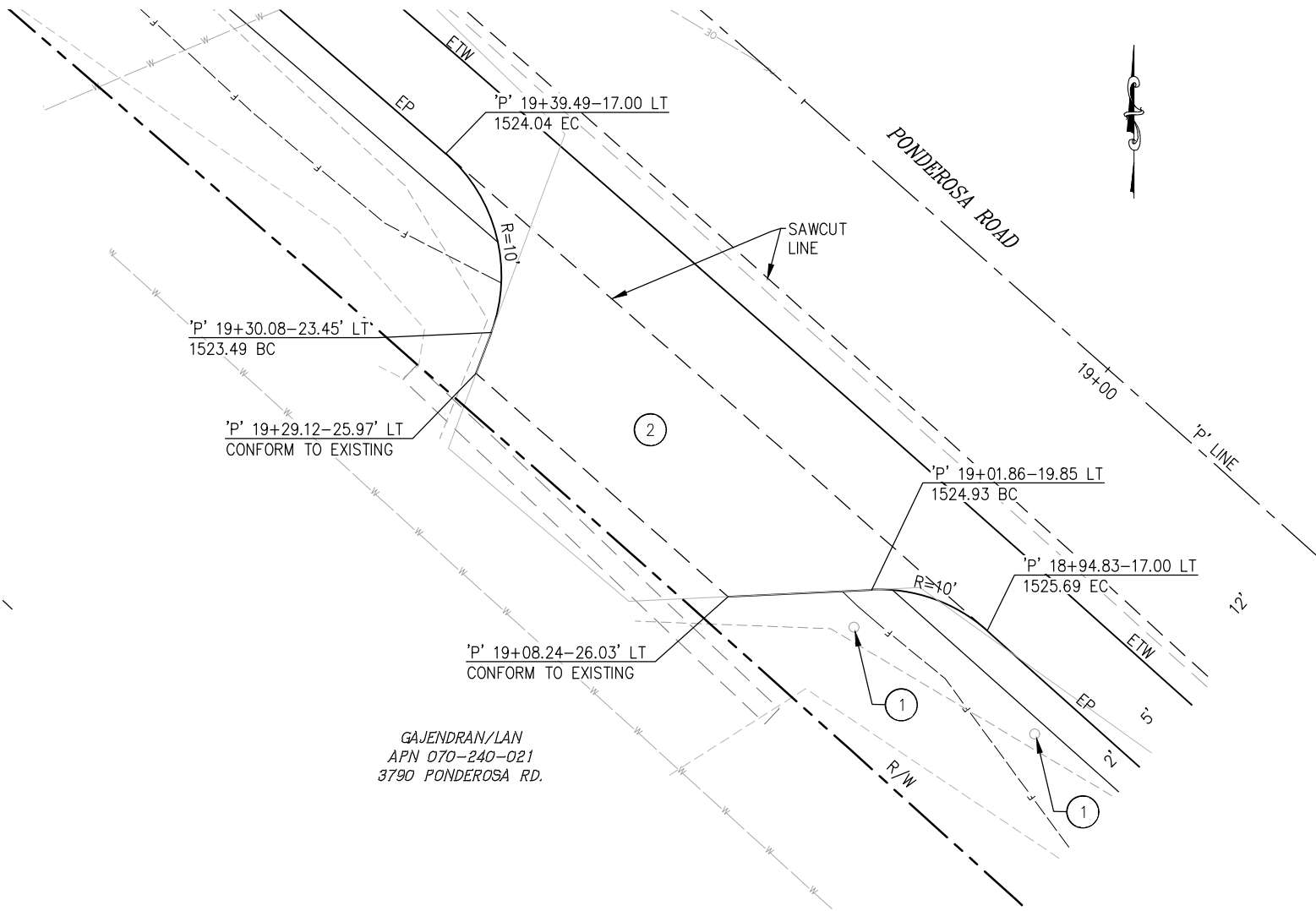
2 PLAN DRIVEWAY AT 3790 PONDEROSA RD. APN: 070-240-021 SCALE: 1"=5'
