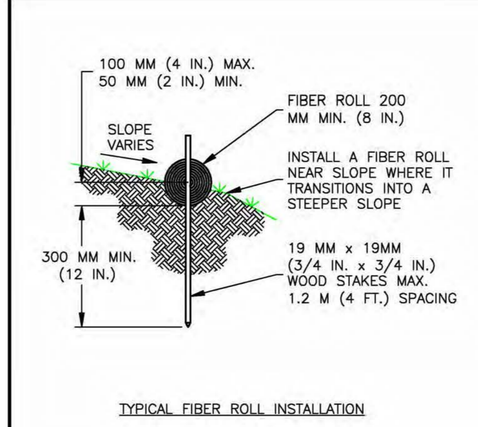
ER-2 TYPICAL FIBER ROLL INSTALLATION FIBER ROLLS NO SCALE
