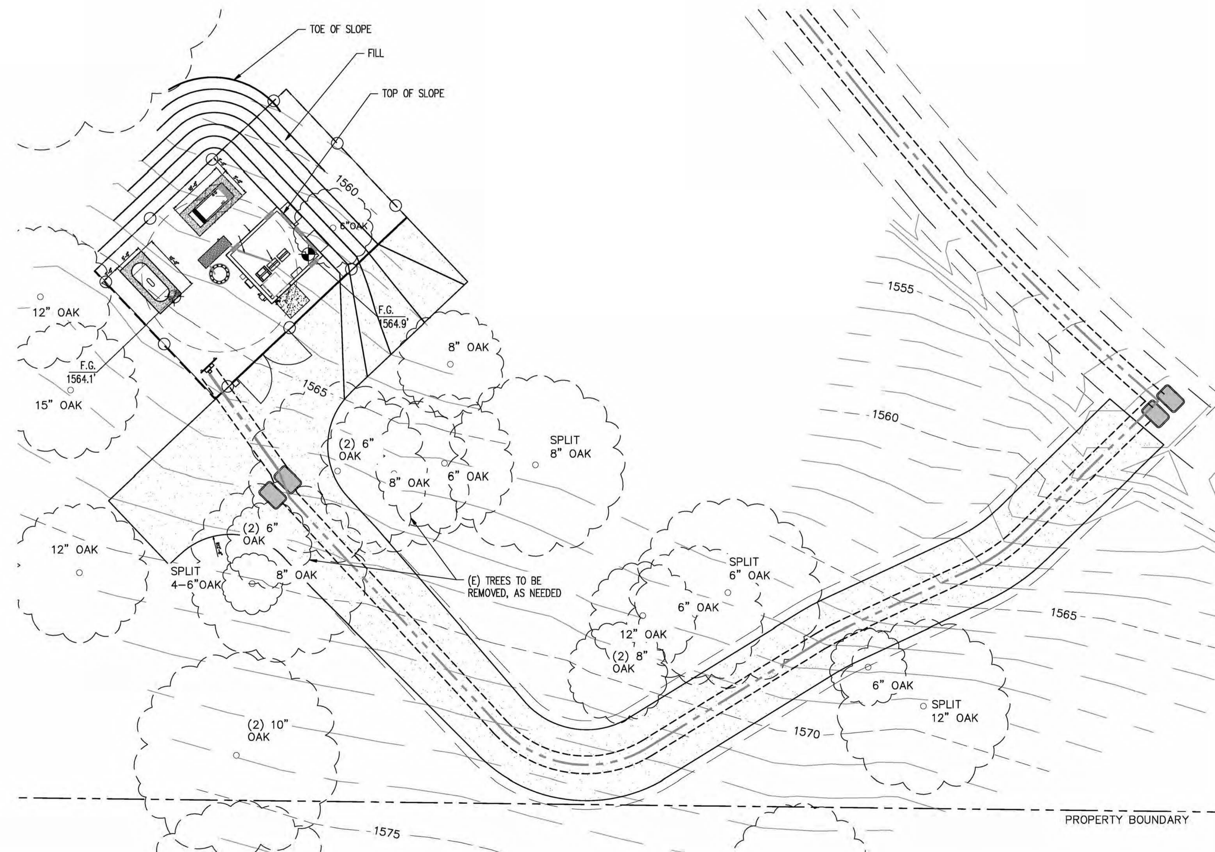
PRELIMINARY GRADING PLAN
