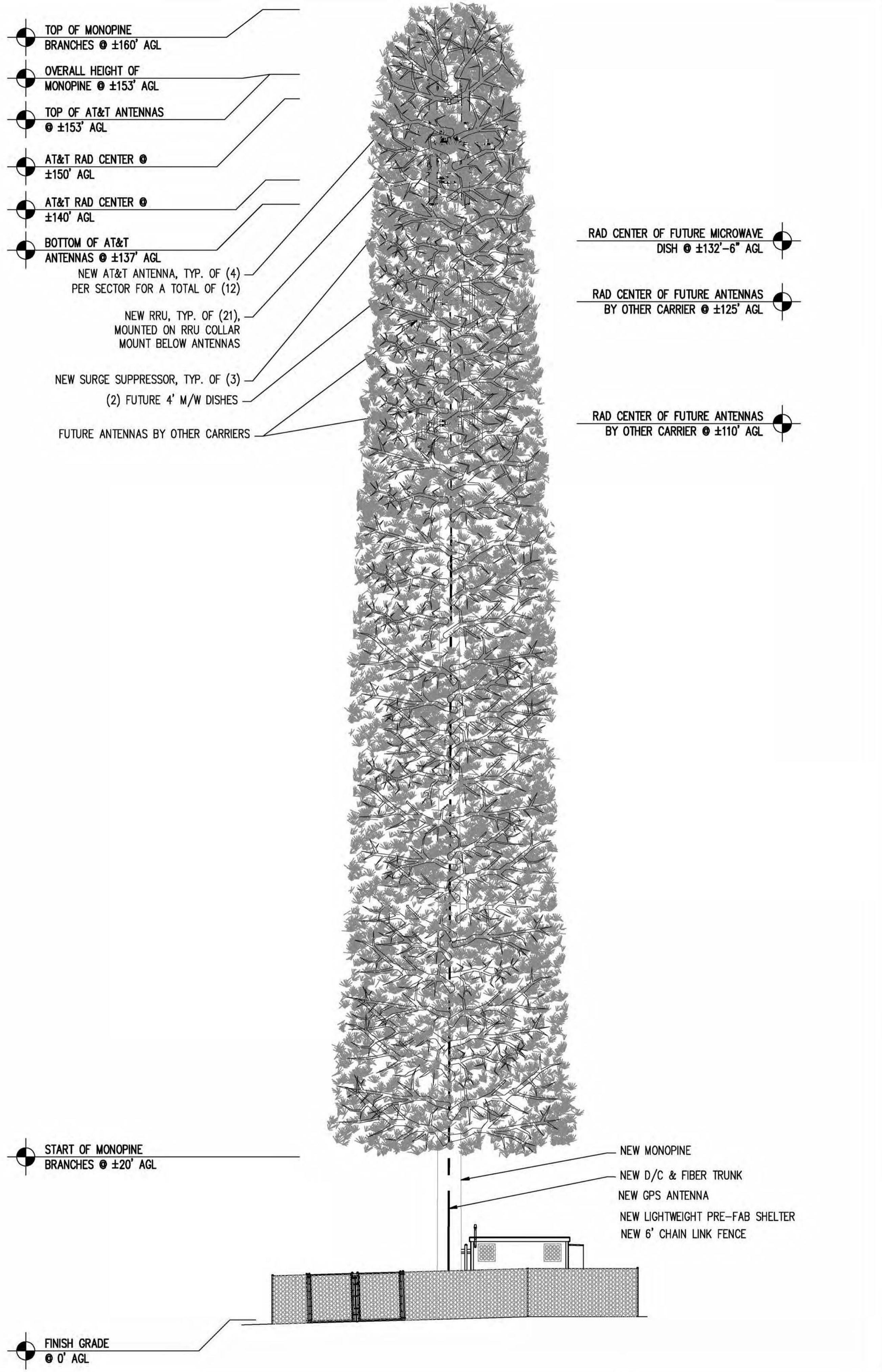
SOUTH ELEVATION
