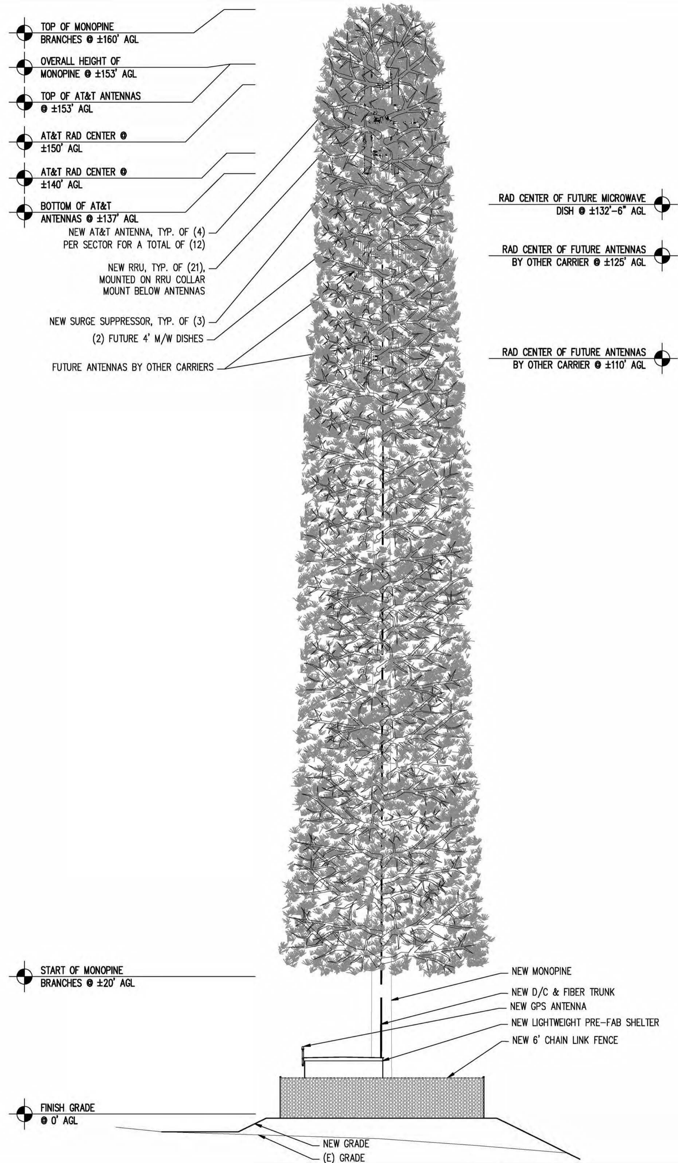
WEST ELEVATION
