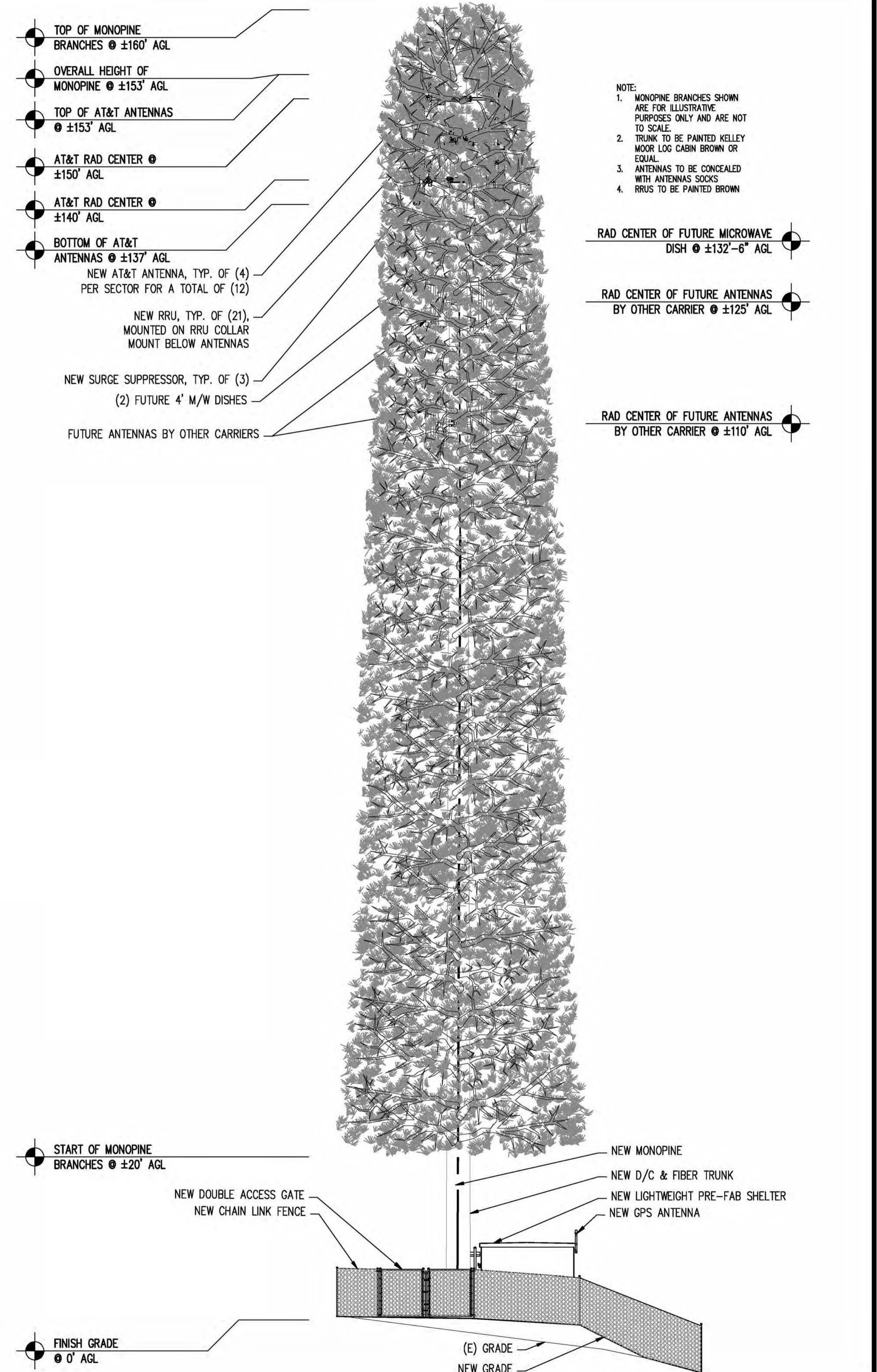
NORTH ELEVATION
