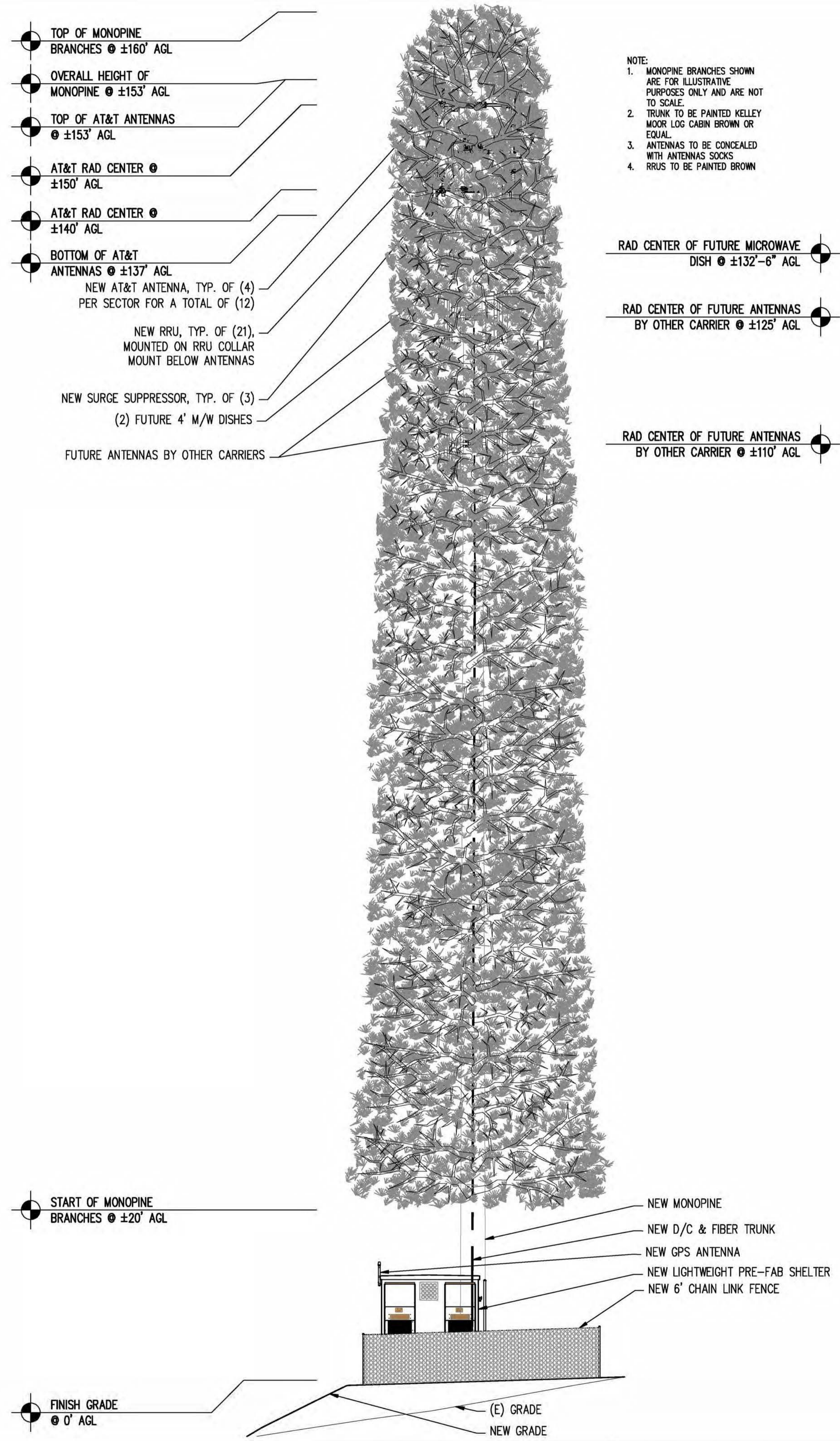
EAST ELEVATION
