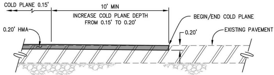
COLD PLANE DETAIL BEGIN/END CONFORMS
