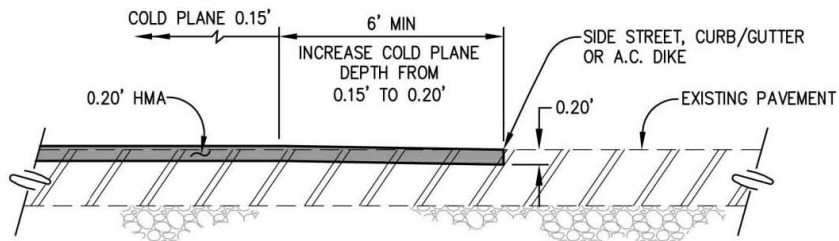
COLD PLANE DETAIL SIDE STREETS, CURB/GUTTER OR A.C. DIKE
