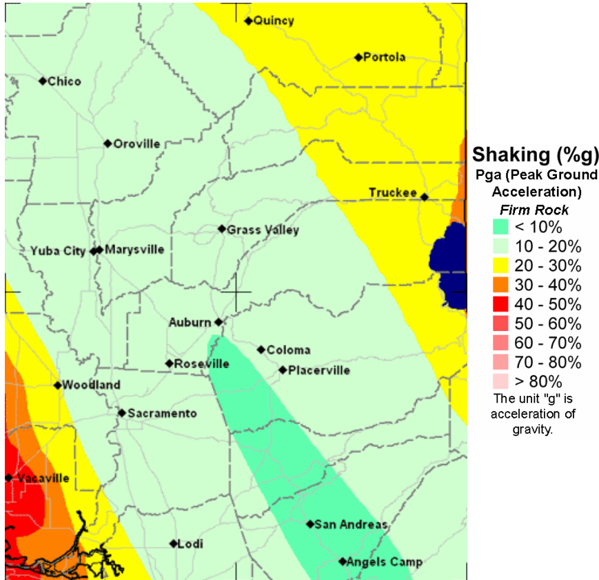
Figure 11-9 Peak Acceleration with 10 Percent Probability of Exceedance in 50 Years (EI Dorado County and Vicinity)
