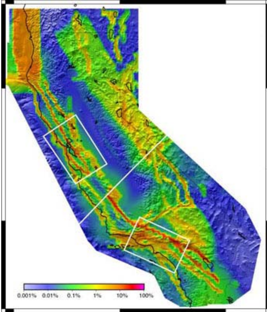
Figure 11-8. Level of Earthquake Hazard (California) 1
