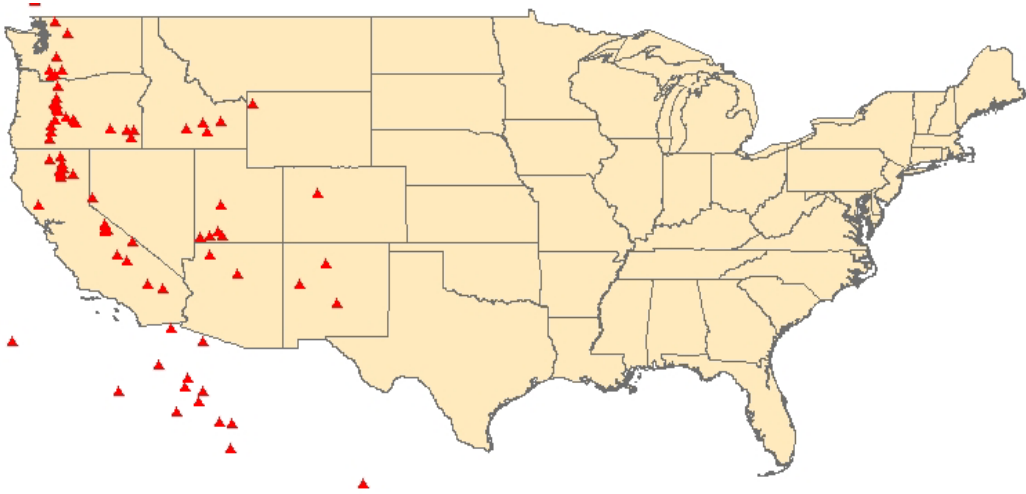
Figure 11-13. Known Volcano Locations in the United States
