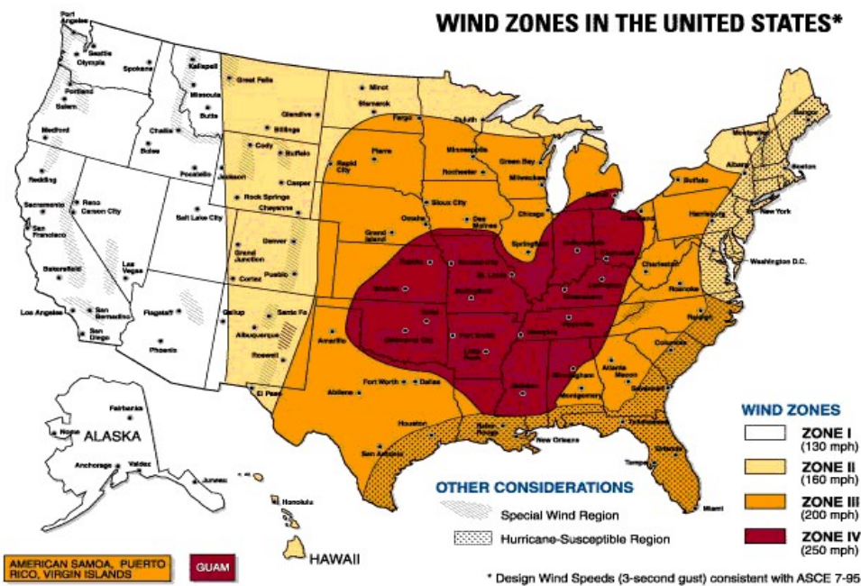
Figure I.2 Wind zones in the United States
