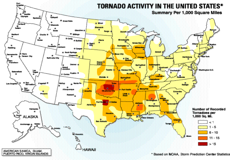
Figure 11-16. Tornado Activity in the United States
