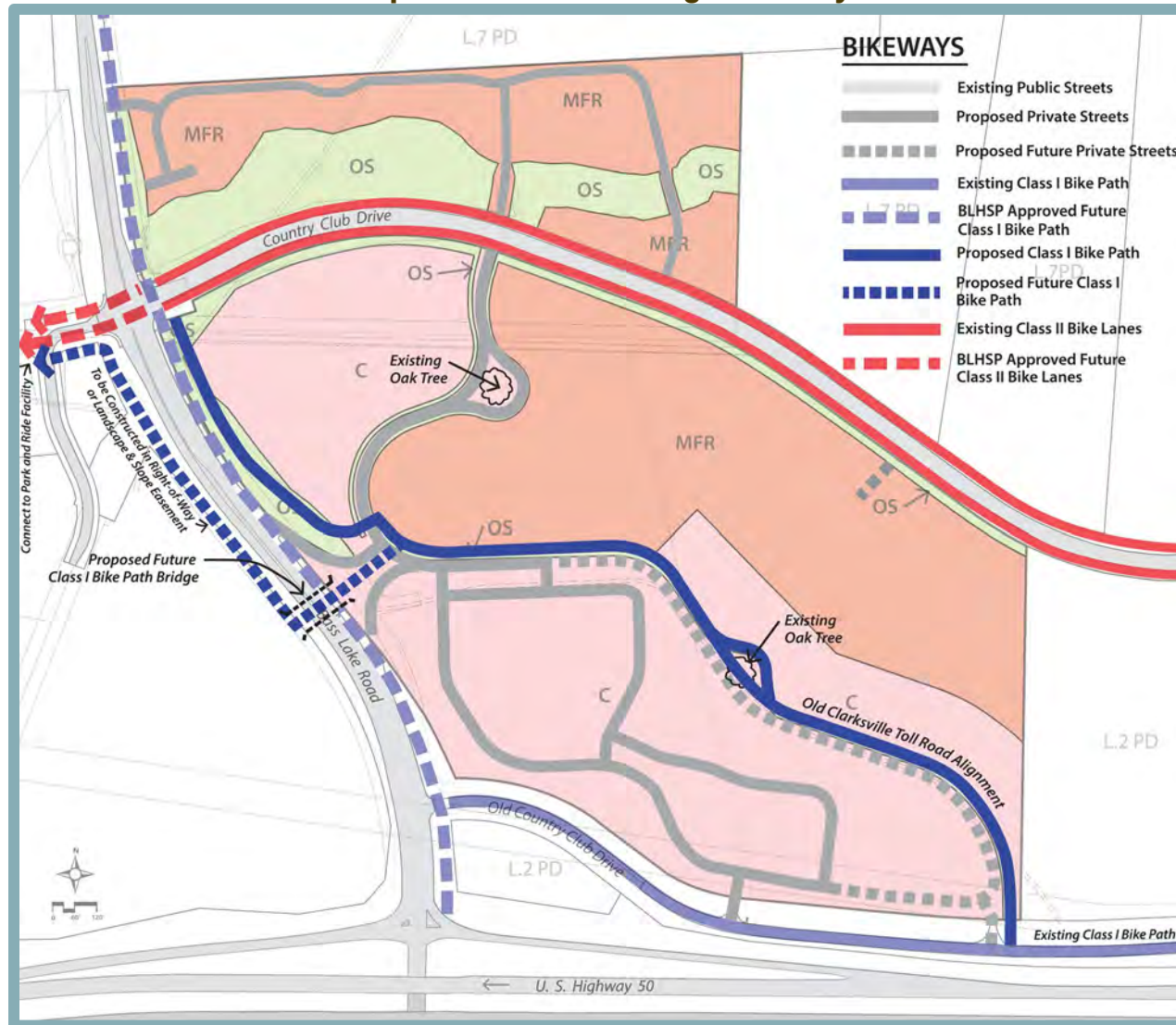
Figure 4.11-2 Proposed and Existing Bikeways
