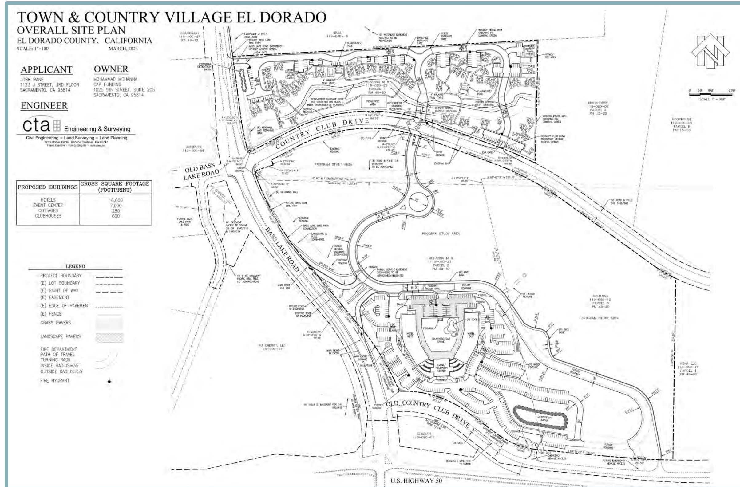
Figure 3-7 Overall Site Plan
