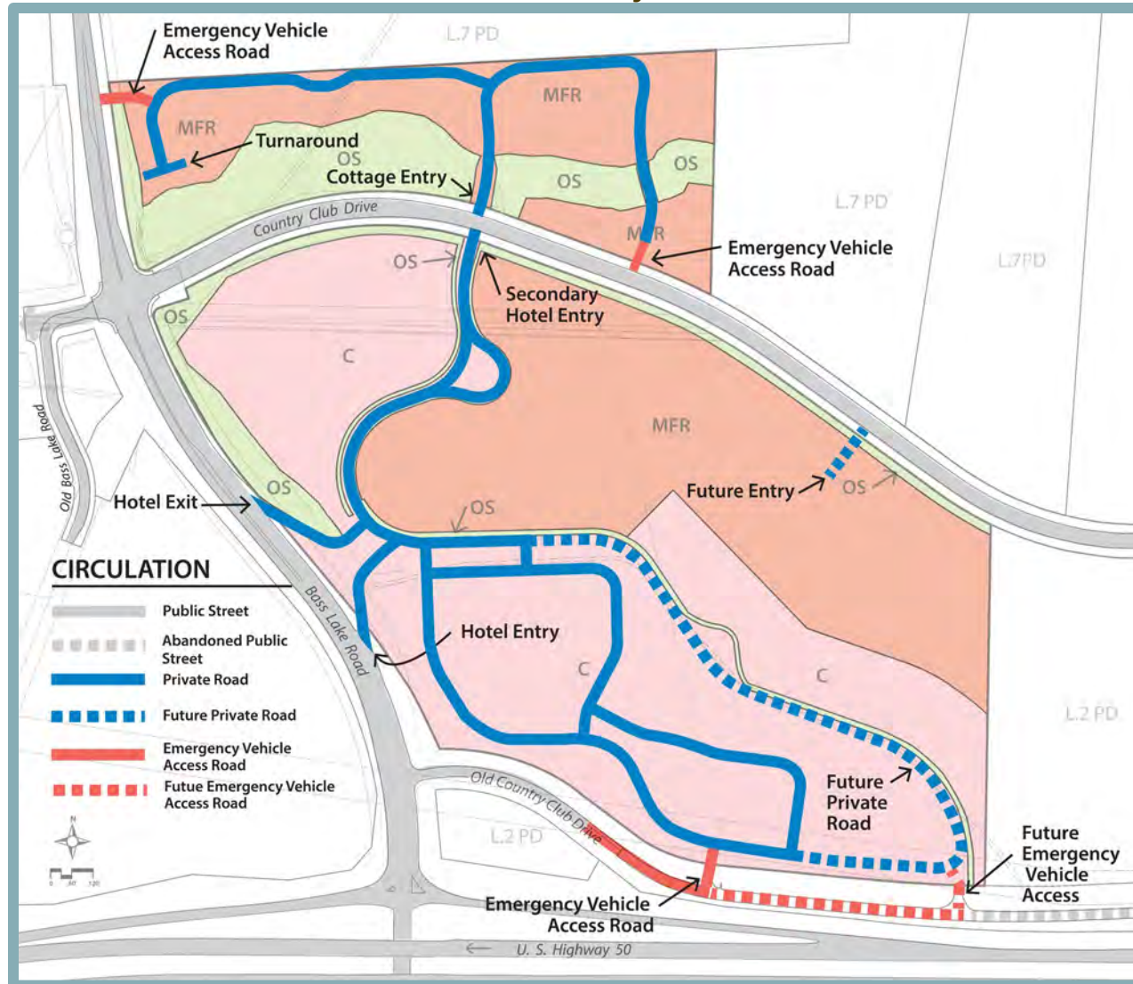
Figure 3-12 Internal Roadway Network
