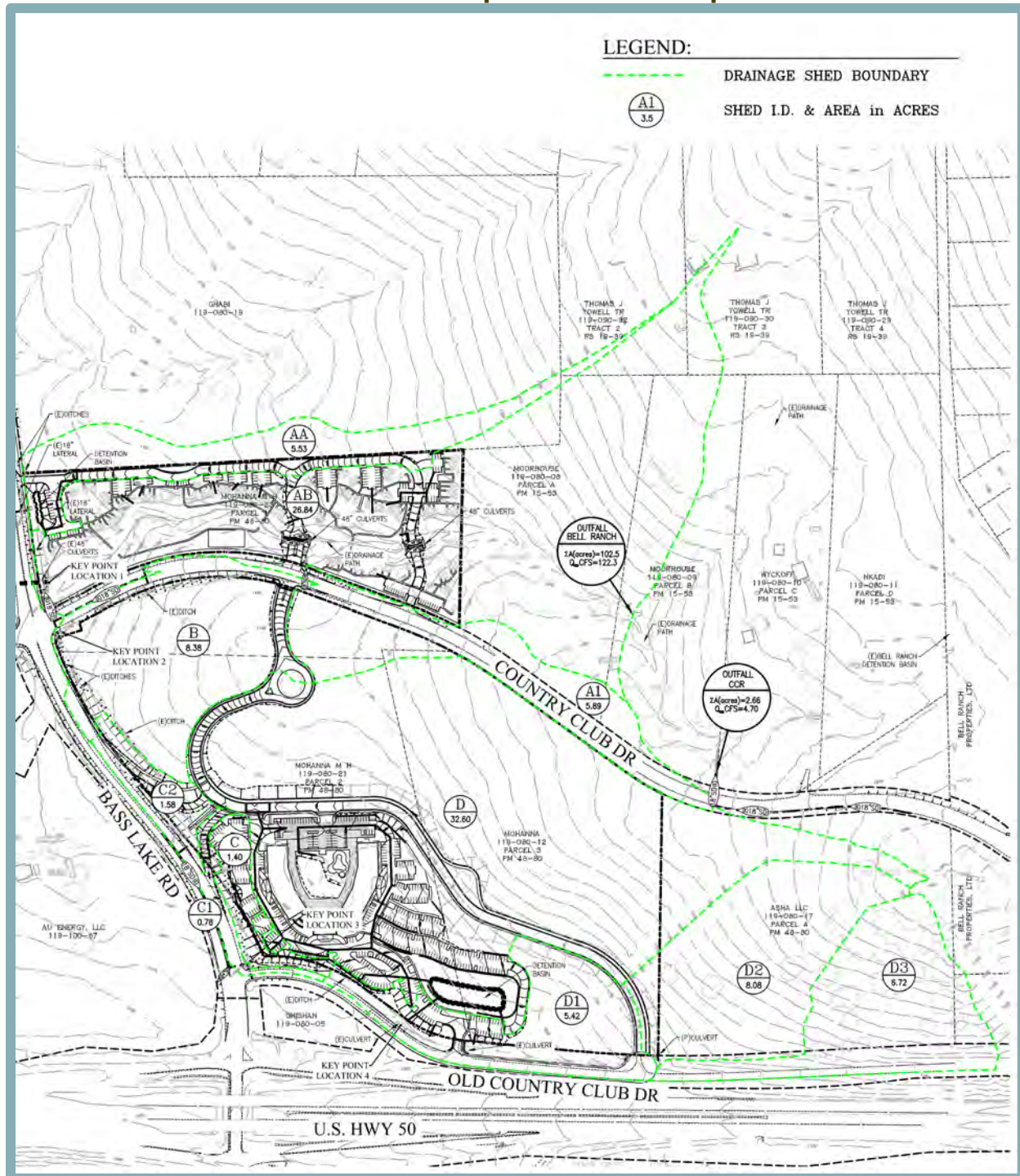
Figure 4.7-4 Post-Development Shed Map
