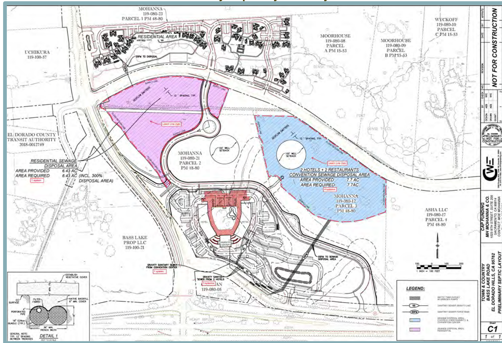
Figure 4.5-3 Preliminary Septic System Layout
