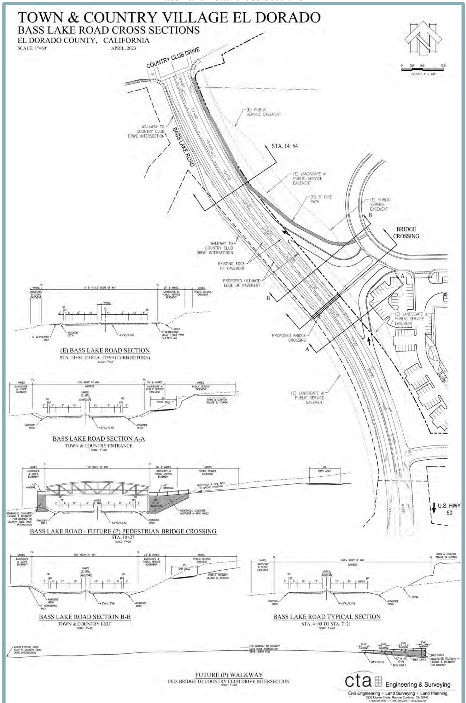
Figure 3-14 Bass Lake Road Cross Sections
