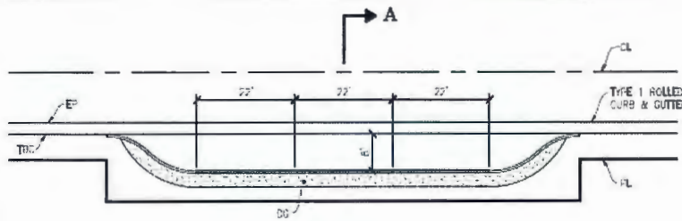
PLAN VIEW SCALE: 1" = 20'
