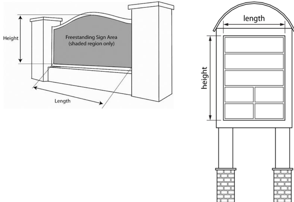
Figure 17.16.070.B Freestanding Sign Area
