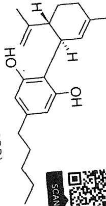
Cannabidiol (CBD) C_{21}H_{30}O_2
