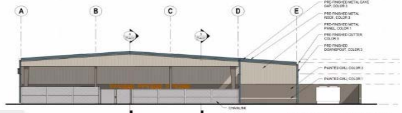
4 EXTERIOR ELEVATION - SOUTH
