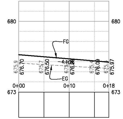
2 BIKE PATH & CURB RAMP CONNECTION DETAIL SCALE: 1" = 5'
