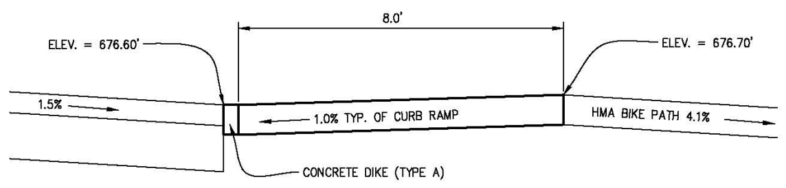
CENTERLINE OF CURB RAMP NO SCALE
