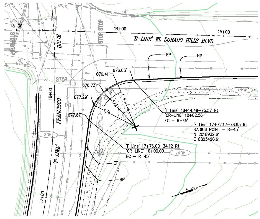
1 CURVE RETURN DETAIL SCALE: 1" = 20'
