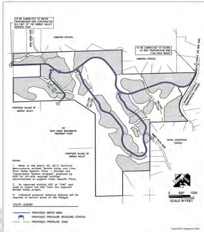
Figure 2-9 Potable Water Plan
