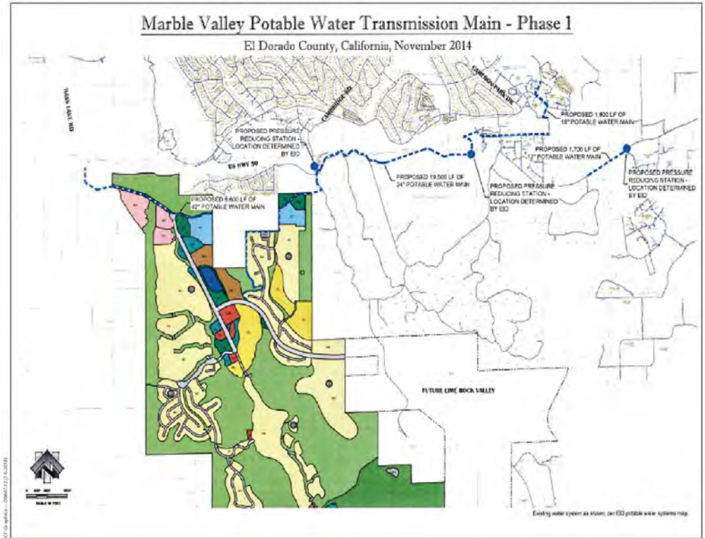
Figure 2-12 Interim Phase I Potable Water Improvements
