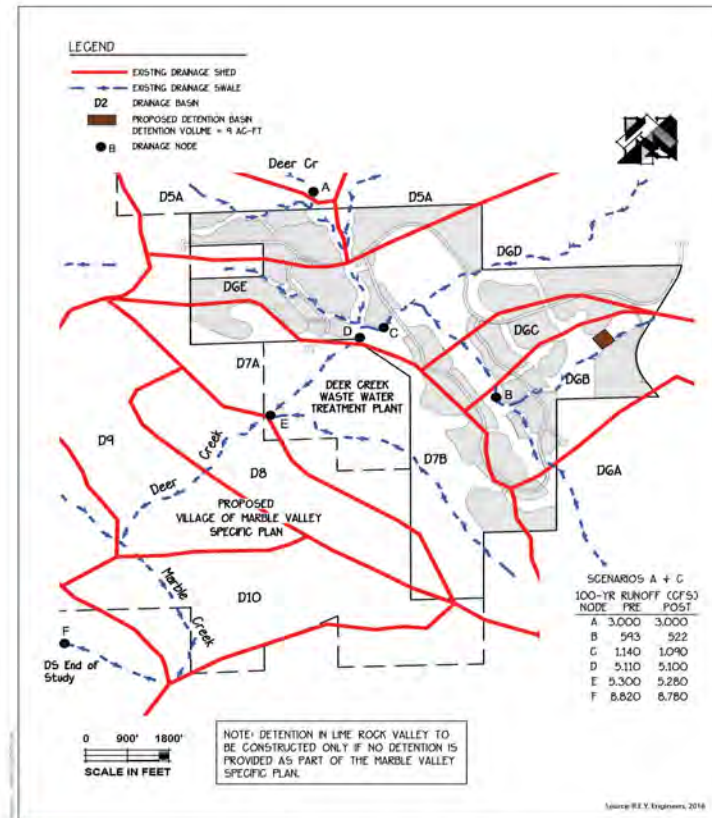
Figure 2-12 Onsite Retention and Detention Plan
