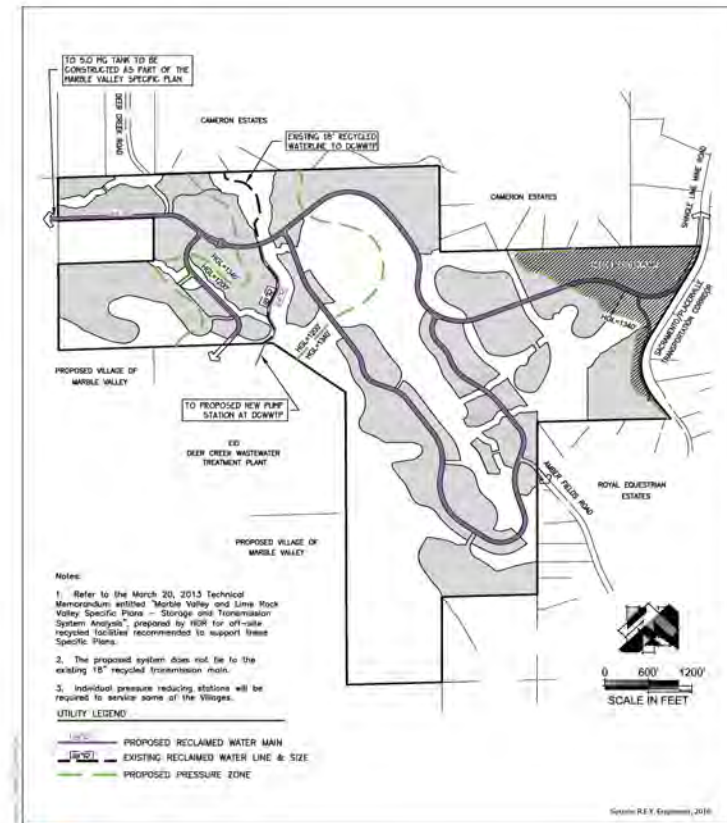
Figure 2-10 Recycled Water Plan
