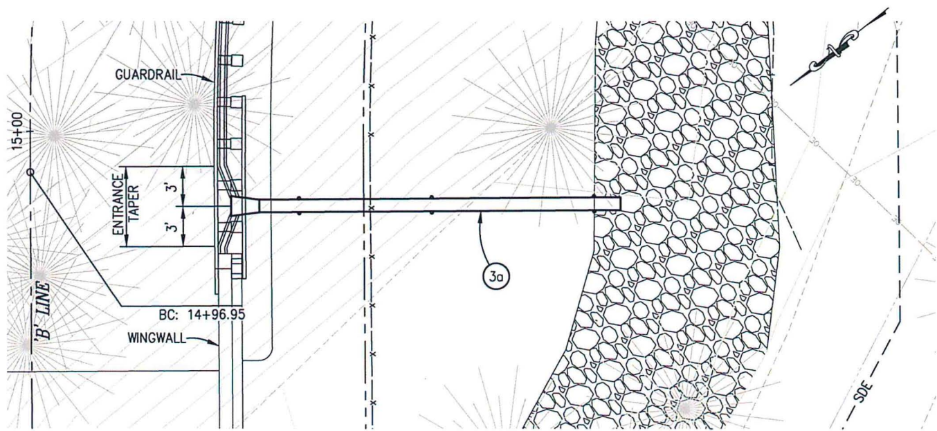
SD SYSTEM 3-PLAN SCALE: 1"=5'
