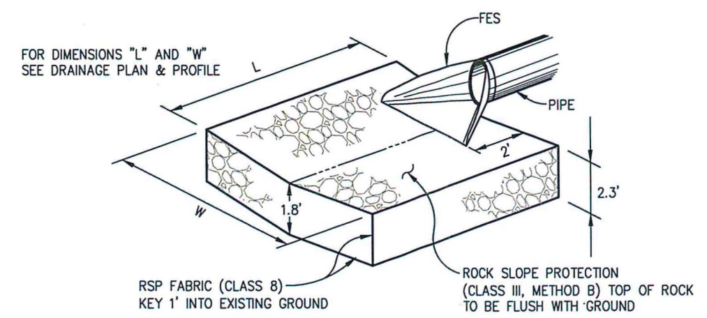
ROCK ENERGY DISSIPATOR NTS
