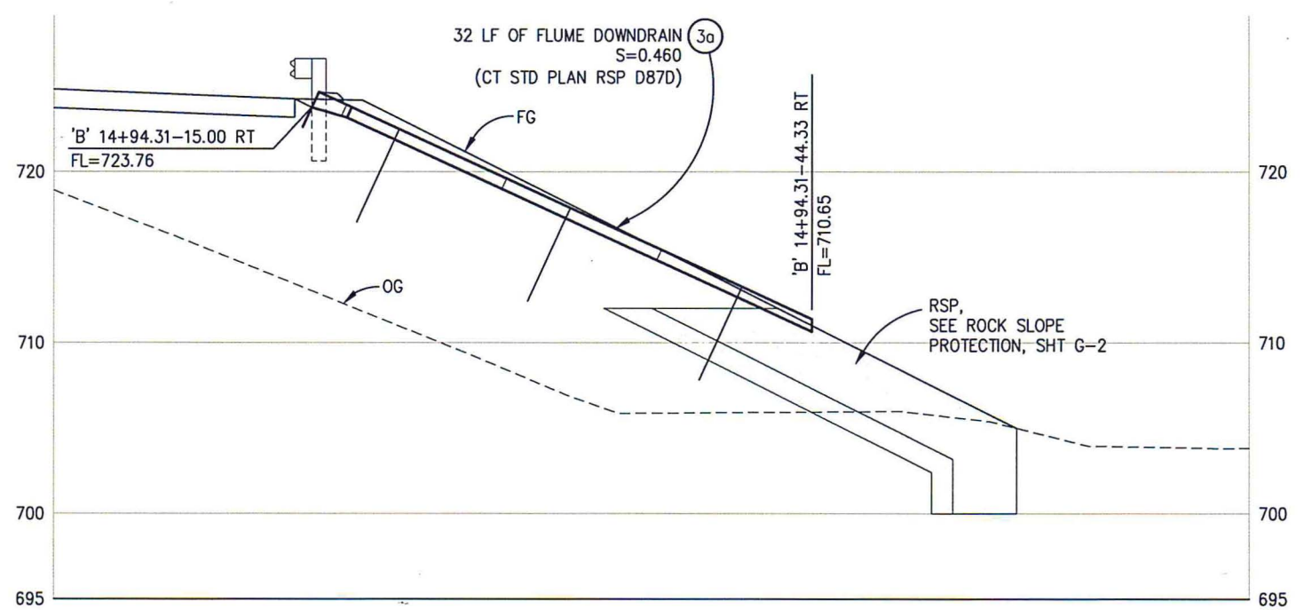
SD SYSTEM 3-PROFILE SCALE: 1"=5' H,V
