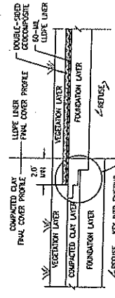
FINAL COVER CONTINUATION/ MATERIAL CHANGE N.T.S.
