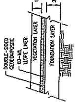
LINEAR LOW DENSITY POLYETHYLENE (LLDPE) LINER FINAL COVER PROFILE 13.8-ACRE AREA N.T.S.
