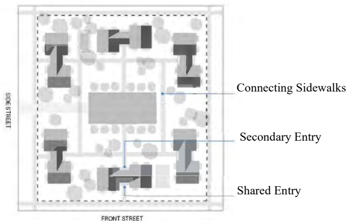
FIGURE 3.2- 57 . SHARED ENTRIES AND SECONDARY ENTRIES
