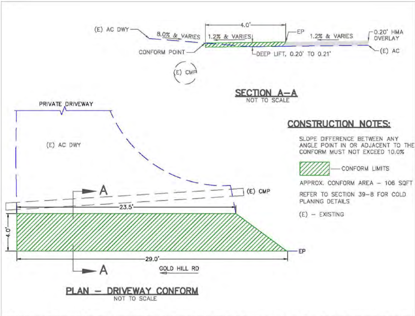
HOT MIX ASPHALT (TYPE A) DRIVEWAY CONFORM DEEP LIFT HMA (6000 GOLD HILL ROAD)
