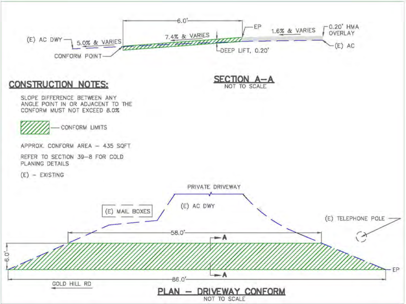
HOT MIX ASPHALT (TYPE A) DRIVEWAY CONFORM DEEP LIFT HMA (SULLIVAN LANE)
