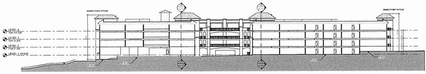
2 Section 5 1" = 20'-0"
