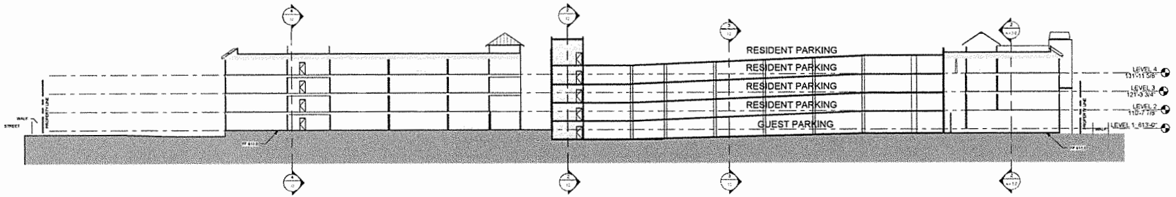
1 Section 1 1" = 20'-0"
