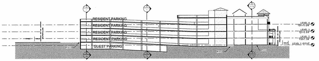
3 Section 3 1" = 20'-0"
