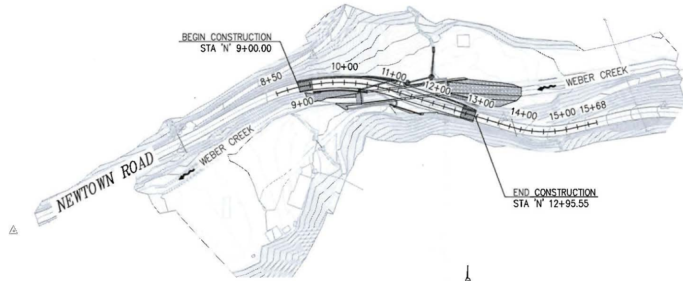
SITE PLAN SCALE: 1"=100'
