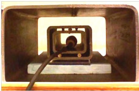
Fig. 1. The three layers of magnetic shielding. The Narda EFA-300’s MF probe is in place of the culture vessel. MF coils for exposure are below, but not in contact with the two smaller shields, insulated from the outer shield by a layer of rigid foam.
