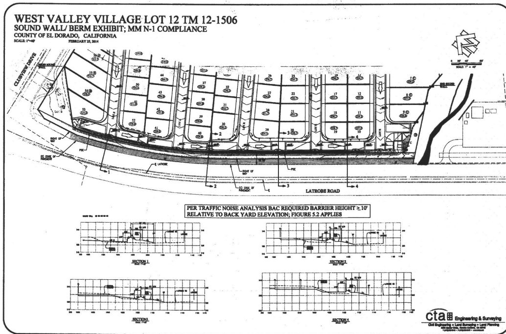
Figure 7: Noise Mitigation for Tentative Map TM 12-1506 (Lot W) 1506
