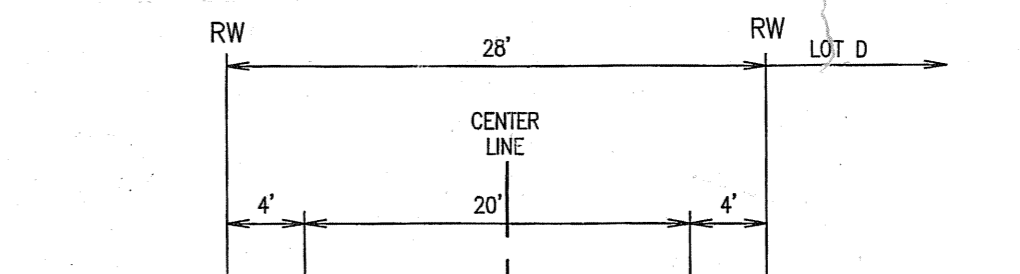
TYPICAL ROAD SECTION A CIRCLE** SCALE: 1"=10'
