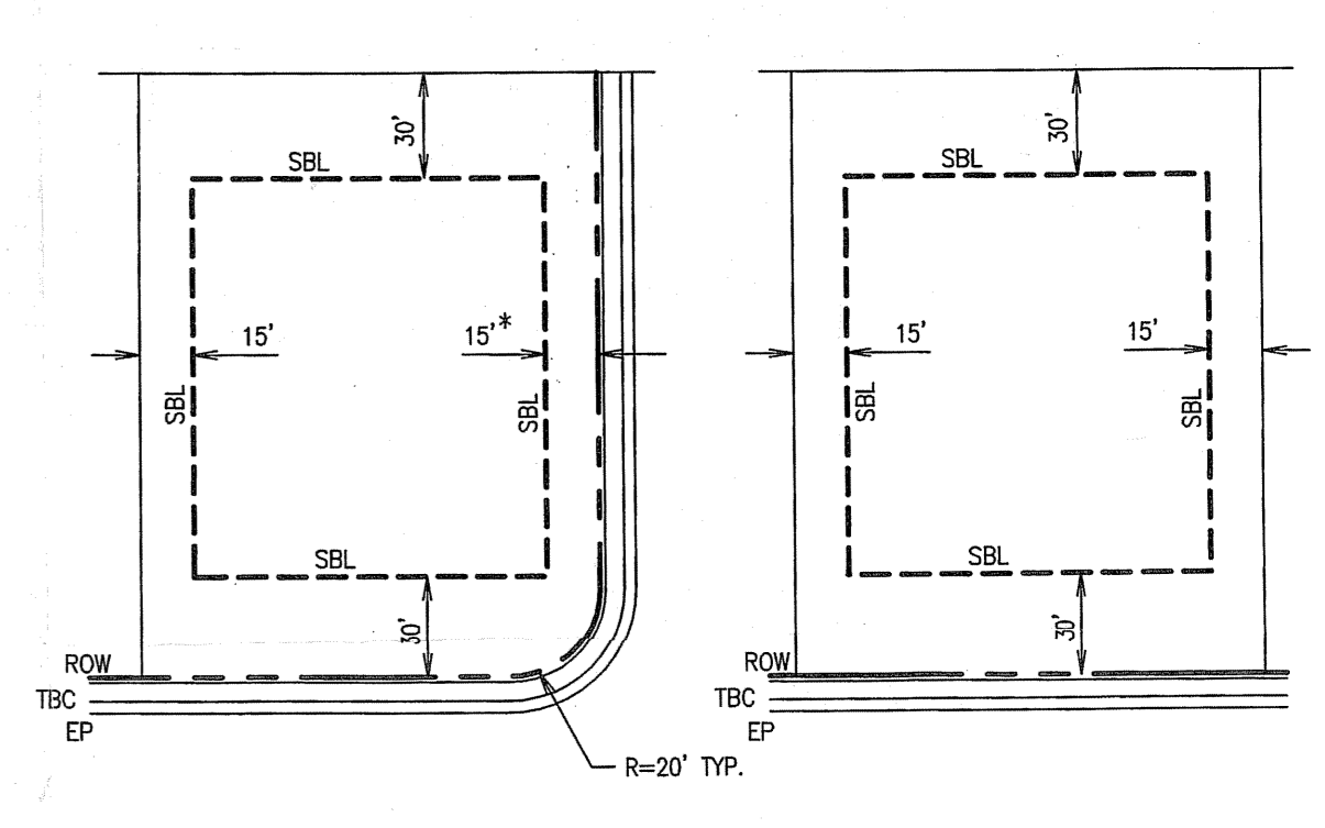
TYP. BUILDING SETBACKS RE5-PD NOT TO SCALE UNLESS OTHERWISE SHOWN
