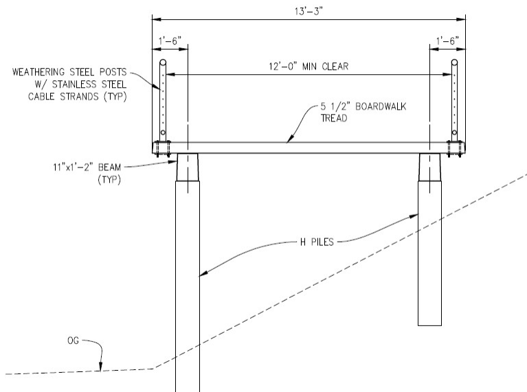
LOTUS ROAD CLASS I MULTI-USE TRAIL IMPROVEMENTS NOT TO SCALE
