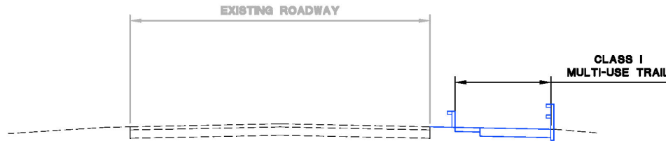
LOTUS ROAD CLASS I MULTI-USE TRAIL IMPROVEMENTS NOT TO SCALE
