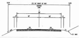
TYPICAL ROAD SECTION W/ 36' ROADWAY * SCALE: 1" = 40'
