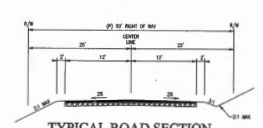
TYPICAL ROAD SECTION SCALE: 1" = 40'
