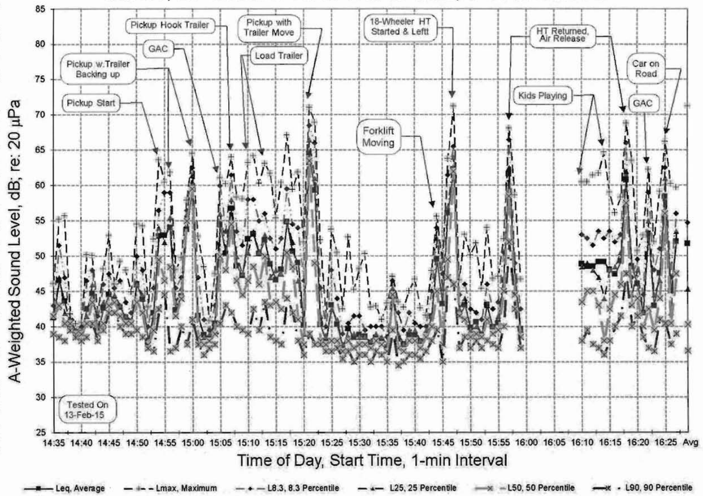
Figure 6. Sound Metrics Measured in 1-minute Intervals at Position #1 During Normal Tunnel Electric Activity.
