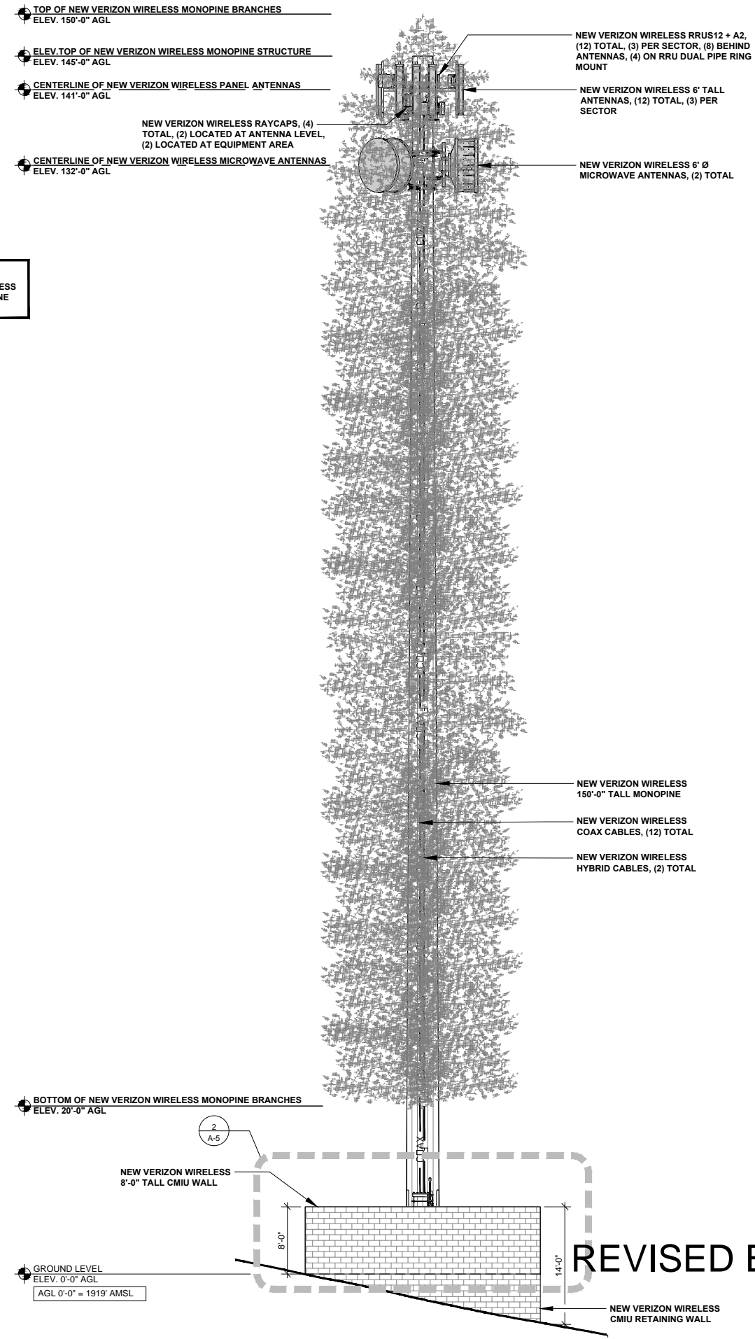
EAST ELEVATION
