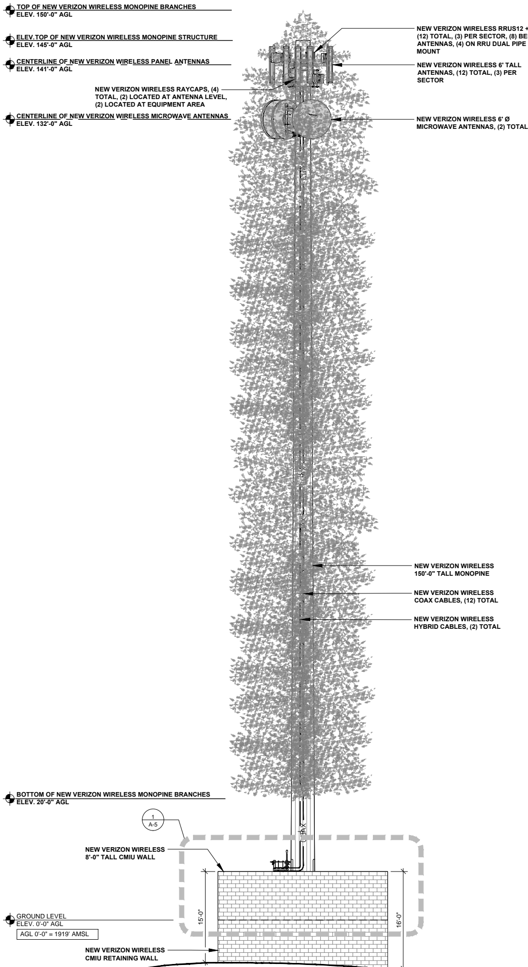
NORTH ELEVATION
