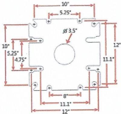
Industry standard bolt pattern and pedestal base dimensions
