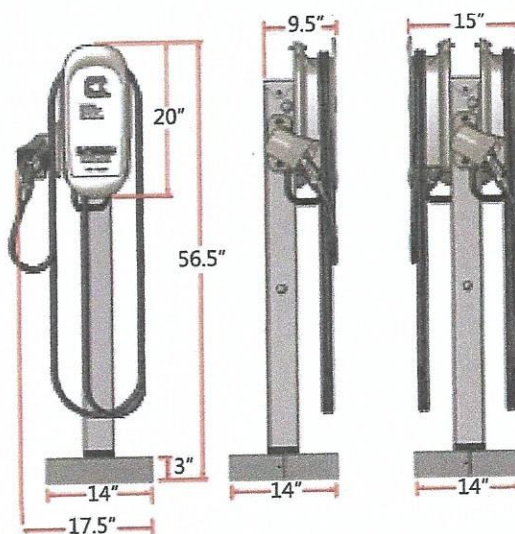
HCS Pedestal Dimensions for single and dual mounted installations
