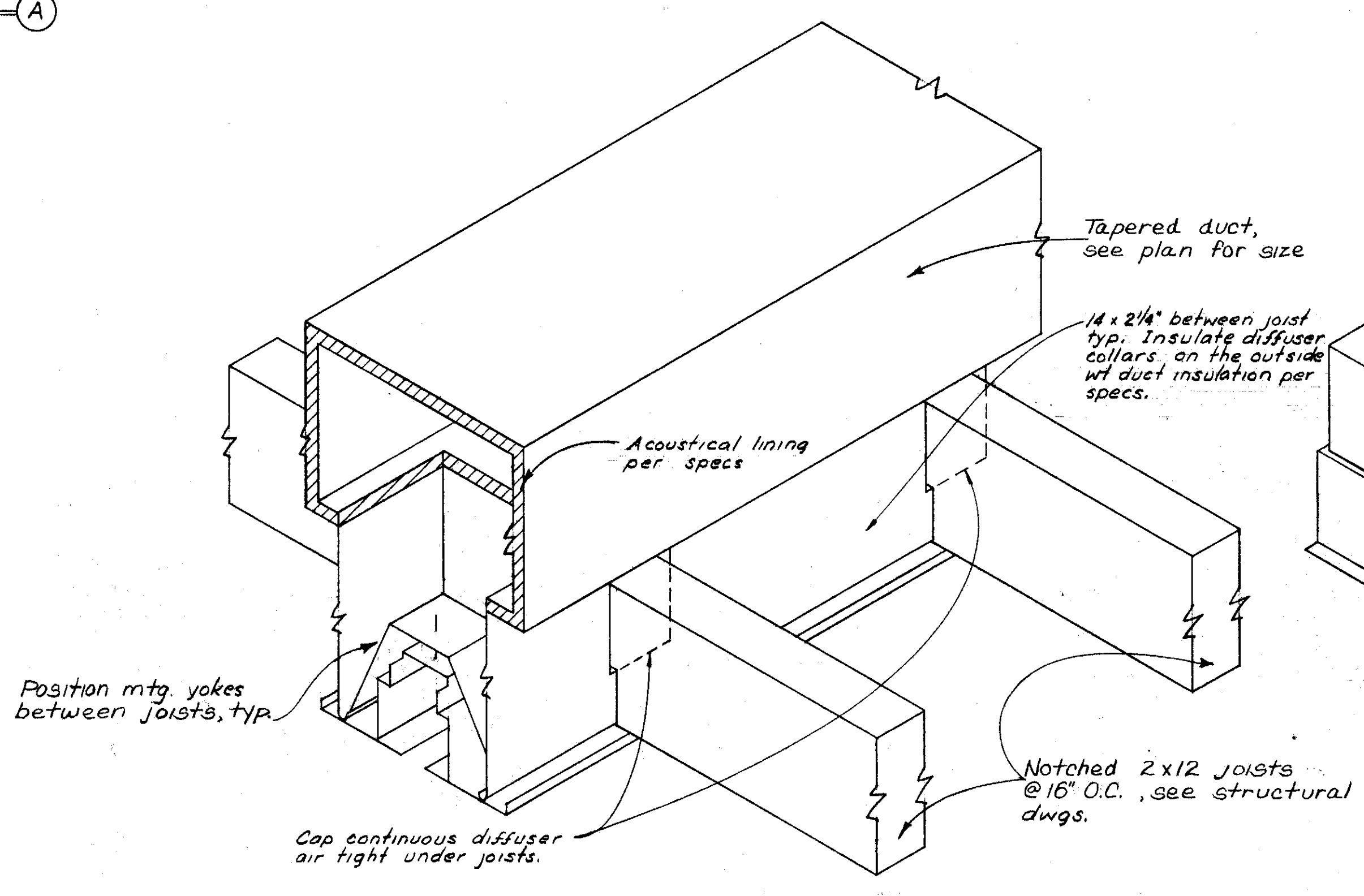
LINEAR DIFFUSER MOUNTING DETAIL No scale
