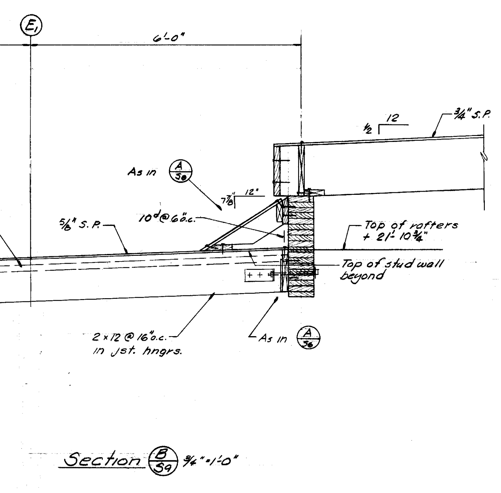
Section D 3/4" = 1'-0"
