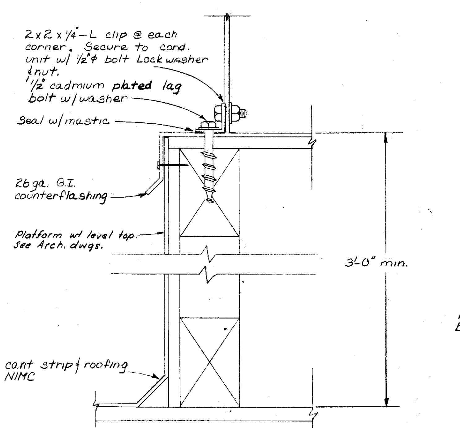
CU-4 MOUNTING DETAIL No scale
