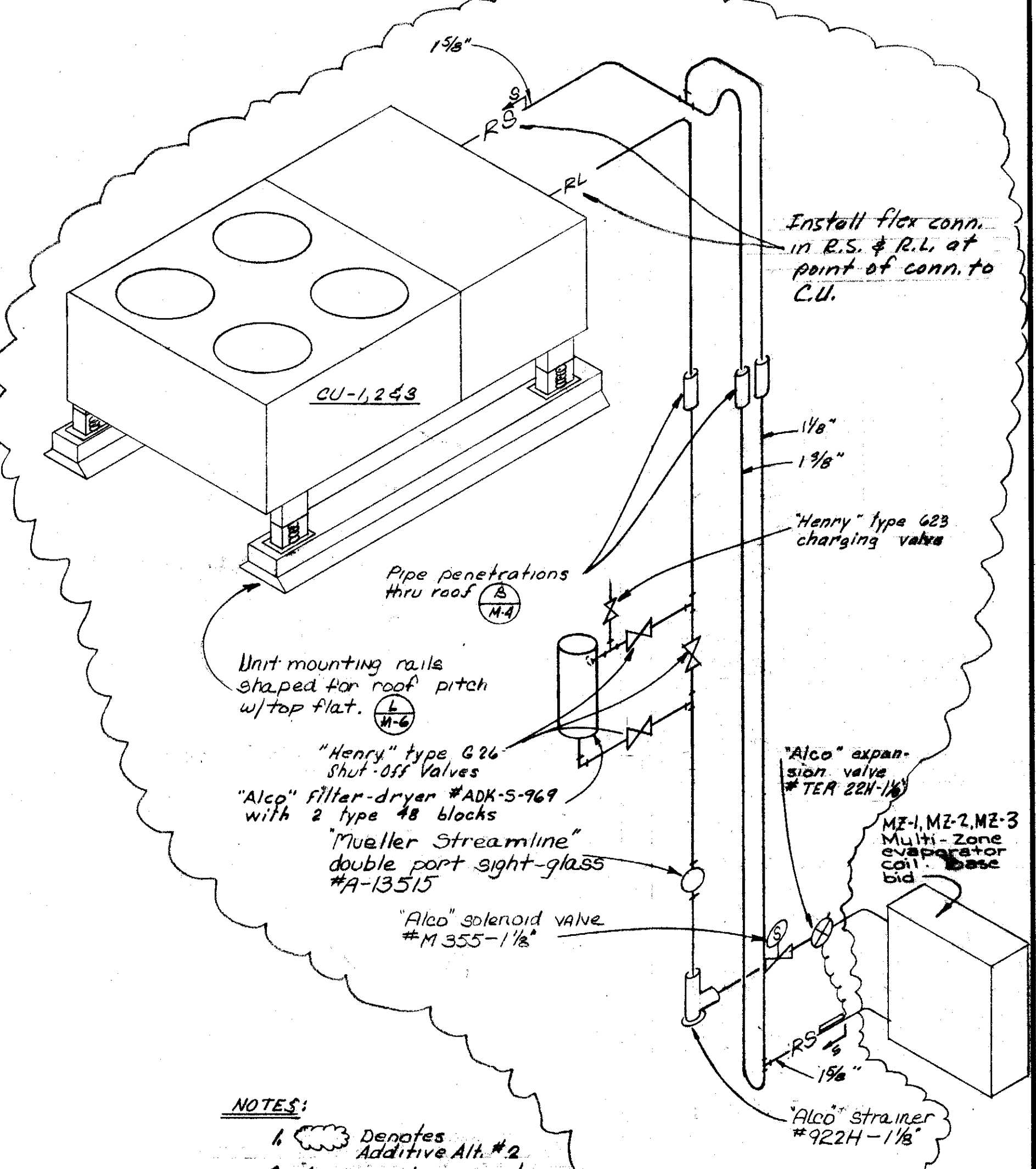
CU-1,2,3 REFRIGERANT PIPING DIAGRAM No scale
