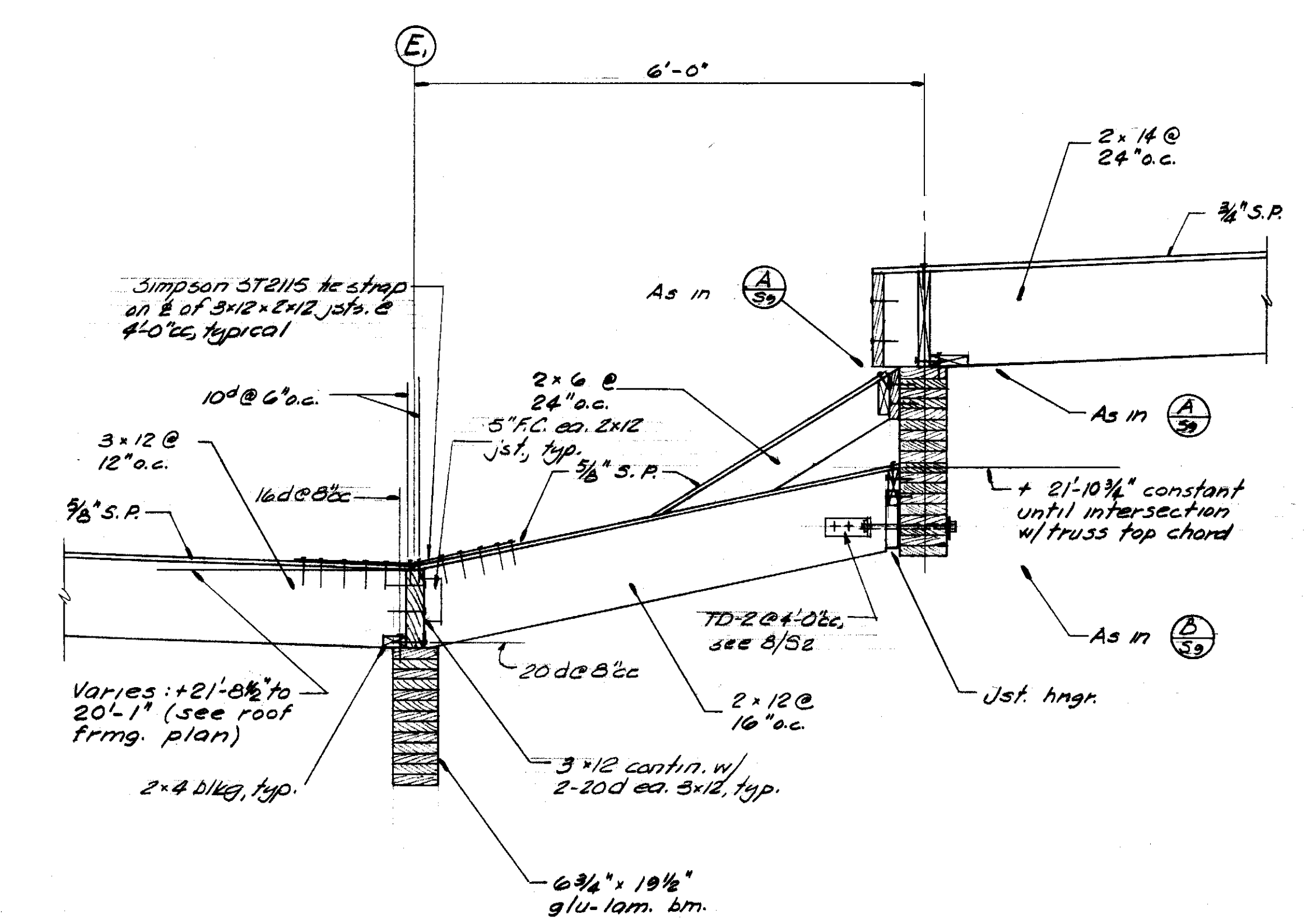
Section E 3/4" = 1'-0"
