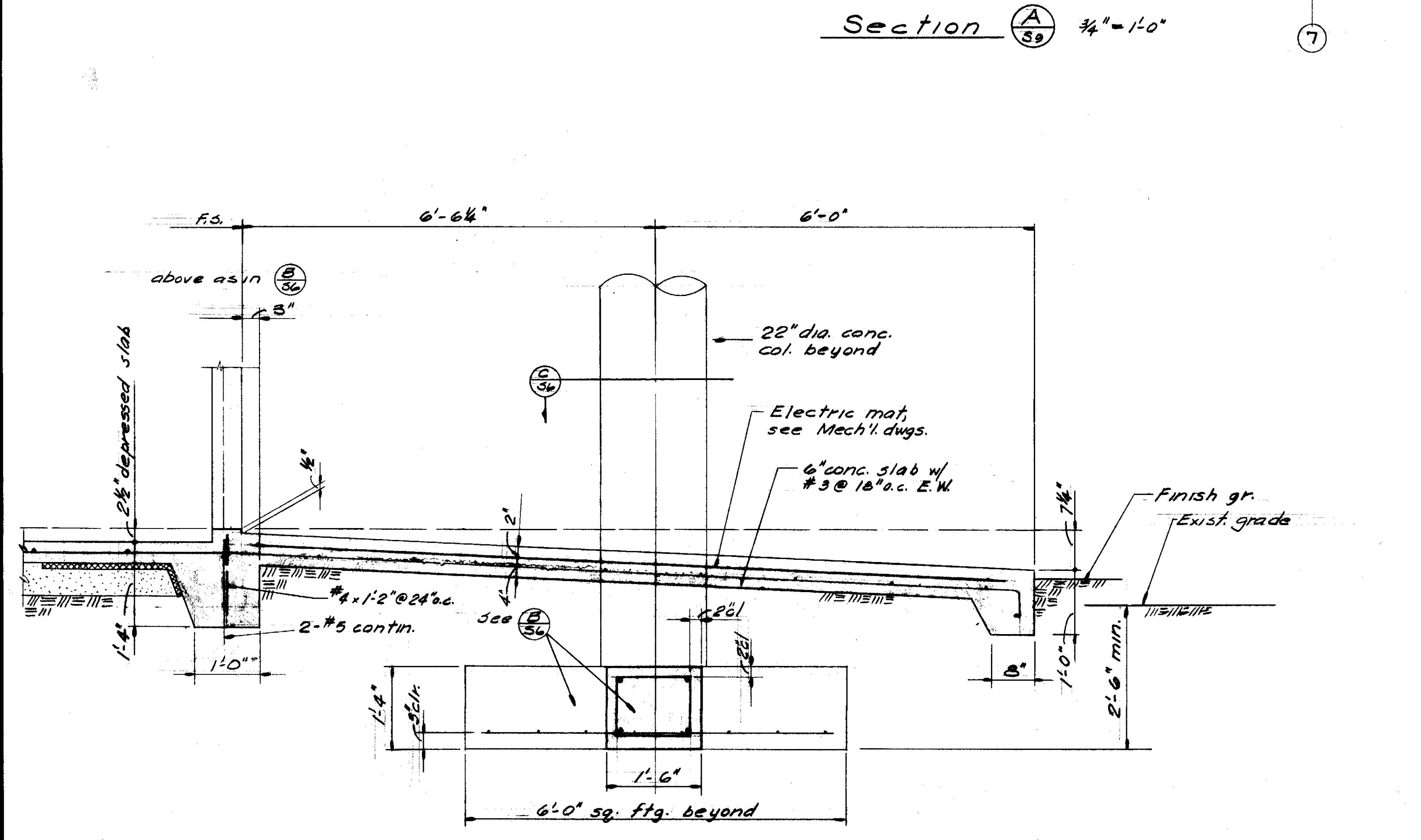
Section C 3/4" = 1'-0"
