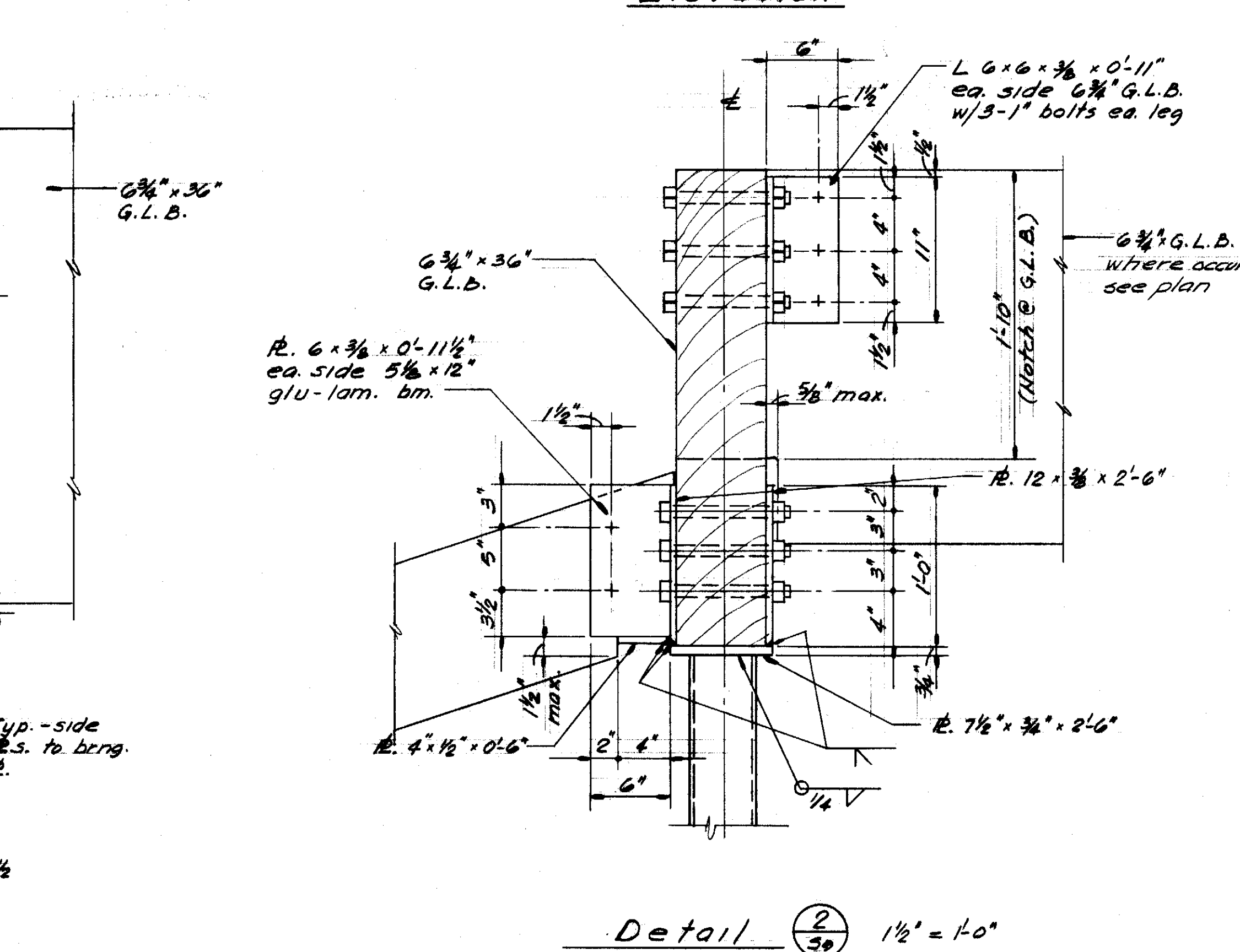
Detail 2 1 1/2" = 1'-0"
