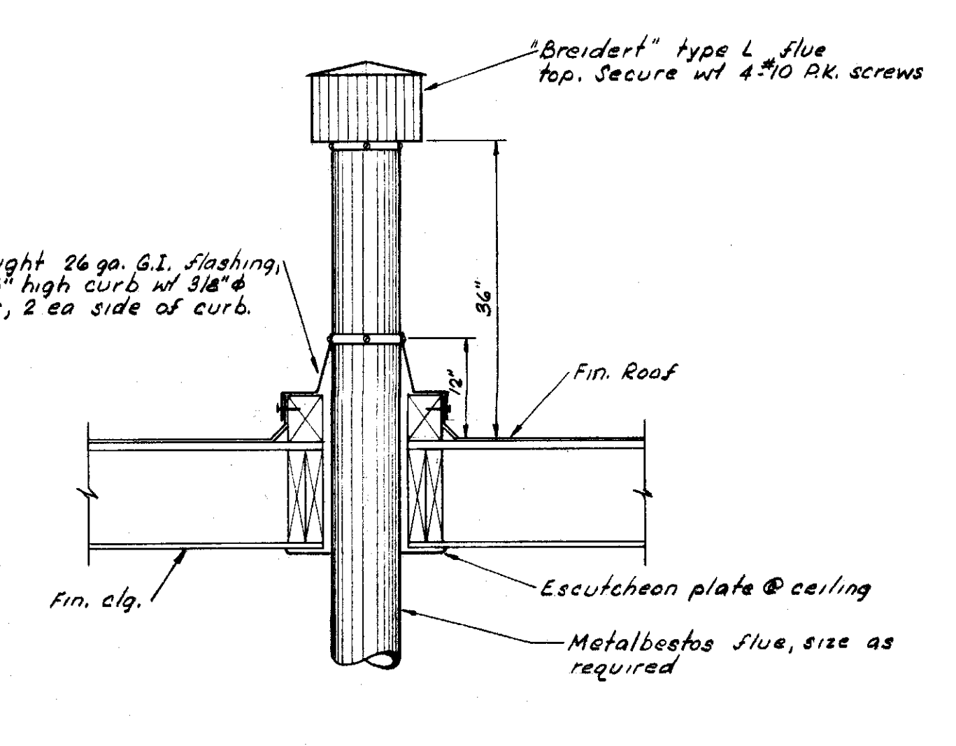
TYPICAL FLUE THRU ROOF DETAIL No SCALE
