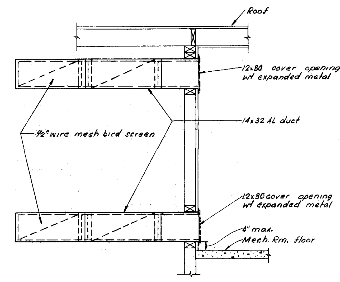
SECTION @ COMBUSTION AIR OPN'GS SCALE = 1/2" = 1'-0"
