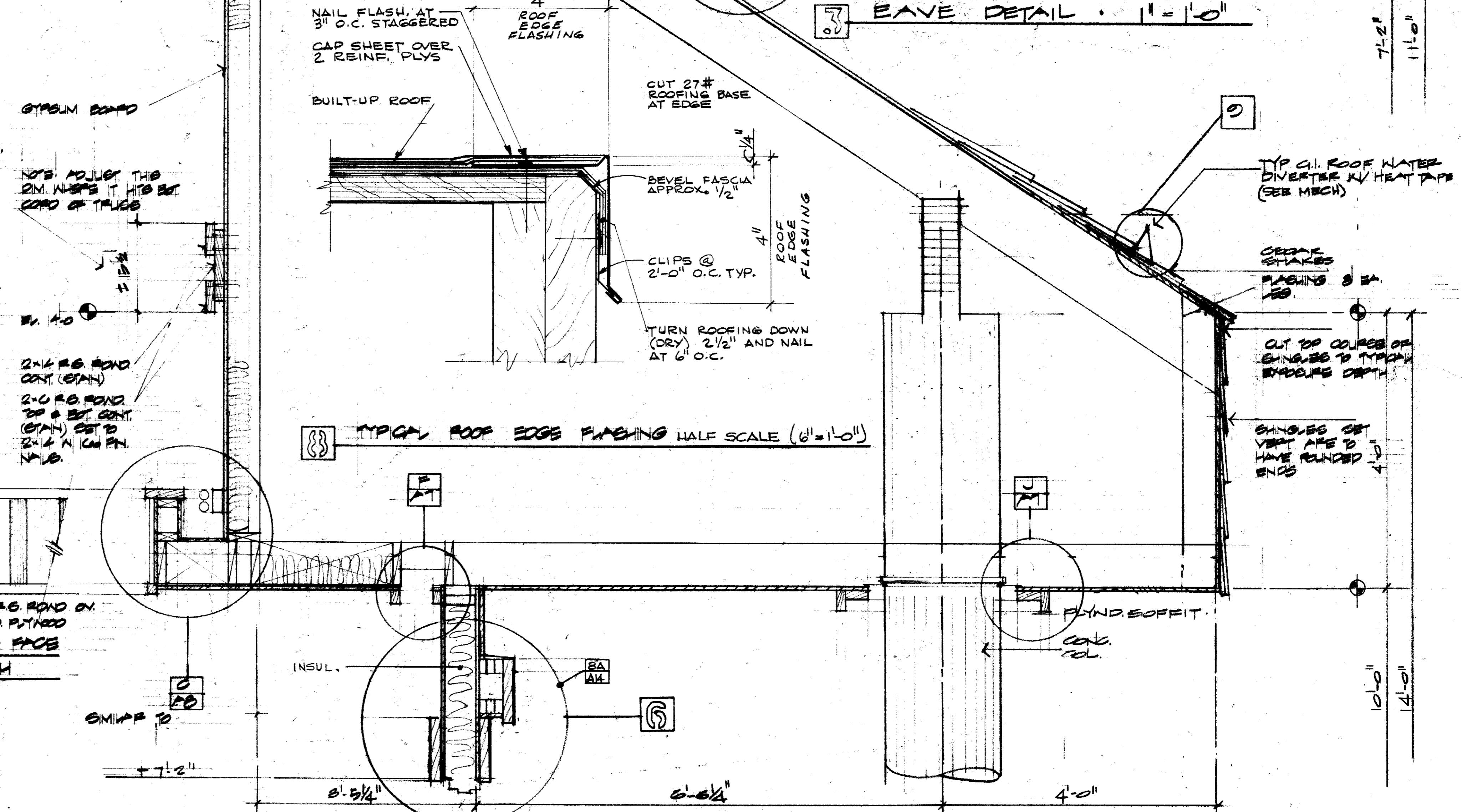
6 ROOF & EAVE DETAIL - 1" = 1'-0"
