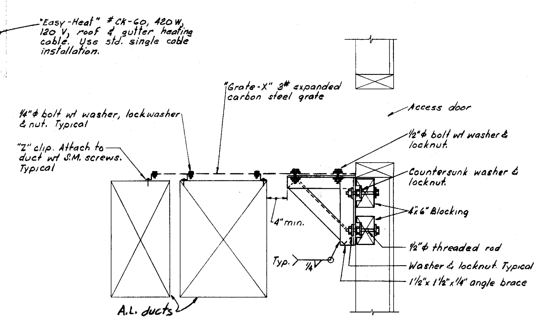
GRATE SUPPORT @ MECH. RM. 202 SCALE = 1/4" = 1'-0"
