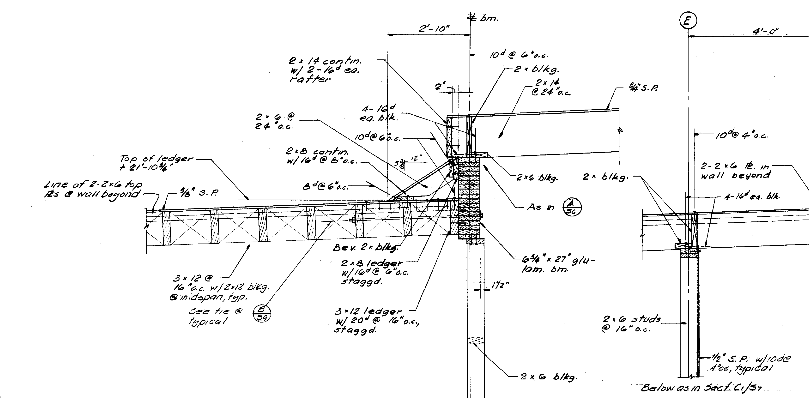
Section A 3/4" = 1'-0"
