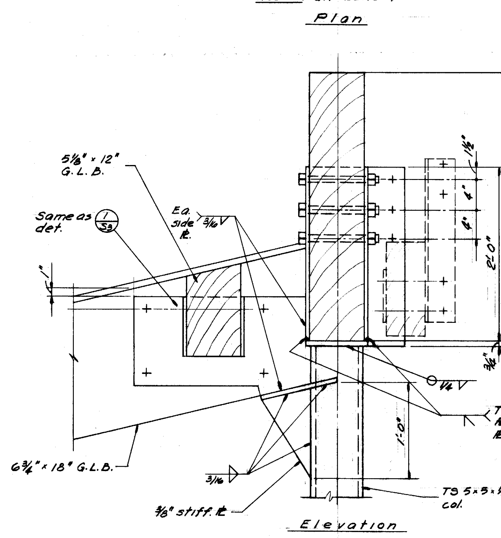
Detail 1 1 1/2" = 1'-0"
