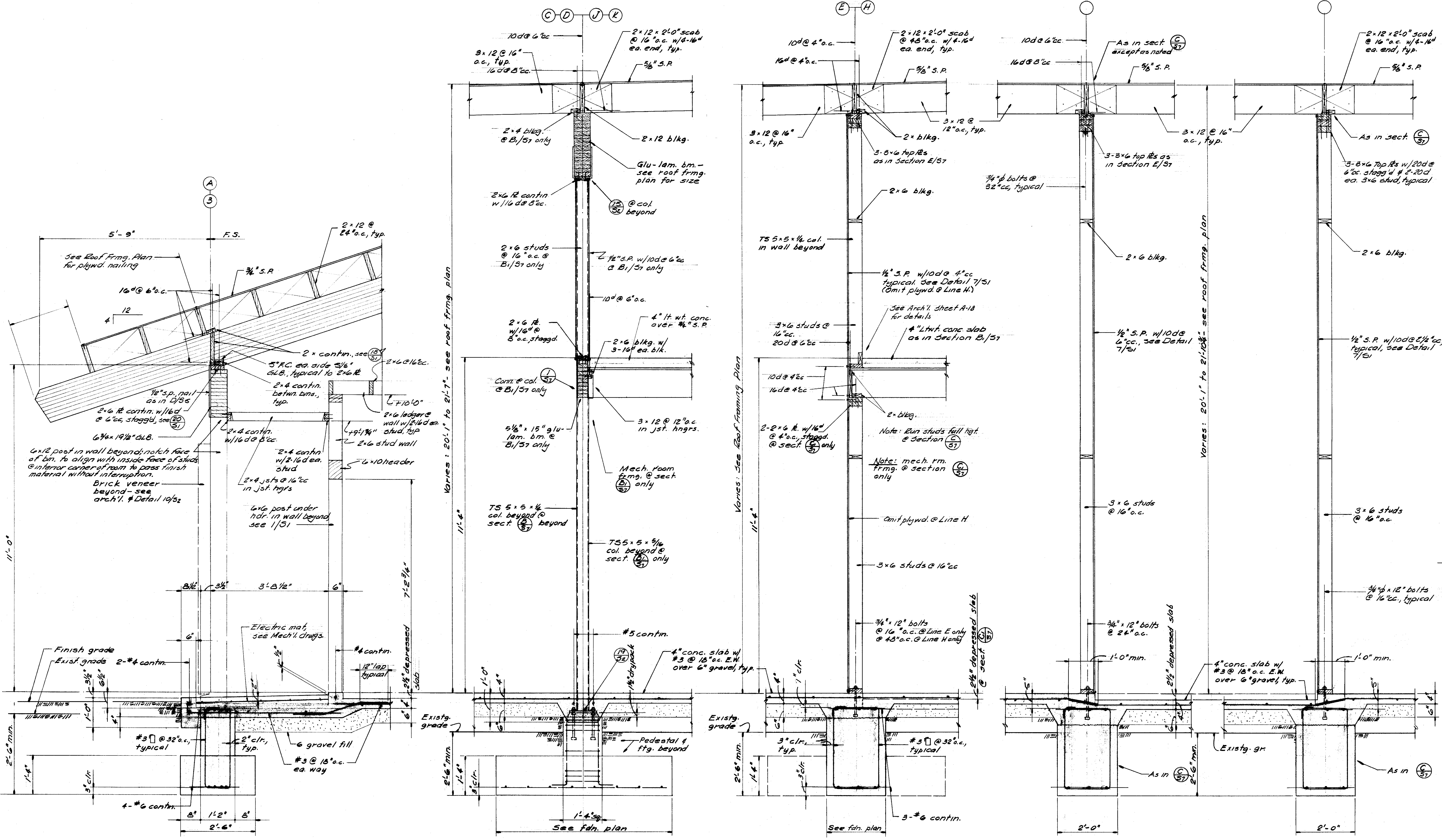
Section A 3/4" = 1'-0"
