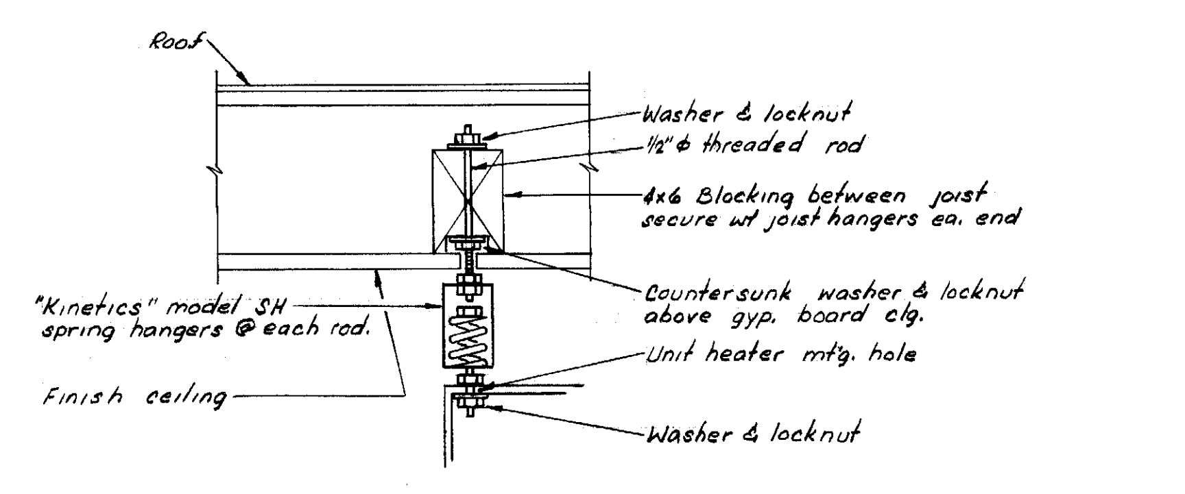
UNIT HEATER MTG. DETAIL No SCALE
