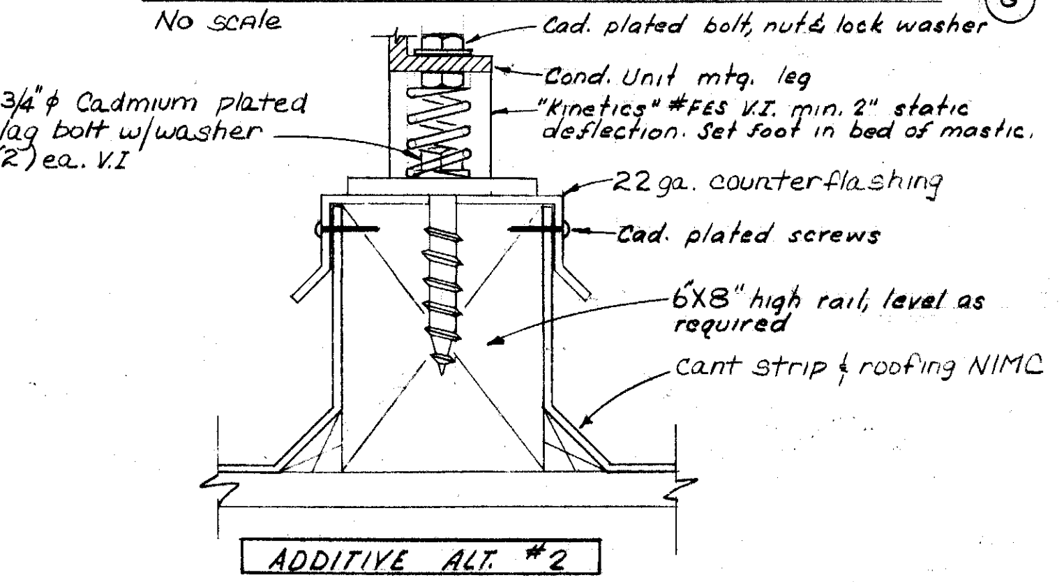
CU-1,2,3 MOUNTING DETAIL No scale
