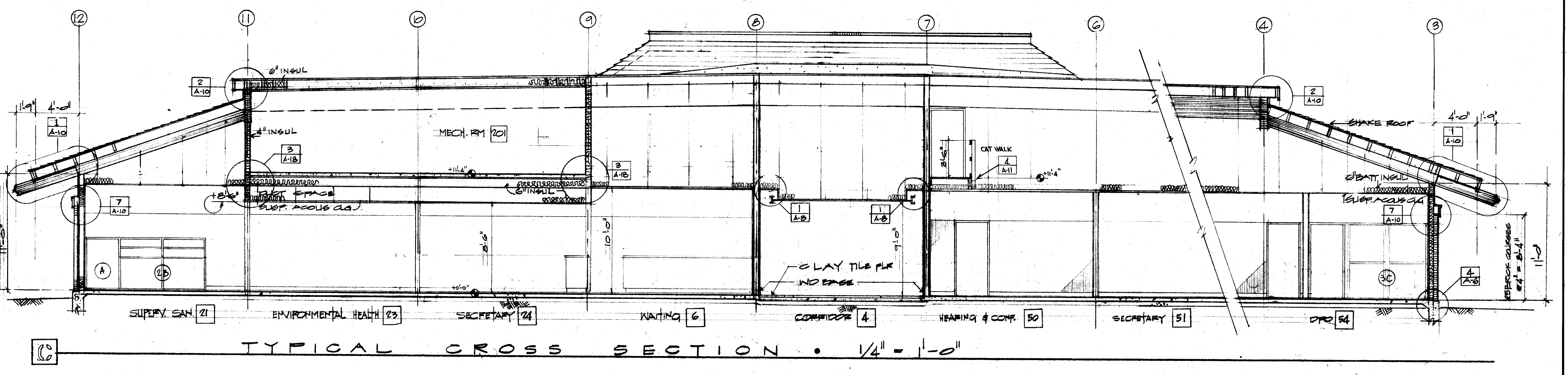
TYPICAL CROSS SECTION • 1/4" = 1'-0"
