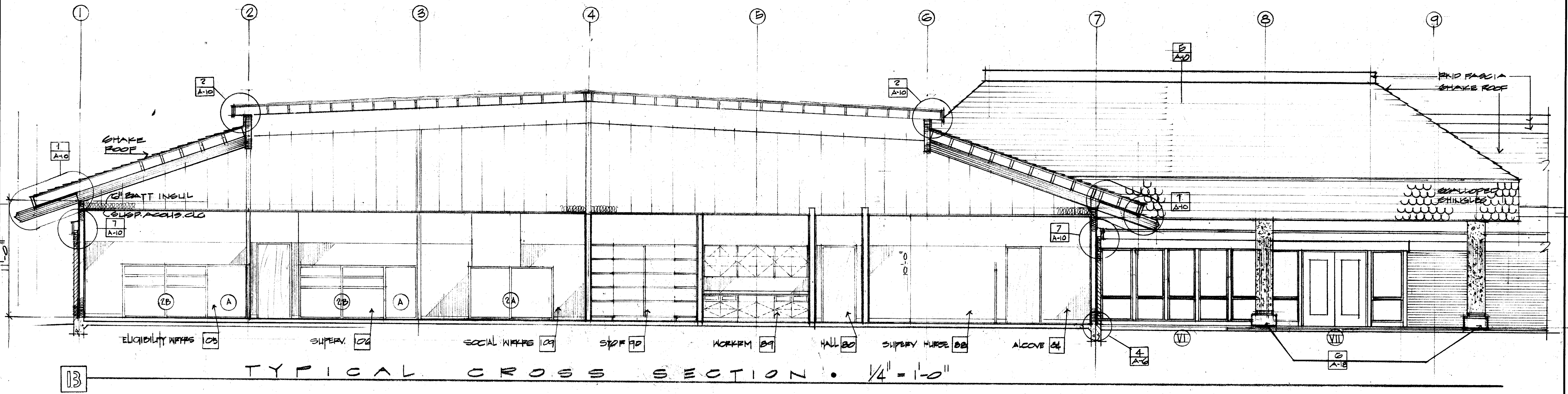
TYPICAL CROSS SECTION • 1/4" = 1'-0"
