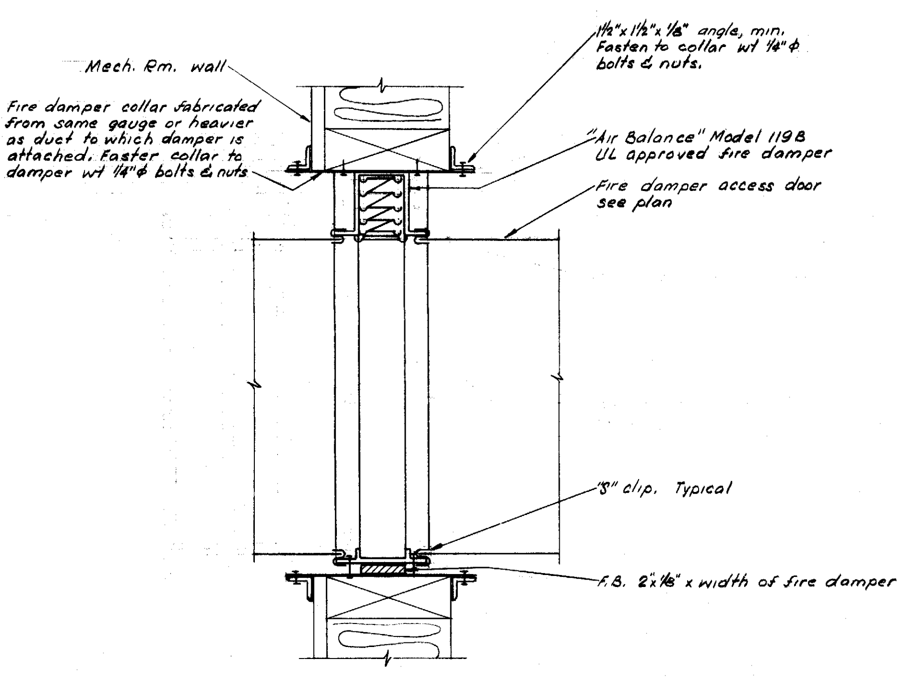
TYPICAL FIRE DAMPER MTG. DETAIL No SCALE
