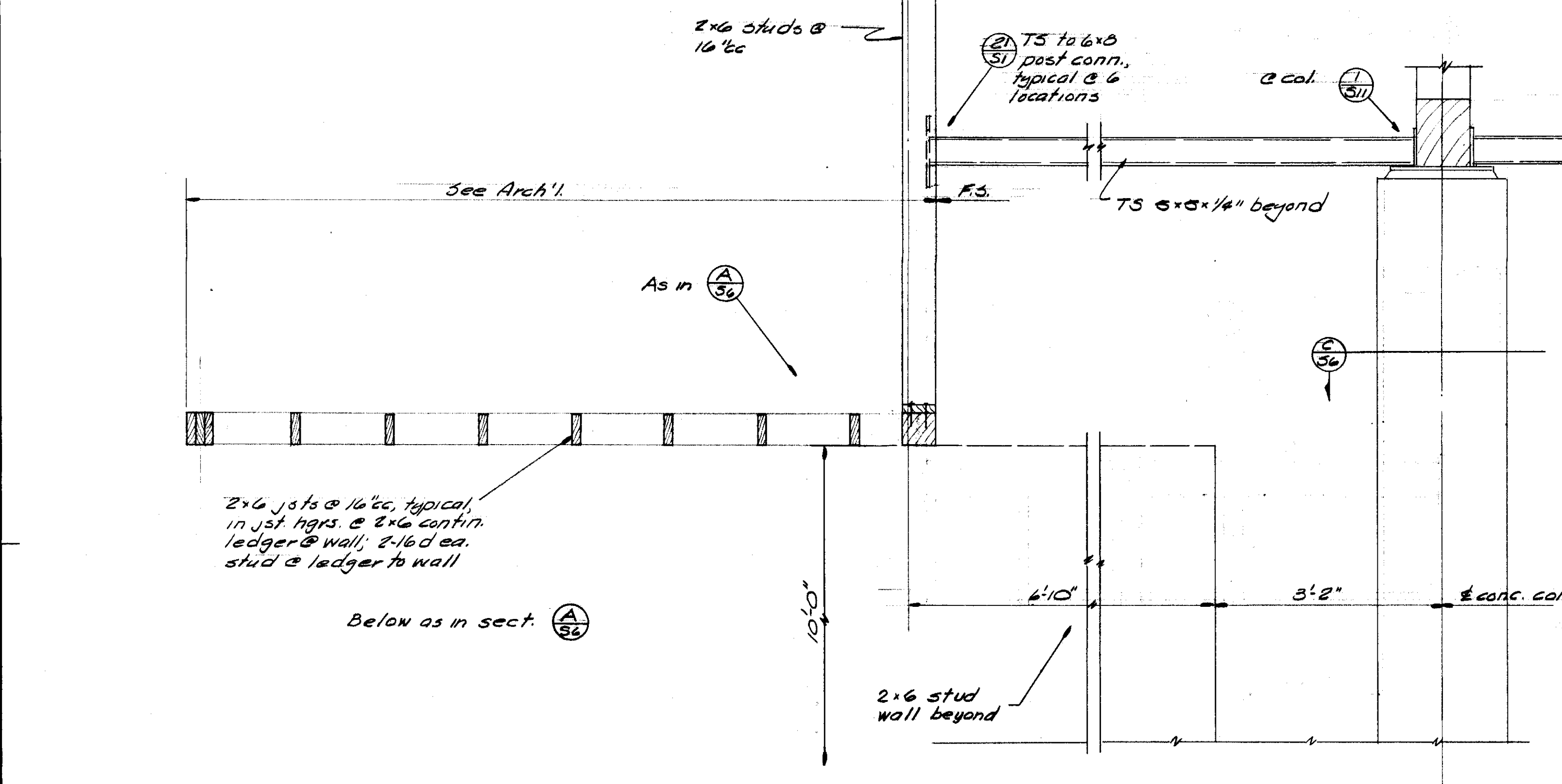
Section B 3/4" = 1'-0"
