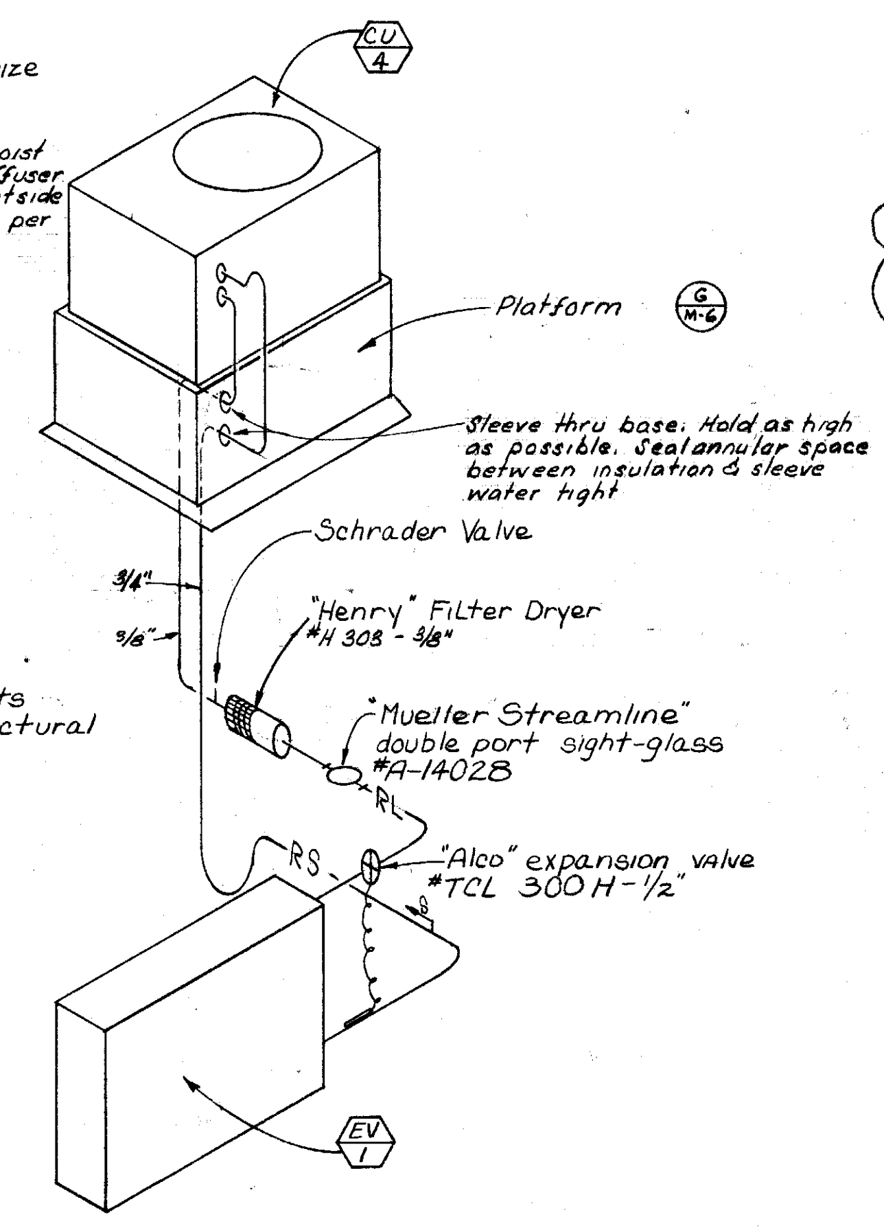
CU-4 REFRIGERANT PIPING DIAGRAM No scale
