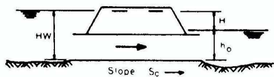
SUBMERGED OUTLET CULVERT FLOWING FULL
