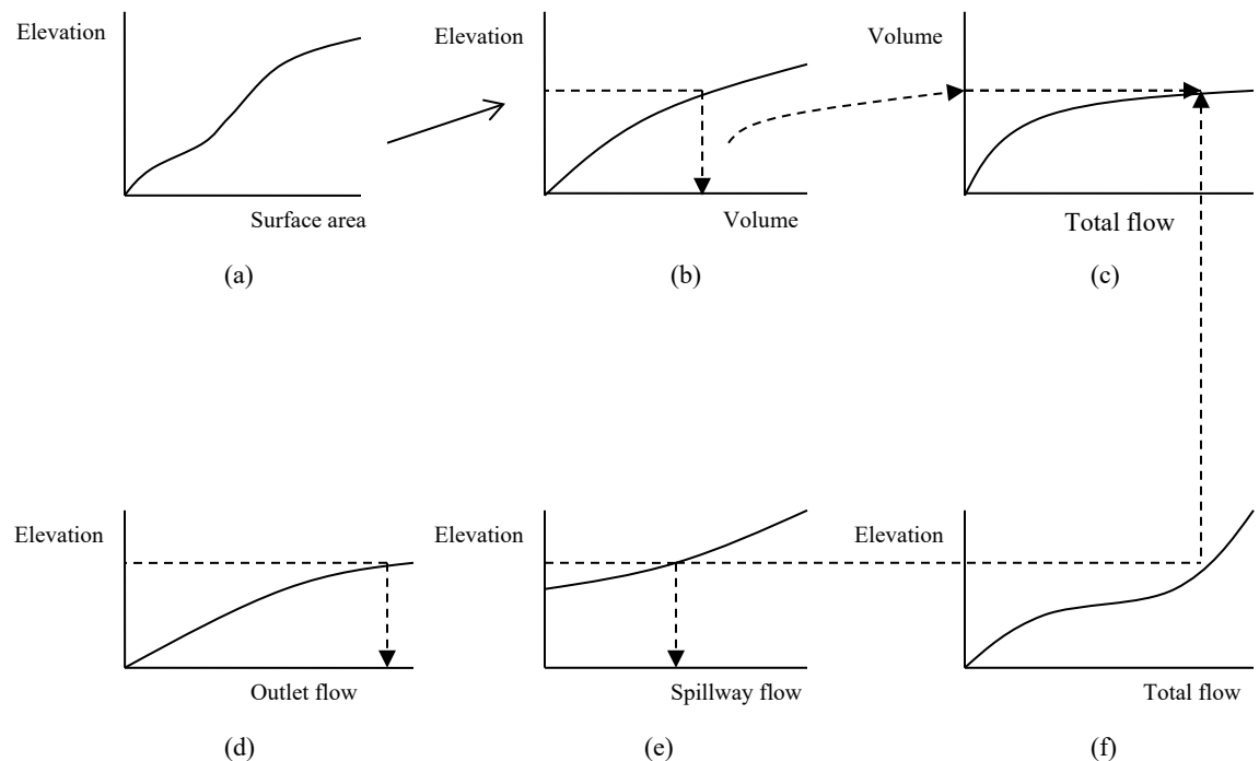
FIG. 5.7.1 Derivation of Storage-outflow Relationship
