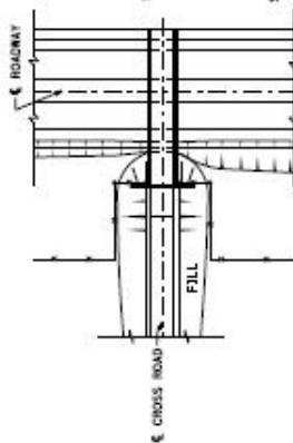
PLAN OF ROADWAY - OVERCROSSING
