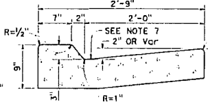
TYPE B4 CURBS
