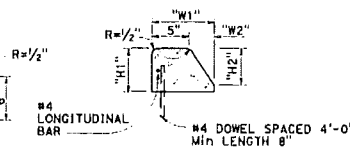
TYPE B3 CURBS Superimposed on existing pavement See Table A
