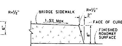
TYPE H CURB On Bridges
