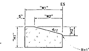
TYPE D CURBS See Table A
