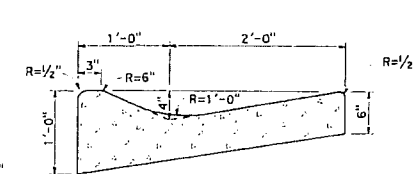
TYPE E CURB
