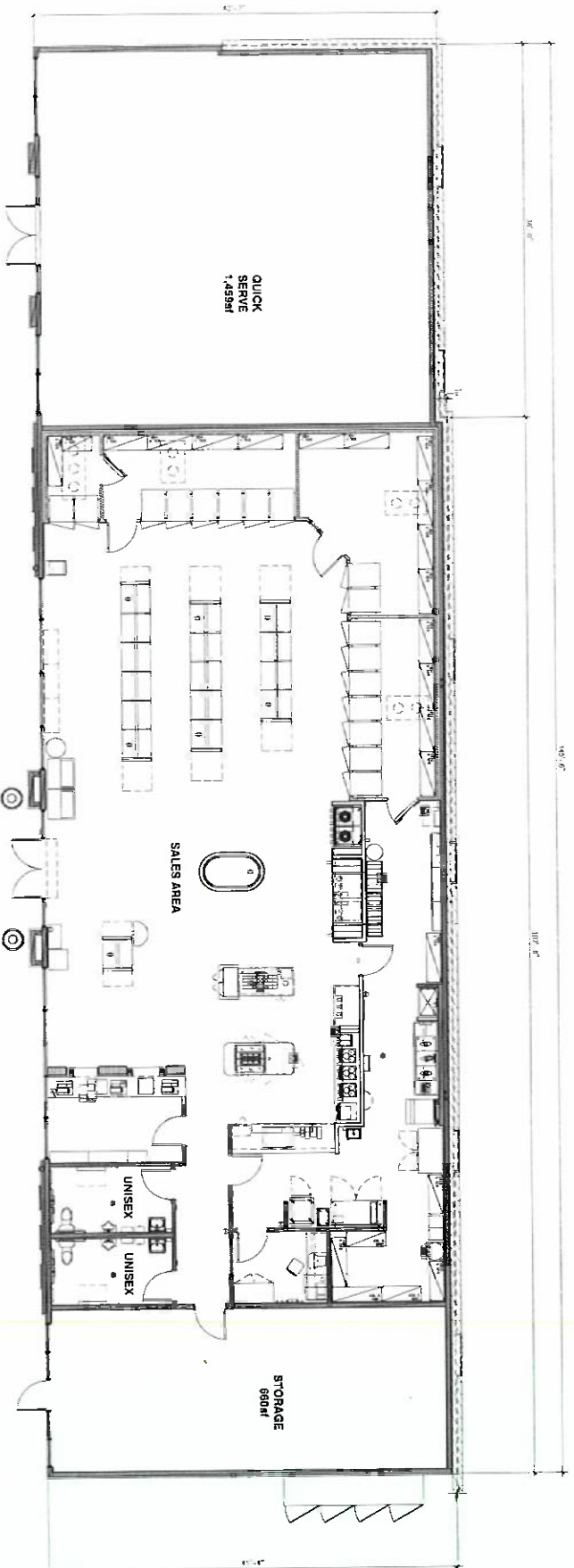
EQUIPMENT FLOOR PLAN
